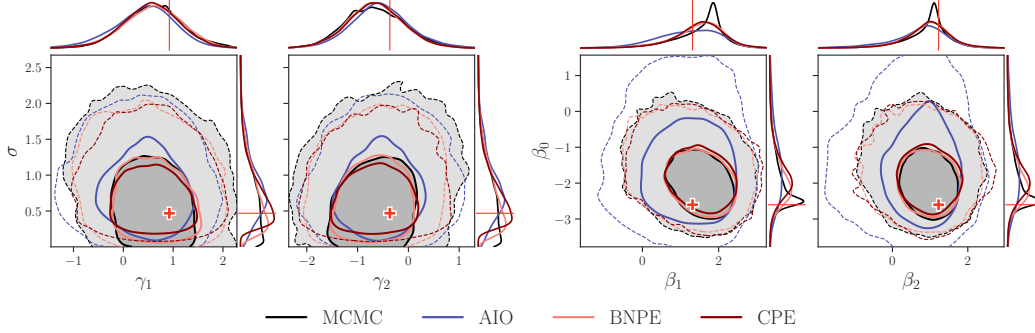
Figure 7: Posterior approximations of the compared methods for the hierarchical model (Section 5.3). Contours enclose 68% and 95% of the posterior mass.
