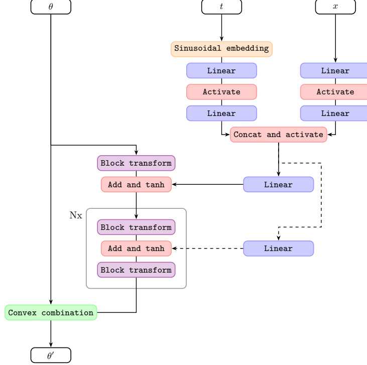
Figure 8: Continuous-time CPE architecture. The data x and the time t are embedded using an MLP and a sinusoidal embedding followed by an MLP, respectively, and concatenated to form the conditioning vector c . We add a linear projection of c after the first block transform, before applying the activation function (Equation (12)). While it is possible to condition after every block transform (dashed lines), we only do so after the first. Finally, the output is combined with the input through the convex combination in Equation (8).
