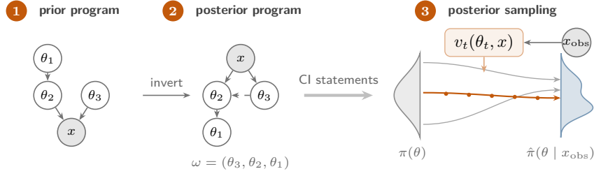
Figure 1: Causal Posterior Estimation: (1) The prior program, i.e., the generative model whose parameters \theta we aim to infer. (2) The prior program is inverted into the posterior program. From the posterior program, conditional dependencies are computed and incorporated into a NN architecture. (3) Posterior inference is conducted by drawing a sample from the prior \pi(\theta) and transporting it to the posterior \pi(\theta|x_{\text{obs}}) by integrating the vector field v_t(\theta^{(t)}, x) .
