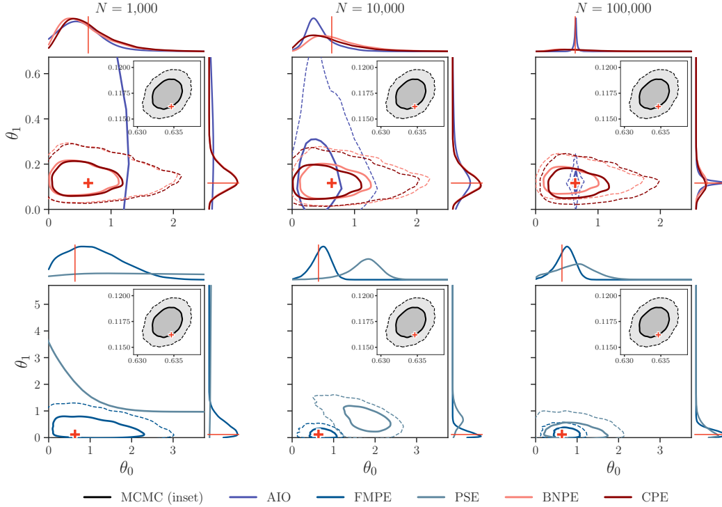
Figure 12: Posterior distributions of all methods for the SIR model, where \theta_0 denotes the contact rate and \theta_1 the recovery rate.
