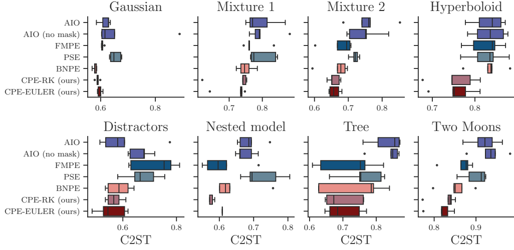
Figure 9: C2ST of CPE and the baselines on the eight benchmark models for a simulation budget of N = 10000 . Values closer to 0.5 are better. CPE-RK and CPE-Euler denote CPE with an adaptive Runge–Kutta 5(4) solver and a 20-step Euler solver, respectively.
