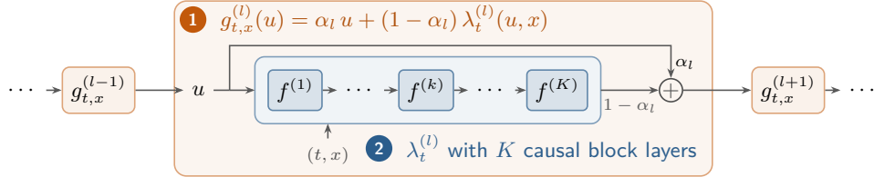
Figure 2: Overview of CPE. The vector field v_t(\theta^{(t)}, x) is a composition of L prior-guided blocks (Section 3.1). Each block forms a trainable convex combination of its input u , with u = \theta^{(t)} for the first block, and a causal block-autoregressive network \lambda_t^{(l)} with K causal block layers (Section 3.2).
