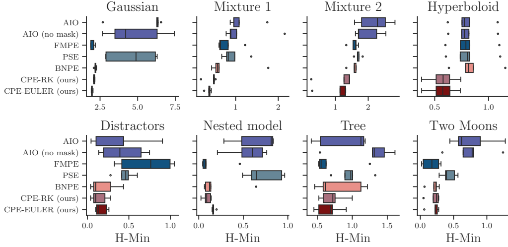
Figure 5: Performance of CPE and all baselines on eight common SBI benchmark models, measured by the H-min metric (lower is better).
