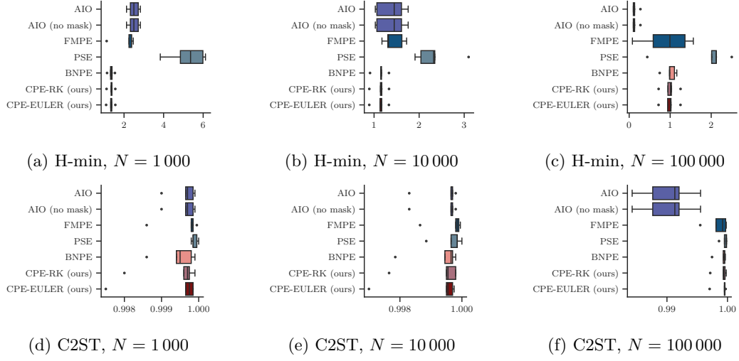
Figure 11: H-min (top row) and C2ST (bottom row) of all methods on the SIR model for simulation budgets N \in \{1000, 10000, 100000\} . Lower H-min values and C2ST values closer to 0.5 are better.
