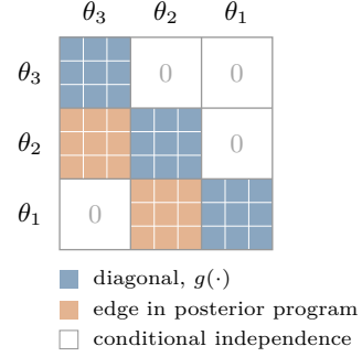
Figure 4: Masked weight matrix B^{(k)} for the posterior program in Figure 3b.
