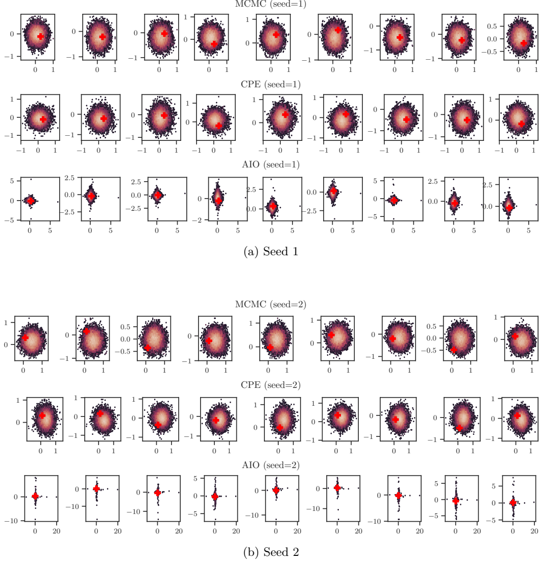
Figure 10: Posterior distributions of CPE and AIO for the linear Gaussian model. The AIO posterior is degenerate for all five seeds (only two out of five seeds shown), although it achieves low C2ST values (Figure 9).
