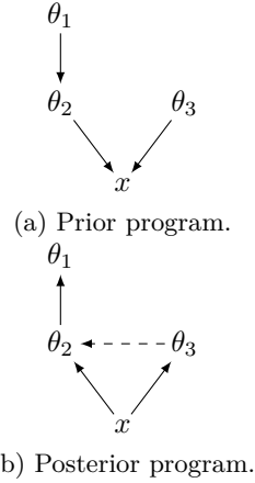
Figure 3: Graphical models illustrating prior and posterior dependencies.
