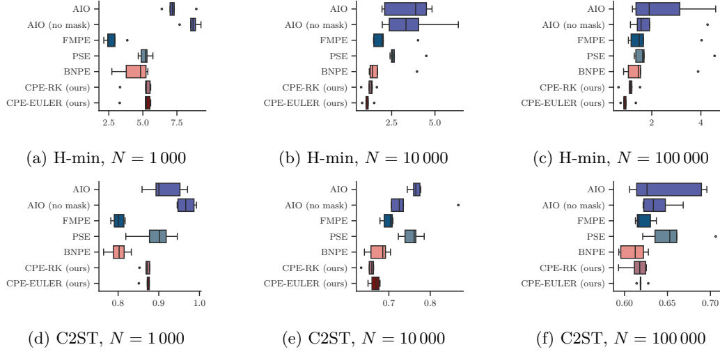
Figure 14: H-min (top row) and C2ST (bottom row) of all methods on the hierarchical model for simulation budgets N \in \{1000, 10000, 100000\} . Lower H-min values and C2ST values closer to 0.5 are better.
