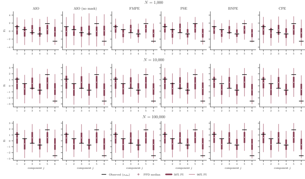
Figure 16: Posterior predictive distributions of all methods for the hierarchical model.
