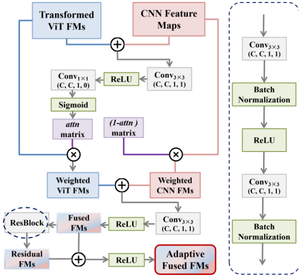
Fig. 6: Architecture of the Adaptive Global-Local Feature Fusion Module. (FMs: feature maps; (C, C, 1, 1) denotes convolution parameters—input channels, output channels, kernel size, and padding. Circular padding is applied to the left and right boundaries of the feature maps.)
