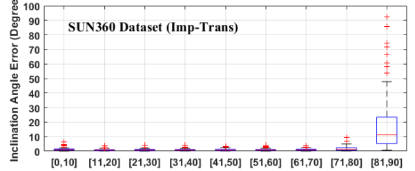
(b) implicit data-driven feature transformation strategy
