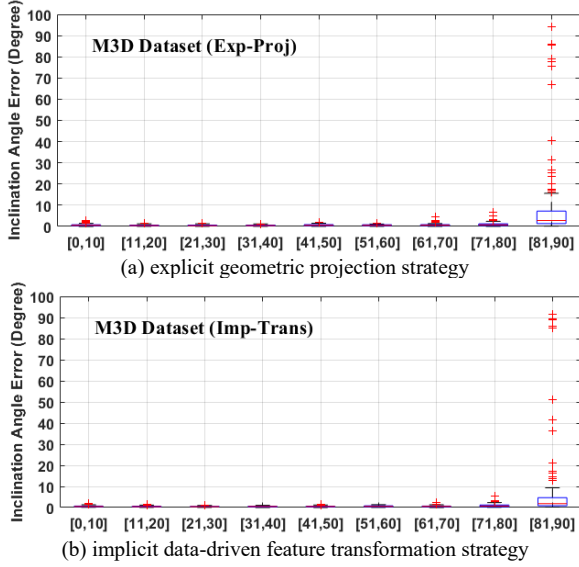
Fig. 8. Box plots of angle error distributions across different camera inclination ranges (in degrees) on the M3D dataset.
