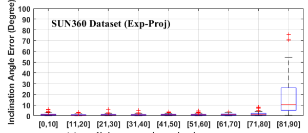
(a) explicit geometric projection strategy
