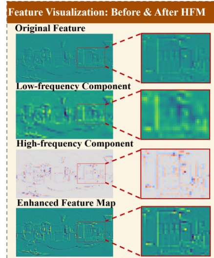
Fig. 5. Visualization of feature responses before and after HFM. The original, low-frequency, high-frequency, and enhanced features are shown using the same feature channel, with the same region enlarged for comparison.
