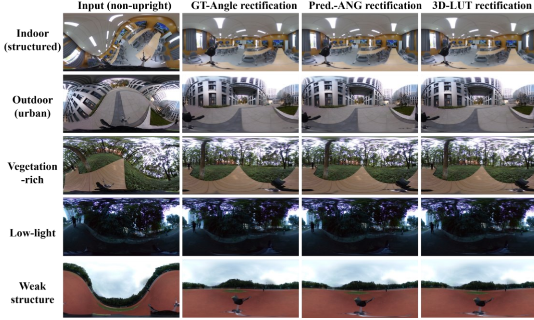
Fig. 10. Representative qualitative rectification results on real-world RICOH THETA panoramas. From left to right: non-upright input, geometric rectification using the ground-truth orientation, geometric rectification using the predicted orientation, and learned 3D spherical-LUT rectification. The examples include indoor, outdoor, vegetation-rich, low-light, and open-scene conditions.
