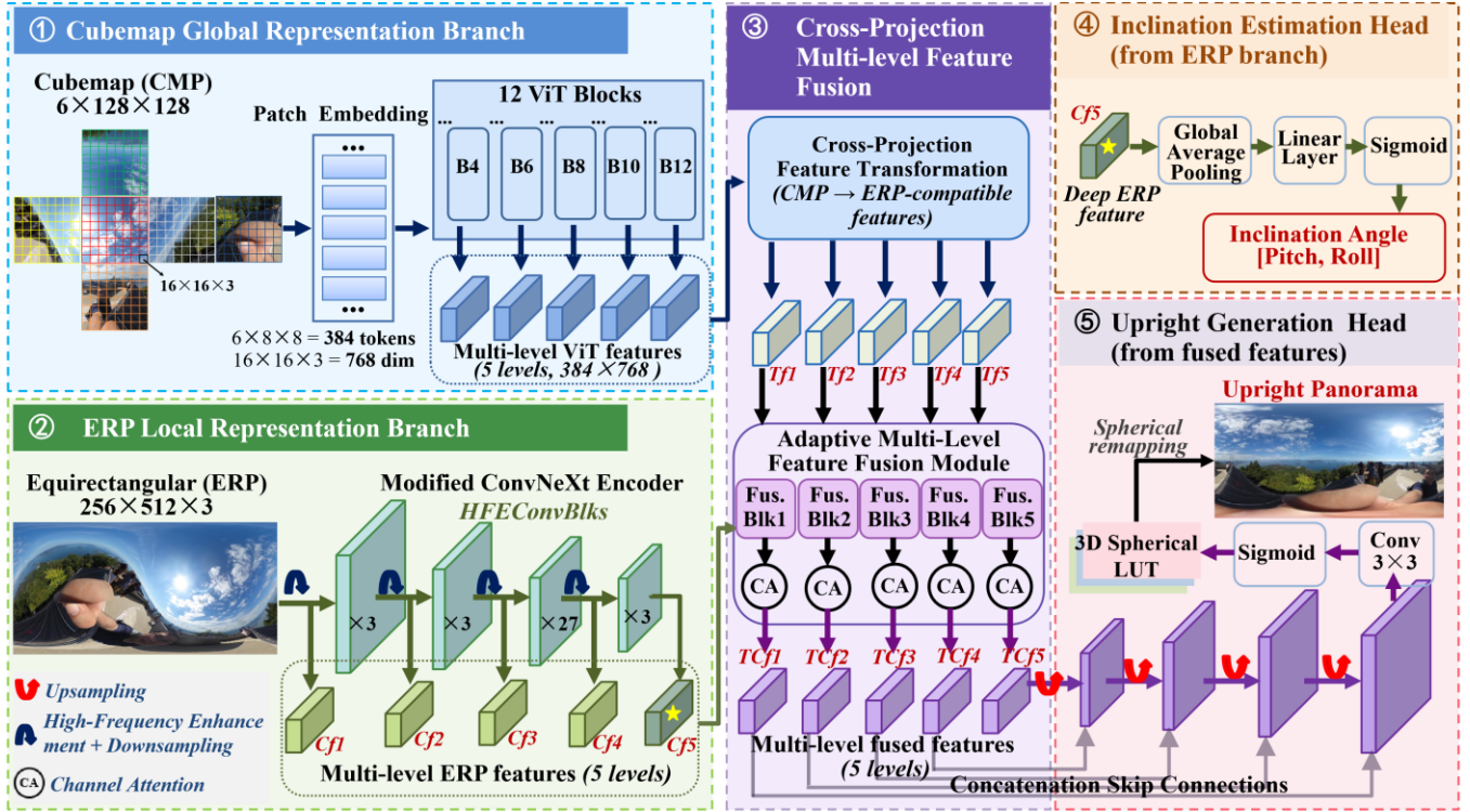
Fig. 2: Overview of the proposed projection-aware dual-projection framework for 360-degree image rectification. The cubemap and ERP branches extract complementary global and local representations, which are integrated through five-level cross-projection fusion. The deepest ERP feature is used for inclination angle estimation, while the fused features are decoded to predict a 3D spherical LUT for upright panorama generation.
