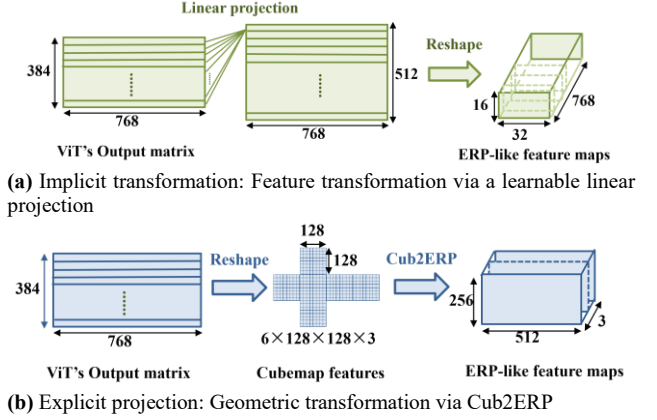
Fig.3: Cross-projection feature transformation strategies for feature fusion.
