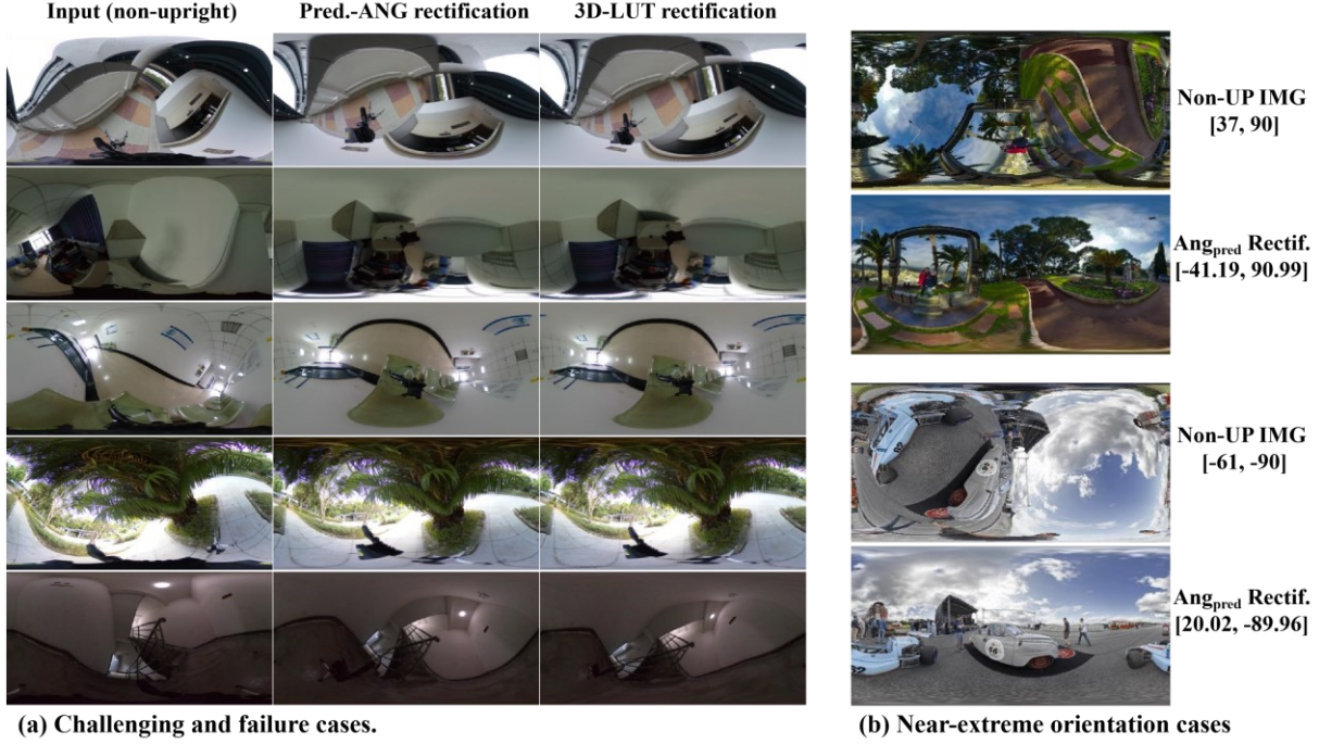
Fig. 11. Representative challenging and failure cases from the controlled benchmarks and the real-world THETA set. (a) Real-world challenging and failure cases under combinations of adverse factors, including large inclination, close-range scene geometry, misleading local structures, repetitive textures, and low illumination. (b) Near-extreme orientation cases in which large pitch-roll discrepancies can still result in visually similar upright rectification.
