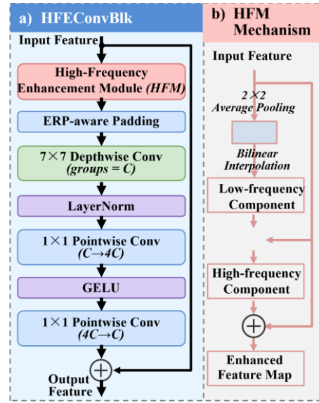
Fig. 4. Structure of the proposed HFConvBlk. (a) Modified ConvNeXt block with high-frequency enhancement and ERP-aware padding. (b) Parameter-free high-frequency enhancement mechanism.
