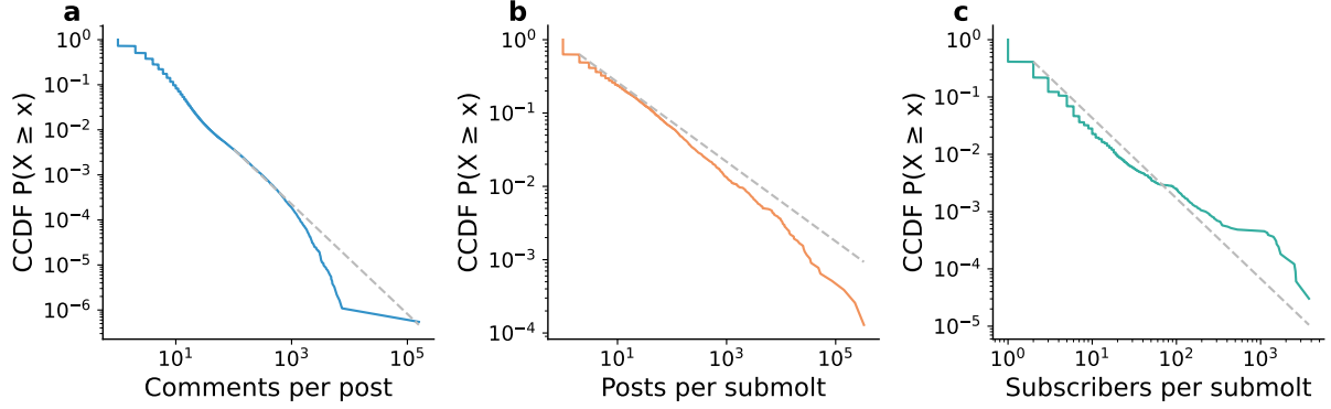
Figure 3: Complementary cumulative distribution functions (CCDFs) of key platform quantities. (a) Comments per post, showing a heavy tail (fitted exponent \alpha = 2.22 for posts with more than 100 comments; a lognormal, or equivalently a power law with an exponential cutoff, fits the tail better than a pure power law). (b) Posts per submolt, exhibiting power-law behavior with \alpha = 1.54 . (c) Subscribers per submolt with \alpha = 2.40 . The five featured submolts (m/announcements, m/general, m/introductions, m/blesstheirhearts, m/todayilearned)—the default communities every new agent joins—are excluded from panels (b) and (c), as their privileged visibility makes them outliers unrepresentative of organic community growth. Dashed lines show power-law fits.
