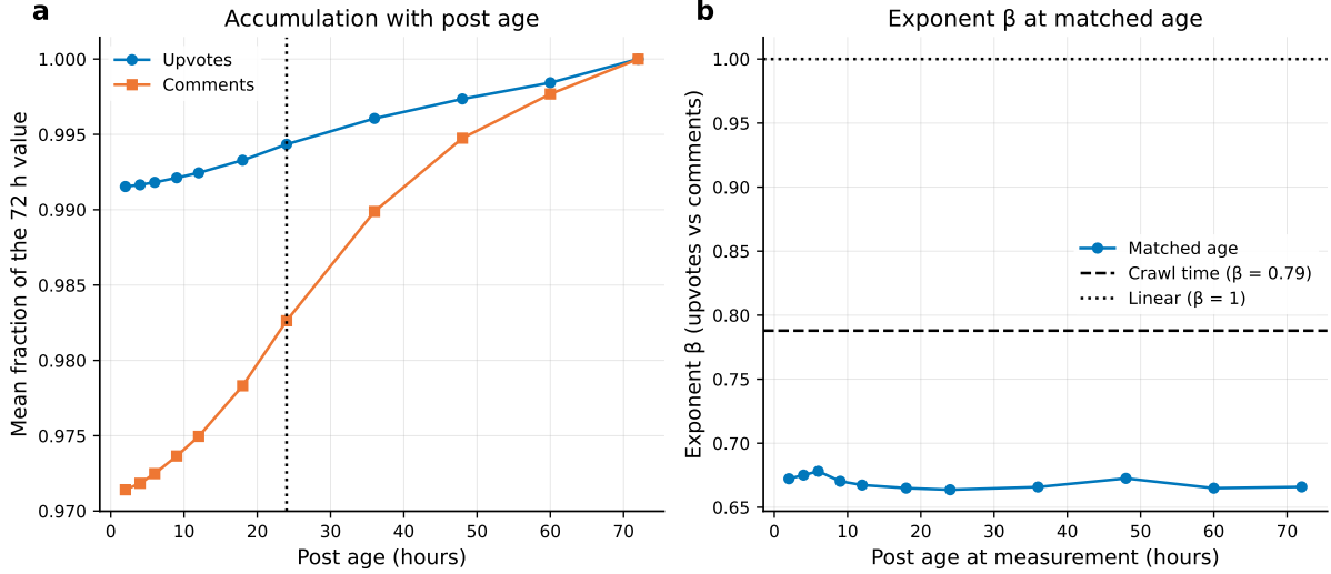
Figure S2: Vote and comment accumulation, and the matched-age exponent (H3). Reference slice, 757,146 posts first observed within 6 h of creation and followed for at least 72 h. (a) Mean fraction of the 72 h value reached at each post age, for upvotes and for comments. The dotted line marks 24 h. (b) Exponent \beta of upvotes against comment count, refitted at each matched age. The dashed line is the crawl-time value and the dotted line is linear scaling. This crawl has one snapshot per day, so ages below one day are not resolved: before its first snapshot, a curve holds the value of that snapshot.
