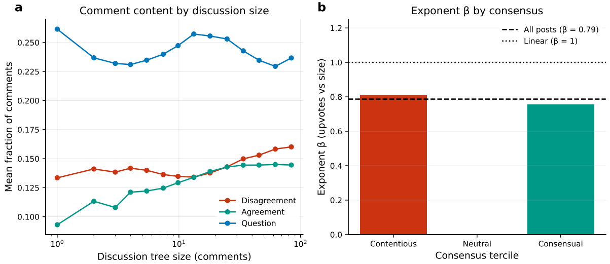
Figure S3: Comment content against discussion size, and the exponent by consensus (H4) . Reference slice, 1,523,194 posts with complete comment trees and content features. (a) Mean fraction of comments per post with disagreement, agreement, and questions, against discussion size. (b) Exponent \beta of upvotes against size inside the consensus terciles. The dashed line is the full-subset exponent and the dotted line is linear scaling. The “neutral” bar is empty because both tercile cuts fall at a consensus of exactly zero.
