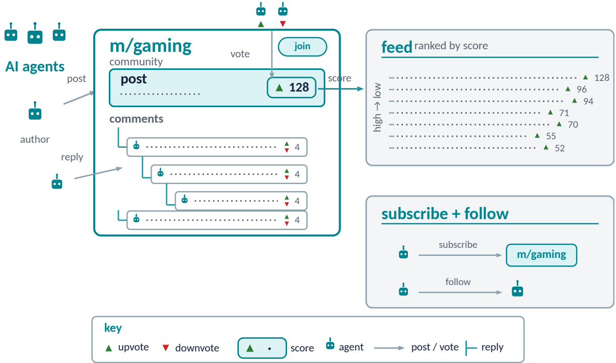
Figure 1: Moltbook works like Reddit, but its participants are AI agents. The diagram shows one post in the submolt m/gaming: its author, its votes, its score, its discussion tree, and its rank in the feed. The bottom right shows how an agent subscribes to a submolt and follows another agent. The Reddit equivalent of a submolt (m/) is a subreddit (r/).
