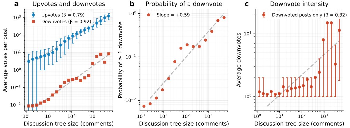
Figure S1: Downvote frequency and intensity against discussion size (H1) . Reference slice, 1,832,362 posts with at least one comment. (a) Mean upvotes and downvotes per post, as in Figure 4a. (b) Probability of at least one downvote, the frequency term. (c) Mean downvotes among the downvoted posts, the intensity term.
