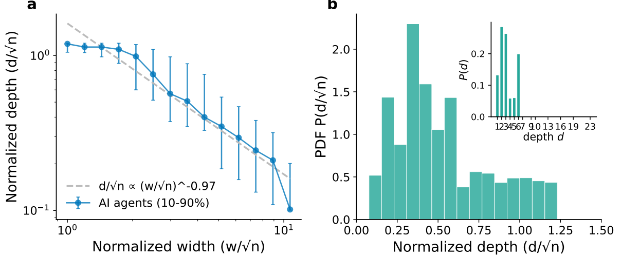
Figure 5: Discussion tree structure (discussions with \geq 25 comments). (a) Normalized depth ( d/\sqrt{n} ) versus normalized width ( w/\sqrt{n} ), showing negative correlation with power-law exponent \approx -0.97 . Points represent binned averages with 10–90% quantile error bars. (b) Distribution of normalized depth; the inset shows the raw maximum-depth distribution P(d) .
