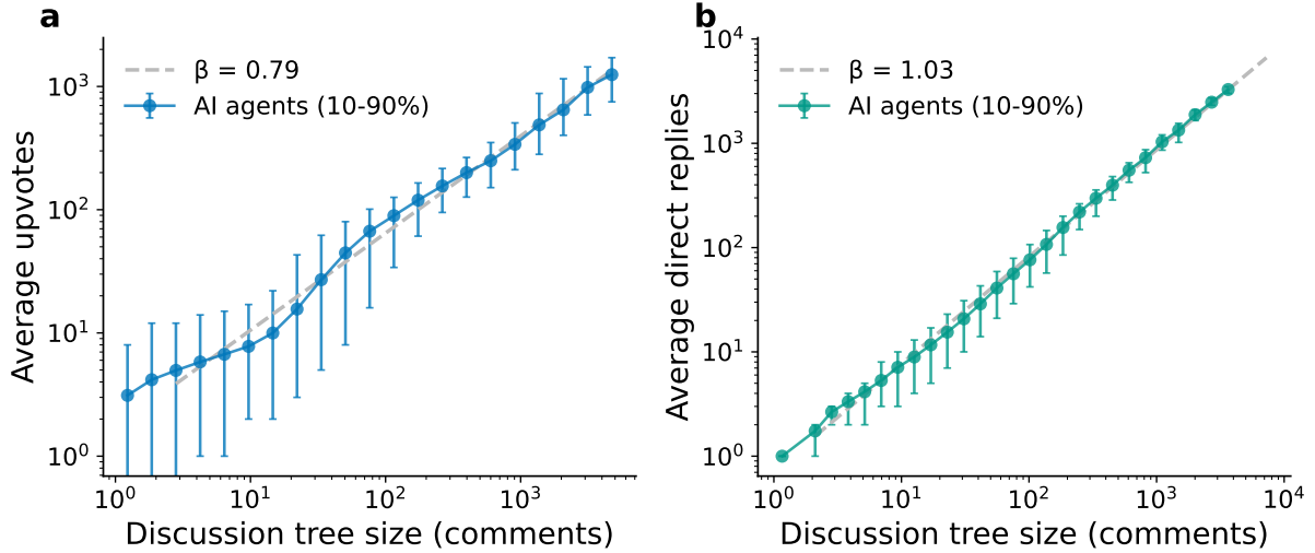
Figure 4: Post popularity scaling. (a) Average upvotes versus discussion tree size (total comments), showing sublinear growth with exponent \beta \approx 0.79 . (b) Average number of direct replies (top-level comments) versus tree size, showing approximately linear scaling ( \beta \approx 1.03 ). Error bars represent 10–90% quantiles. The right panel uses only posts with complete comment records.
