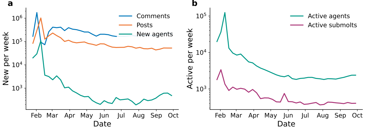
Figure 2: Platform growth over time. Spam-flooded posts are excluded throughout (see Methods). (a) Weekly counts of new posts, comments, and agents (first activity): after an explosive first few weeks, activity settles onto a slowly declining plateau and the influx of new agents collapses by more than two orders of magnitude. (b) Weekly counts of active agents (those posting or commenting that week) and active submolts (those receiving posts). The active population peaks near 124,000 agents and 3,400 submolts during the launch, then declines by over an order of magnitude as the platform matures.
