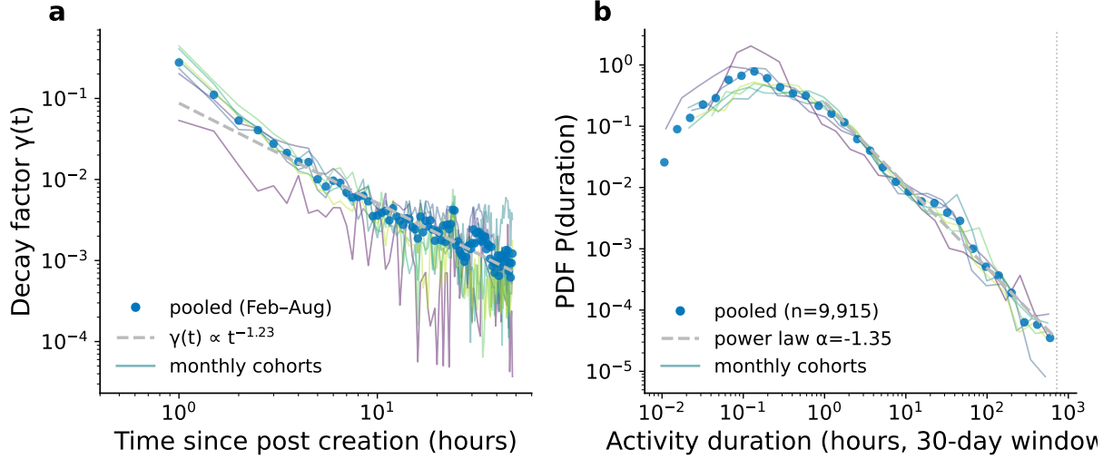
Figure 6: Temporal dynamics of engagement. (a) Decay factor \gamma(t) , the mean growth ratio of cumulative comments as a function of time since post creation; the power-law decay (fitted exponent -1.23 ) indicates that the probability of receiving new comments decreases inversely with post age. Thin lines show seven monthly cohorts (the 15th of each month, February–August 2026); markers show the pooled estimate. (b) Distribution of post activity duration (time from post creation to last comment received) measured within a fixed 30-day observation window, for the same seven monthly cohorts (thin lines) and pooled (markers; power-law tail \alpha = -1.35 ). The cohorts collapse onto a common curve, indicating the decay law is stable across the platform’s first eight months, and that while most posts become inactive within hours, some sustain engagement for days.
