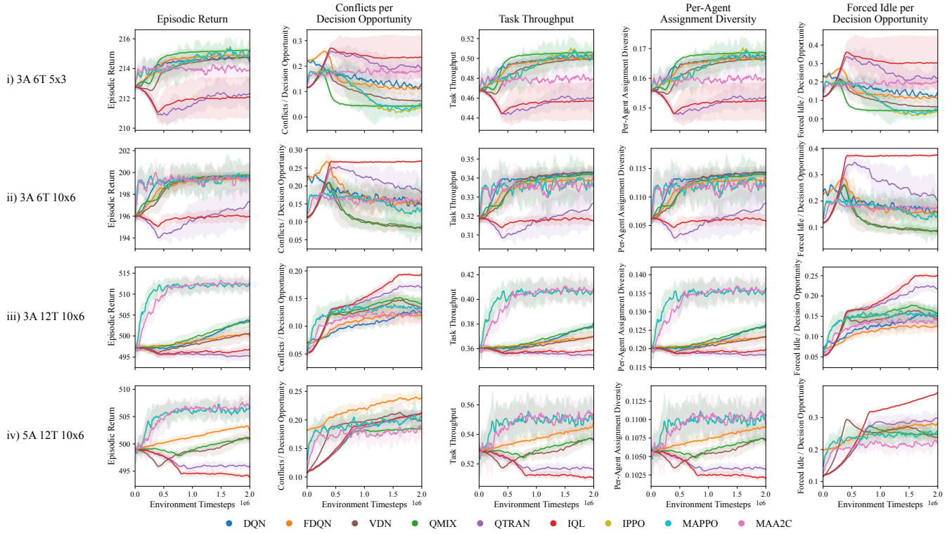
Figure 7: Learning curves for the Baseline STAT configurations. Curves show mean evaluation performance across five seeds, with shaded regions denoting 95% confidence intervals. We report episodic return as the aggregate outcome measure together with four process diagnostics: conflicts per decision opportunity, task throughput, per-agent assignment diversity, and forced idle per decision opportunity. These diagnostics capture complementary aspects of assignment interference, task-completion efficiency, division of labor, and the immediate cost of coordination failures.
