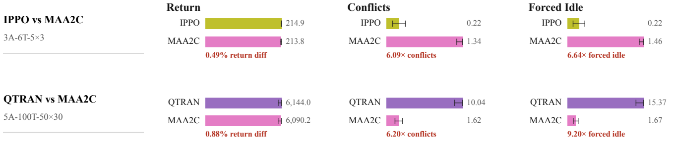
Figure 2: Example outcome-similar STAT policy pairs. Each row compares two methods whose mean returns differ by less than 1%, while assignment conflicts and forced idle differ substantially. Bars show means across five seeds with 95% confidence intervals.
