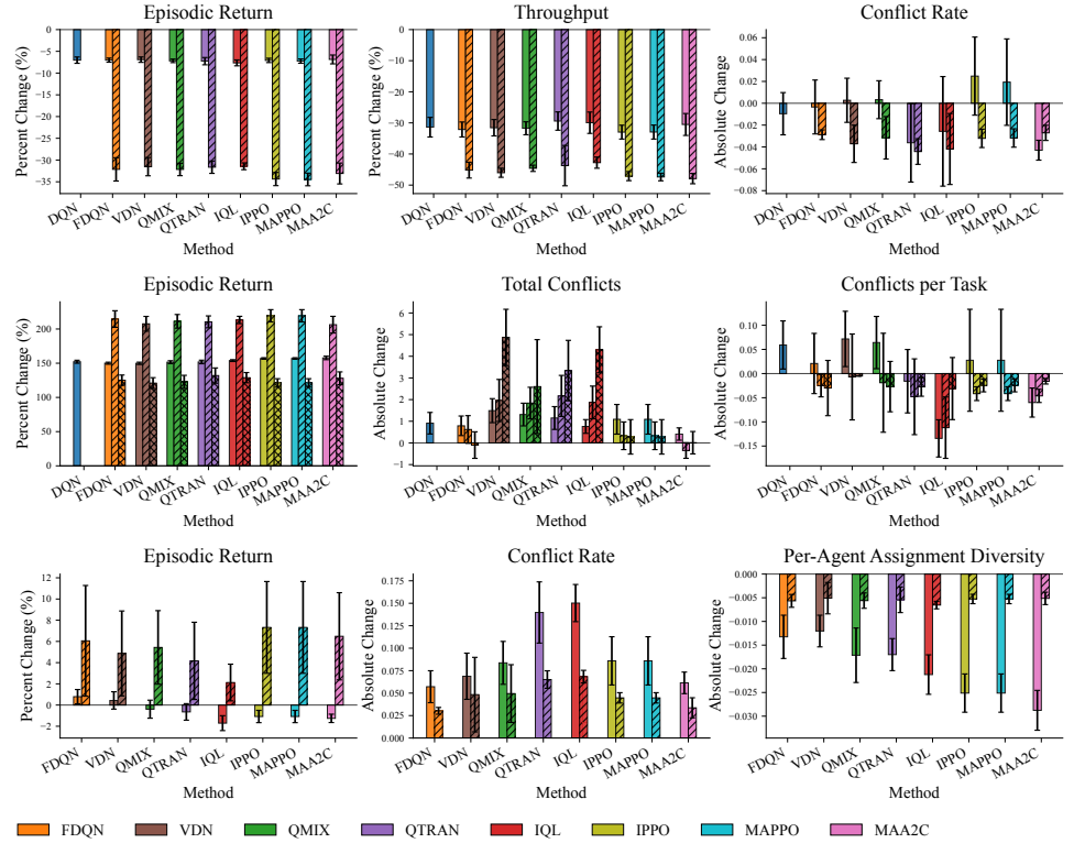
Figure 3: Process-aware analysis under controlled STAT scaling. Each row varies one configuration factor while holding the others fixed: (A) spatial extent, (B) task count, and (C) agent count. Bars show mean changes across five seeds with 95% confidence intervals.
