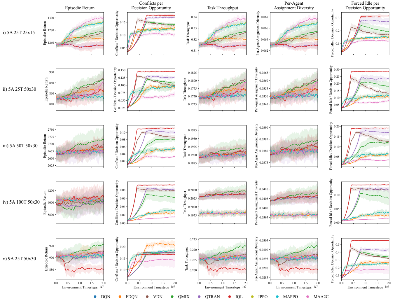
Figure 8: Learning curves for the Extreme STAT configurations. Curves show mean evaluation performance across five seeds, with shaded regions denoting 95% confidence intervals.
