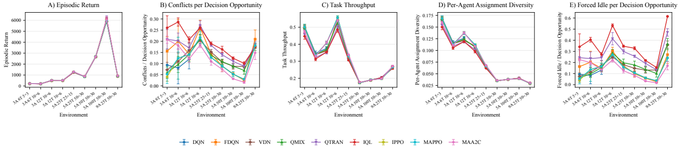
Figure 6: Final performance across all STAT configurations. Points show means across five seeds with 95% confidence intervals. Alongside episodic return, we report conflicts per decision opportunity, task throughput, per-agent assignment diversity, and forced idle per decision opportunity. The resulting profiles illustrate that strong aggregate performance does not necessarily correspond to uniformly favorable values across all coordination processes.
