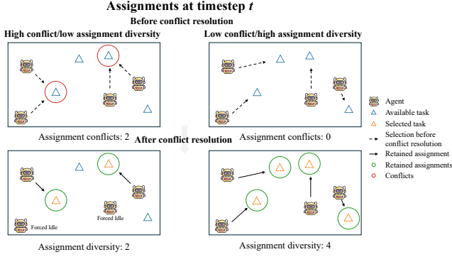
Figure 1: Illustration of STAT assignment diagnostics. The top row shows task selections before conflict resolution, and the bottom row shows the retained assignments after resolution.
