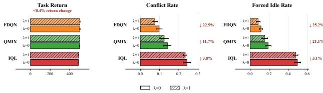
Figure 4: Reward-shaping ablation with an explicit conflict penalty in STAT. FDQN, QMIX, and IQL are trained with \lambda = 0 or \lambda = 1 , where \lambda penalizes agents that lose conflict resolution. Reported task return excludes the conflict penalty so that both conditions are compared under the same task-level objective. Bars show means across five seeds with 95% confidence intervals.
