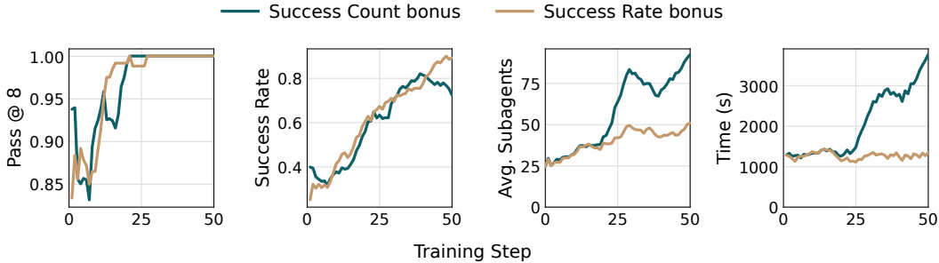
Figure 9: Ablation comparing success count vs. rate delegation bonus on TEXTCRAFT-SYNTH, plotting the success curves, sub-agent count and time per training step.
