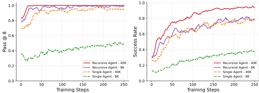
Figure 4: TEXTCRAFT-SYNTH training curves (moving average; window size 10).
