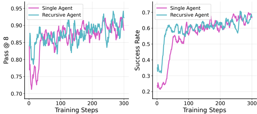
Figure 11: ART-E (Email Search) training curves for Qwen-3-14B (moving average; window size 10).
