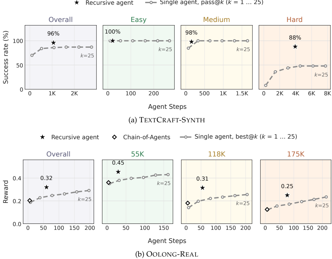
Figure 10: Comparison of the trained recursive agent with a trained single agent under idealized best-of- k and chain-of-agents harnesses. We vary k \in \{1, 5, 10, 15, 20, 25\} and plot overall and per-difficulty success rates/rewards as a function of the number of agent steps used by each configuration. Sampling more does not substitute for delegating: the recursive agent (★) lies above the best-of- k frontier while using less inference-time compute, despite best-of-25 consuming 2.6\times\text{--}3.3\times more agent steps.
