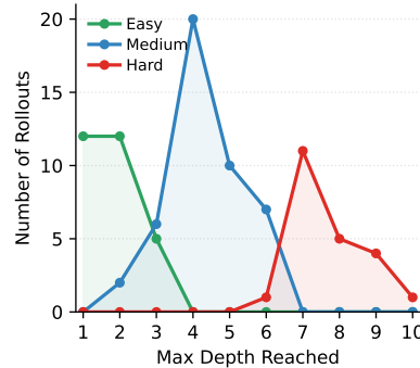
Figure 7: Maximum delegation depth on TEXTCRAFT-SYNTH.
