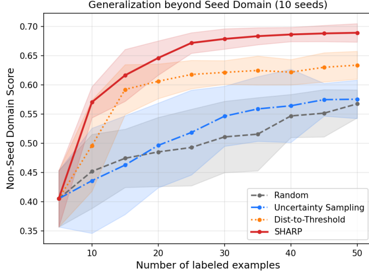
Figure 2: Non-Seed Domain Score learning curves (mean \pm 1 s.d. over 10 seeds) for SHARP and the unstratified baselines. All methods start from an identical supply-gap-only seed ( n_0 = 5 ). Algorithm 1 leads the unstratified baselines at every budget level, finishing at 0.690 vs. 0.634 for Dist-to-Threshold. The stratified controls, not plotted, track SHARP within one s.d. throughout and finish at 0.690 (Stratified Random) and 0.687 (Stratified DtT); see the text.
