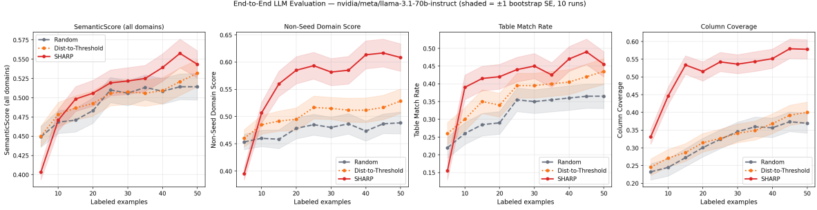
Figure 4: End-to-end LLM evaluation vs. annotation budget for SHARP and the unstratified baselines; panels from left to right show SemanticScore, Non-Seed Domain Score, Table Match Rate, and Column Coverage (shaded bands: \pm 1 bootstrap SE over 10 seeds; Stratified Random is reported in Table 2). Algorithm 1 trails at n \leq 10 on overall SemanticScore but leads from n = 15 onward, finishing at 0.543 vs. 0.532 for Dist-to-Threshold and 0.514 for Random. The Non-Seed Domain Score (second panel) shows Algorithm 1’s cross-domain advantage emerging from n = 10 , peaking at 0.617 at n = 45 , and finishing at 0.608 vs. 0.528 for Dist-to-Threshold.
