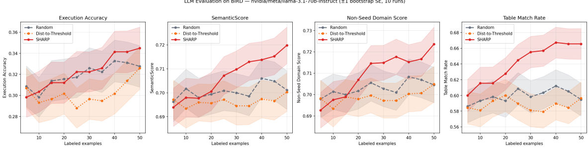
Figure 7: BIRD LLM evaluation learning curves for SHARP and the unstratified baselines ( \pm 1 bootstrap SE, 10 seeds, 58 test queries each; Stratified Random is reported in Tables 7 and 8). SHARP leads on SemanticScore from n = 20 onward and on Table Match Rate at every budget. Execution accuracy differences are within one standard error across all methods throughout the budget.
