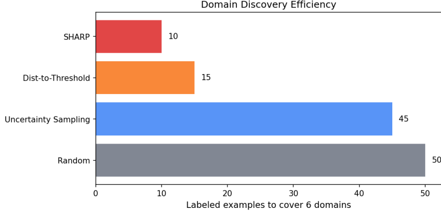
Figure 3: Annotation efficiency: labeled examples needed to first reach 6-domain coverage (of 7 domains), for SHARP and the unstratified baselines. Algorithm 1 reaches 6-domain coverage at n = 10 , as do the two stratified controls (not plotted; their curves coincide with SHARP’s); Dist-to-Threshold reaches 6 domains at n = 15 ; Random requires the full n = 50 budget to reach 6 domains. No method achieves full 7-domain coverage within the n = 50 budget.
