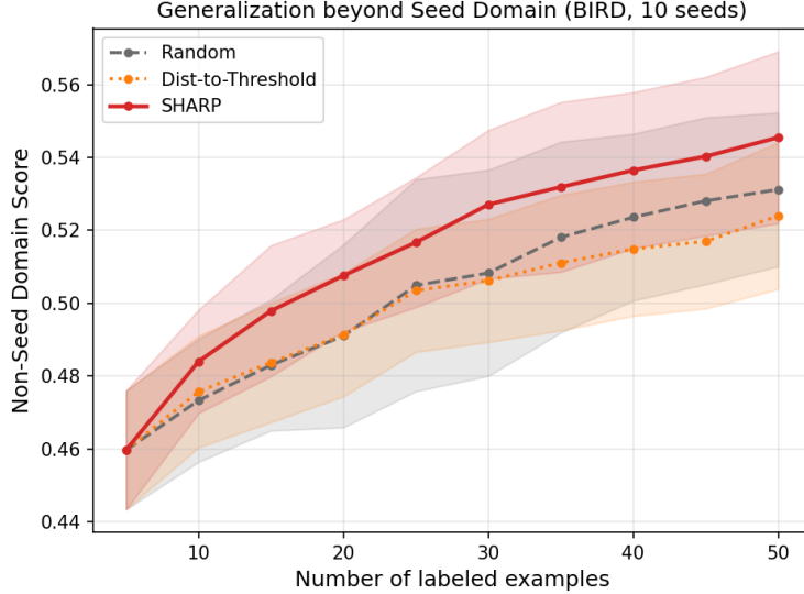
Figure 6: BIRD retrieval simulation: Non-Seed Domain Score (mean \pm 1 s.d., 10 seeds) for SHARP and the unstratified baselines; the stratified controls are reported in Table 6. SHARP leads from n = 10 onward, finishing at 0.545 vs. 0.531 for Random and 0.524 for Dist-to-Threshold.
