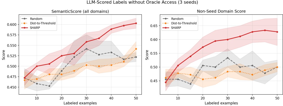
Figure 5: LLM-scored-label experiment: SemanticScore (left) and Non-Seed Domain Score (right) vs. annotation budget (mean \pm 1 SE over 3 seeds). Labels are computed by calling the LLM on each annotated example and scoring with the production formula (Equation 23); no oracle test SQL is observed during the loop. Selection under Algorithm 1 is label-free in this configuration (Remark 1); Random and Dist-to-Threshold serve as baselines. The DDL schema is included in all prompts.
