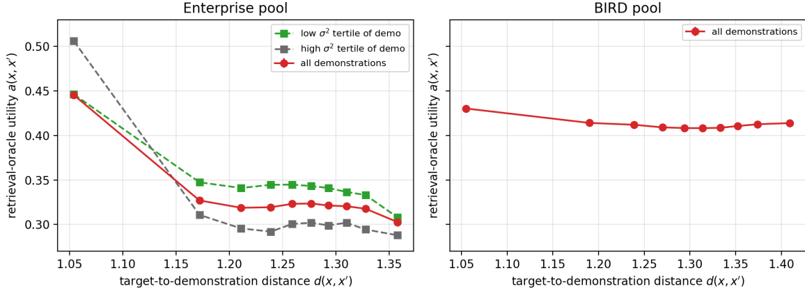
Figure 1: Calibration of Assumption 2 with the retrieval-oracle proxy a(x, x') = \text{SemanticScore}(s_{x'}, s_x) . Mean utility by decile of the target-to-demonstration distance ( \pm 1 SE), all ordered pairs. Enterprise (left) also splits demonstrations by tertile of their self-consistency noise \sigma^2(x') ; the high-noise curve’s nearest-decile value is confounded with the dense seed domain. Both panels share the vertical scale. Utility is high only in the nearest decile and flat beyond it; the near-to-far gap is 0.12 on the enterprise pool and 0.02 on BIRD.
