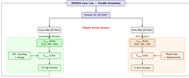
Fig. 1. Dual Actor-Critic architecture. The locomotion branch (green) and arm branch (orange) maintain separate critics with disjoint reward streams. Observation widths are those of the main comparison (S6s); the S7 variant adds three anti-gaming features to the arm branch (55-dim) and freezes the locomotion branch. The unified variant (not shown) concatenates both observation streams into a single 109-dim critic input.
