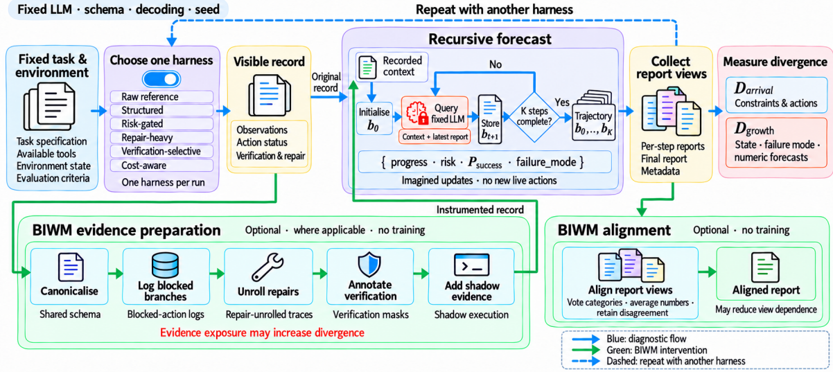
Figure 2: Harness-to-belief instrumentation pipeline. (a) A fixed task, LLM, schema, decoding procedure, and seed isolate harness-induced arrival and growth divergence through recursive belief forecasts. (b) BIWM evidence preparation exposes blocked, repaired, verified, and shadow evidence, which may increase measured divergence. (c) BIWM alignment reconciles cross-harness report views and may reduce view dependence.
