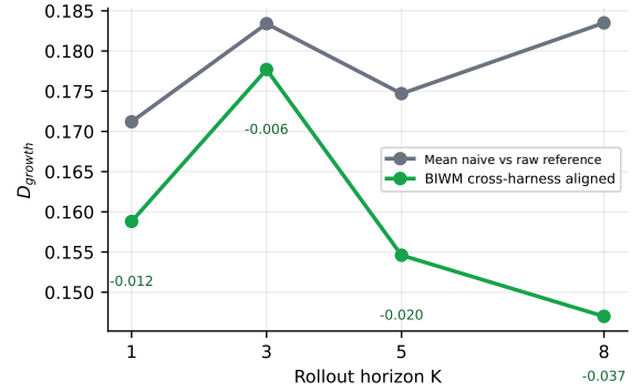
Figure 3: Cross-harness alignment reduces growth divergence across horizons. The reduction increases from 0.012 at K = 1 to 0.037 at K = 8 .
