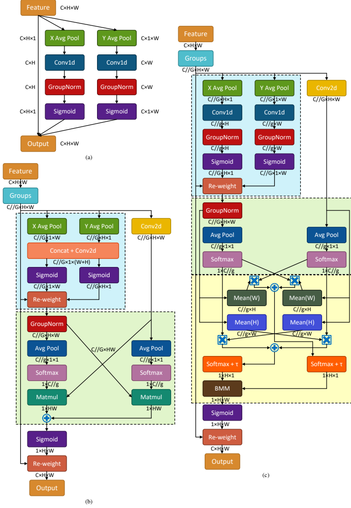
Fig. 5. Architectures of (a) ELA, (b) EMA, and (c) CEA.
