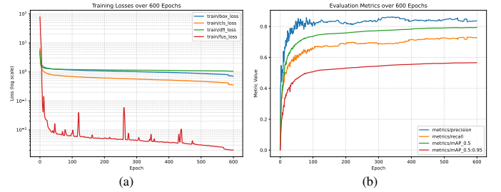
Fig. 10. Evolution of training losses and evaluation metrics for CFGPNet-m on the MFAD dataset during 600 training epochs: (a) box, class, DFL, and fusion loss values; (b) precision, recall, mAP@50, and mAP@50:95 scores.
