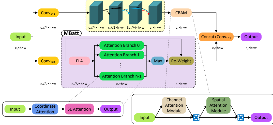
Fig. 6. Architecture of the ASAF network.
