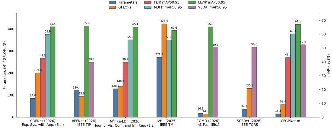
Fig. 1. CFGPNet-m versus state-of-the-art multispectral detectors.
