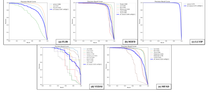
Fig. 9: Illustration of precision-recall curves for CFGPNNet-e on (a) FLIR, (b) M3FD, (c) LLVIP, (d) VEDAI, and (e) MFAD datasets.
