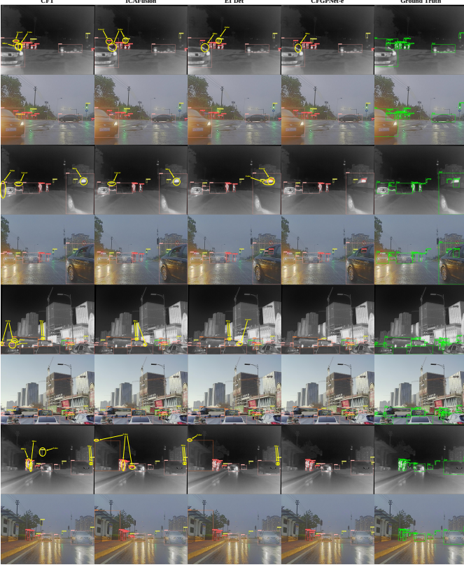
Fig. 12. Illustration of inference results for CFT, ICAFusion, EI 2 Det, and CFGPNet-e on the M3FD dataset. The yellow arrow annotations show "Miss" (missed detection), "False" (false alarm), "Lower" (low-confidence detection), and "BBox" (inaccurately positioned bounding boxes).
