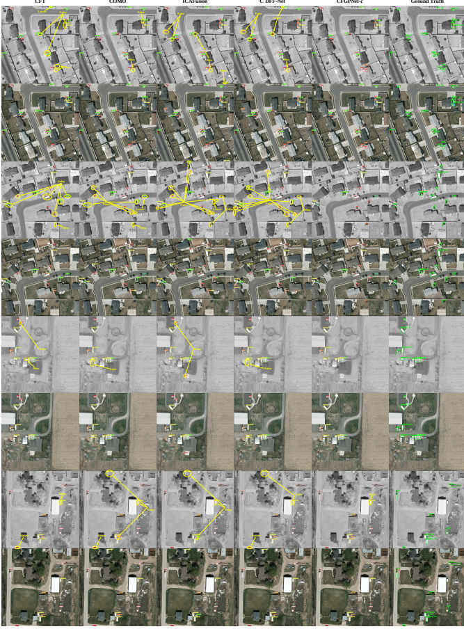
Fig. 14. Illustration of inference results for CFT, COMO, ICAfusion, C 2 DFF-Net, and CFGPNet-c on VEDAI Split 1. The yellow arrow annotations show "Miss" (missed detection), "False" (false alarm), "Lower" (low-confidence detection), and "BBox" (inaccurately positioned bounding boxes).
