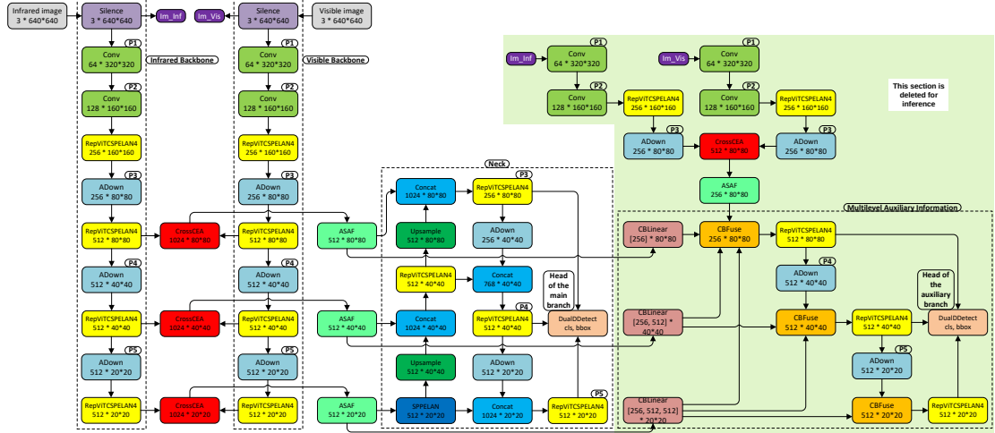
Fig. 2. Overview of the proposed CFQNet framework. The auxiliary branch (green area) is used only during training for gradient enhancement and is removed during inference. The Silence module splits the six-channel input into two three-channel tensors: infrared (channels 1–3) and visible (channels 4–6). The diagram reports each module name, the number of output channels in brackets, and the output spatial dimension, all based on a 640 \times 640 input image size.
