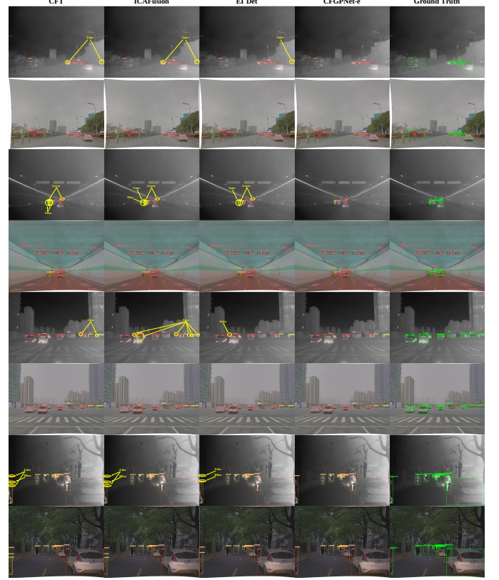
Fig. 15. Illustration of inference results for CFT, ICAfusion, EI 2 Det, and CFGPNet-e on the MFAD dataset. The yellow arrow annotations show "Miss" (missed detection), "False" (false alarm), "Lower" (low-confidence detection), and "BBox" (inaccurately positioned bounding boxes).
