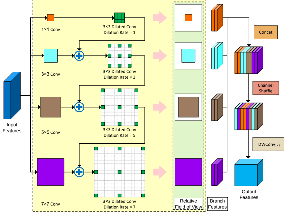
Fig. 4. Architecture of the MFE module.
