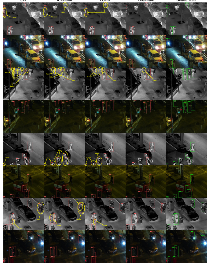
Fig. 13. Illustration of inference results for CFT, ICAFusion, COMO, and CFGPNet-e on the LLVIP dataset. The yellow arrow annotations show "Miss" (missed detection), "False" (false alarm), "Lower" (low-confidence detection), and "BBox" (inaccurately positioned bounding boxes).
