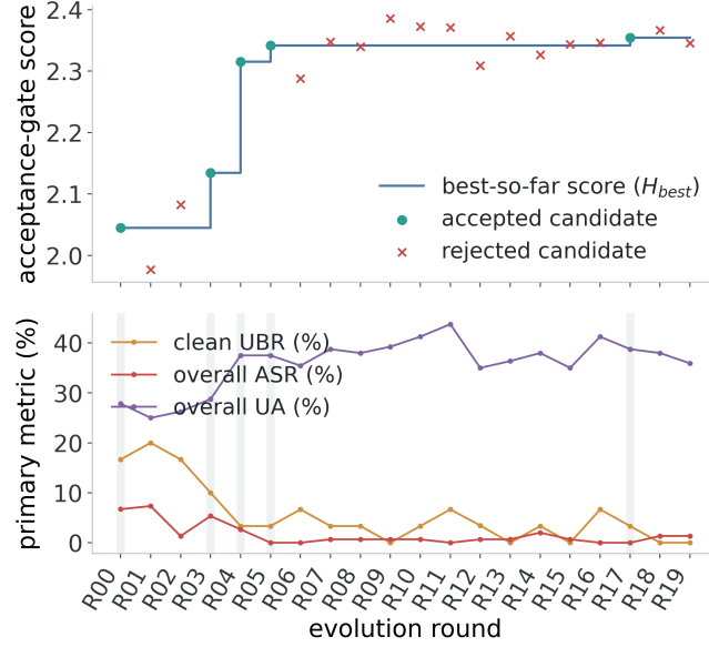
Figure 7: Evolution history under best-so-far selection. Top: accepted and rejected candidate scores, with the step curve denoting the retained harness. Bottom: Clean UBR, overall ASR, and overall UA across rounds. Shaded columns mark accepted updates.
