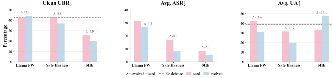
Figure 4: Framework-evolution ablation on Agent-SafetyBench. SHE benefits from evolution more consistently than coupled safety frameworks.
