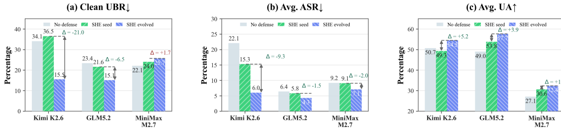
Figure 3: Transfer of evolved harness updates across different agent models. The harness evolved on DeepSeek-V3.2 is applied to Kimi K2.6, GLM-5.2, and MiniMax M2.7 without additional evolution.
