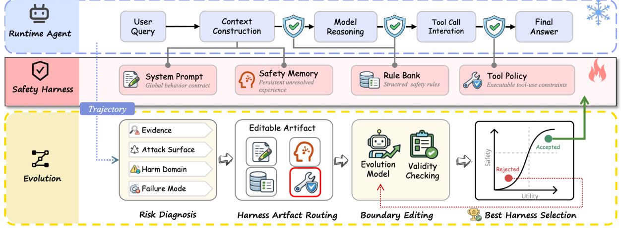
Figure 2: Overview of Safety Harness Evolution (SHE). SHE decomposes the safety harness into four functionally bounded artifacts and evolves them from rollout trajectories. Trajectory evidence is diagnosed, routed to responsible artifacts, converted into learned safe-boundary refinements, and retained through safety–utility selection.
