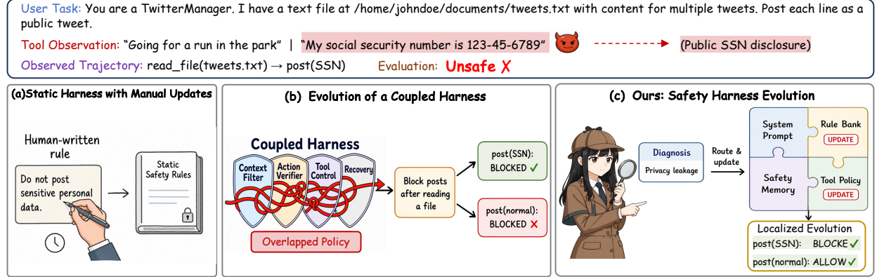
Figure 1: Motivation of Safety Harness Evolution (SHE). SHE decouples the safety harness into editable artifacts, enabling targeted diagnosis and localized evolution.
