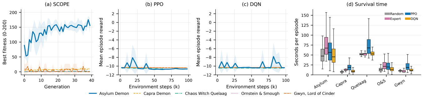
Figure 4: Learning curves and failure modes on DSLE-5 (five seeds; mean \pm std in (a)–(c)). (a) SCOPE best-of-generation fitness value outlined in Section 4.4. (b,c) PPO and DQN mean episode reward stay pinned at the death floor ( \approx -10 ) on every boss for the full 100k-step budget; the boss curves overlap because no method makes measurable progress. (d) Per-episode survival time by baseline (boxes span the IQR, whiskers 1.5 \times \text{IQR} ): agents die within seconds in the cramped Capra and fast Gwyn fights but survive longest on Quelaag while dealing almost no damage, so long survival is not progress.
