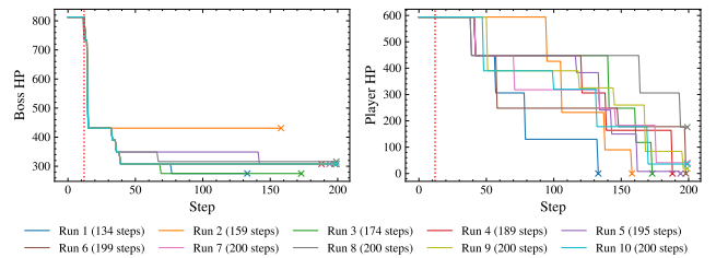
Figure 3: Asylum Demon stochasticity replay test. Ten runs begin from the same save state and execute the same set of actions. The two panels show boss-health and player-health trajectories. Despite identical replayed inputs, the health trajectories diverge by step 12.
