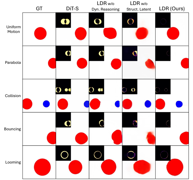
Figure 3: Qualitative OOD comparison under single-task training. For each task and each method, we show a predicted frame and its error map (darker is better). LDR stays close to the GT, while the baseline and both ablations drift.
