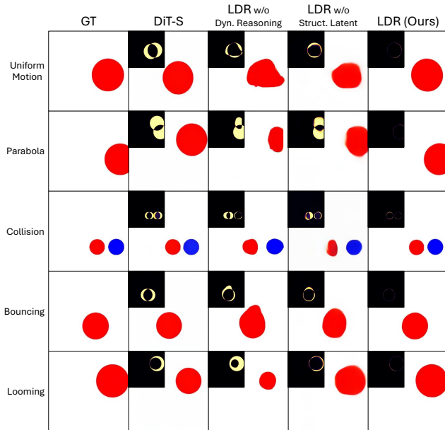
Figure 4: Qualitative OOD comparison under joint five-task training. A single model holds all five tasks, yet LDR still stays close to GT while the others drift.
