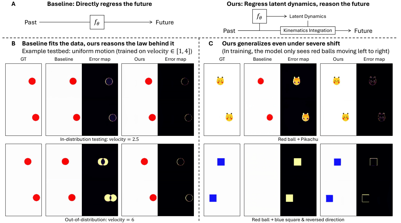
Figure 1: Learning how the world evolves. (A) Baseline method directly regresses the future, whereas our method regresses latent dynamics and reasons the future via kinematic integration. (B) Both match the ground truth (GT) in-distribution (ID), but only ours stays close to GT out-of-distribution (OOD). (C) Trained only on red balls moving left to right, LDR extrapolates the learned dynamics to a Pikachu and to a blue square moving right to left, while the baseline fails.
