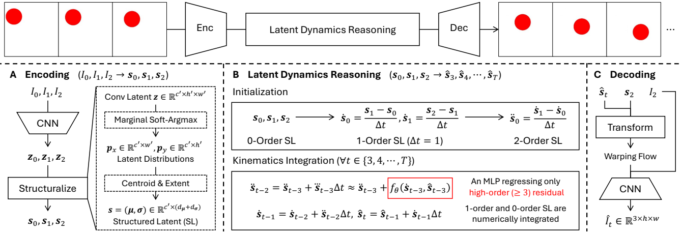
Figure 2: Overview of LDR. Given three conditioning frames I_0, I_1, I_2 , LDR predicts the future frames \hat{I}_3, \hat{I}_4, \dots, \hat{I}_T in three stages. (A) LDR first encodes each input frame into a structured latent (SL). (B) LDR measures the low-order time derivatives of the given SL, then rolls out by regressing only the high-order residual with f_\theta and numerically integrating the lower orders to the next latent \hat{s}_t ( t \in \{3, 4, \dots, T\} ). (C) LDR finally decodes each predicted latent to an RGB frame \hat{I}_t .
