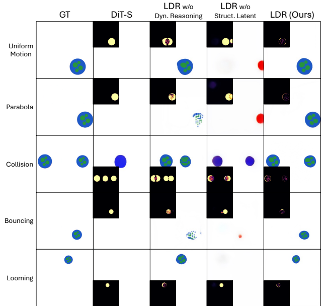
Figure 5: Stress test under severe OOD shift. Trained only on red balls but tested on an unseen object (e.g., ‘‘earth’’), LDR still predicts the correct motion, while the others fail.
