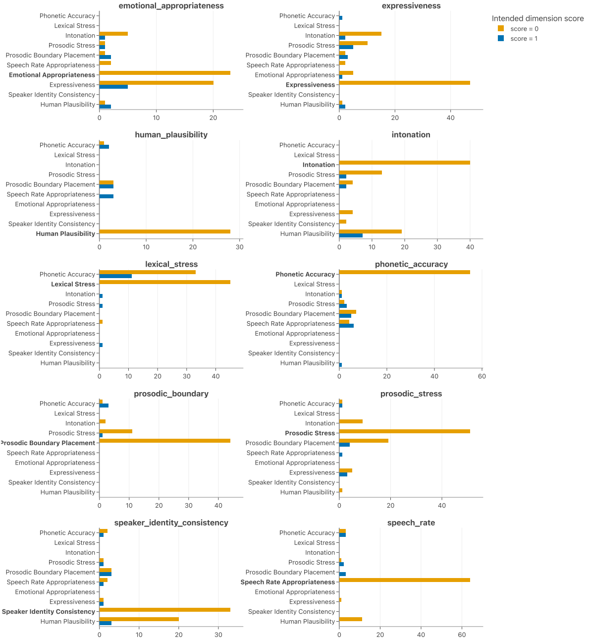
Figure 2: Co-occurrence of perceptual failures across speech quality dimensions. Per-dimension failure counts stratified by intended-dimension ground-truth label. Each subplot corresponds to one intended dimension (column panels); bars show the number of score-0 (failure) observations on each rating dimension (y-axis), split by whether the sample’s ground-truth label on its own intended dimension is a failure (orange, score = 0) or a pass (blue, score = 1). Tall blue bars on dimensions other than the intended one reveal that samples annotated as passing on their intended construct nonetheless exhibit failures on unrelated dimensions.
