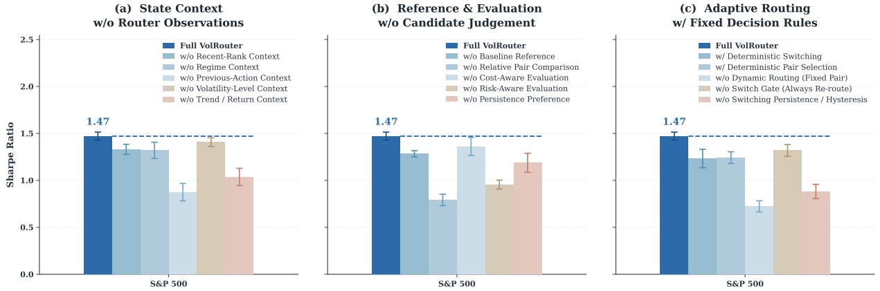
Figure 4: Component ablation on S&P 500. Panels remove (a) state context, (b) candidate-reference/evaluation signals, and (c) adaptive-routing components. Full VolRouter has Sharpe 1.47 under this ablation protocol. Error bars summarize the ablation driver and are not confidence intervals for Table 1.
