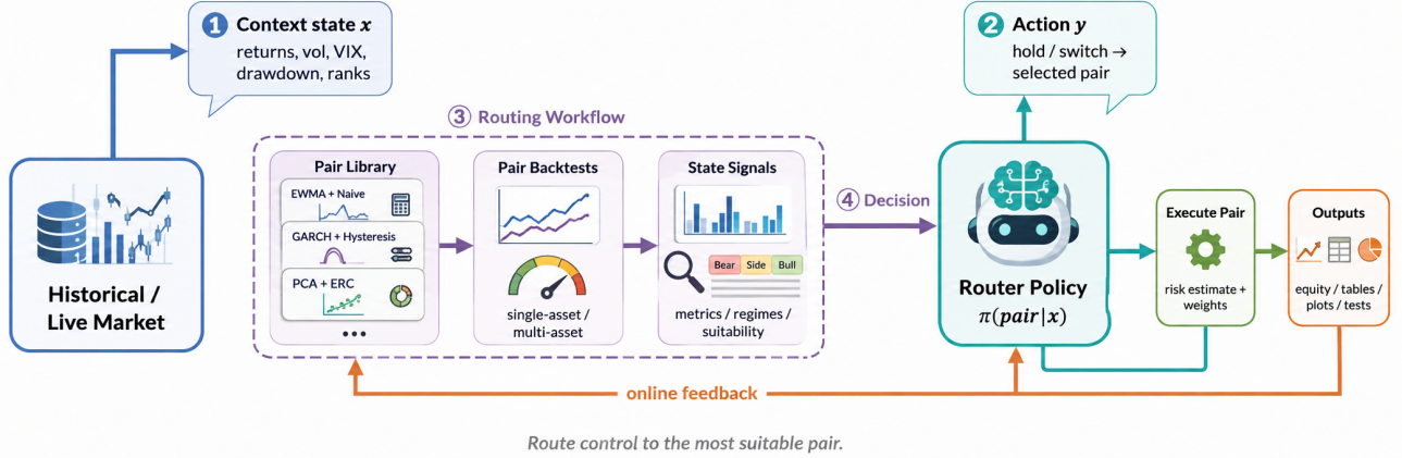
Figure 2: Overview of VolROUTER. Market history is summarized into a control-relevant profile. The Router interprets the state, decides whether the active pair should be kept, and selects a replacement only when switching is justified. The selected estimator-controller pair then produces the portfolio action; the LLM, when used, never produces the trade directly.
