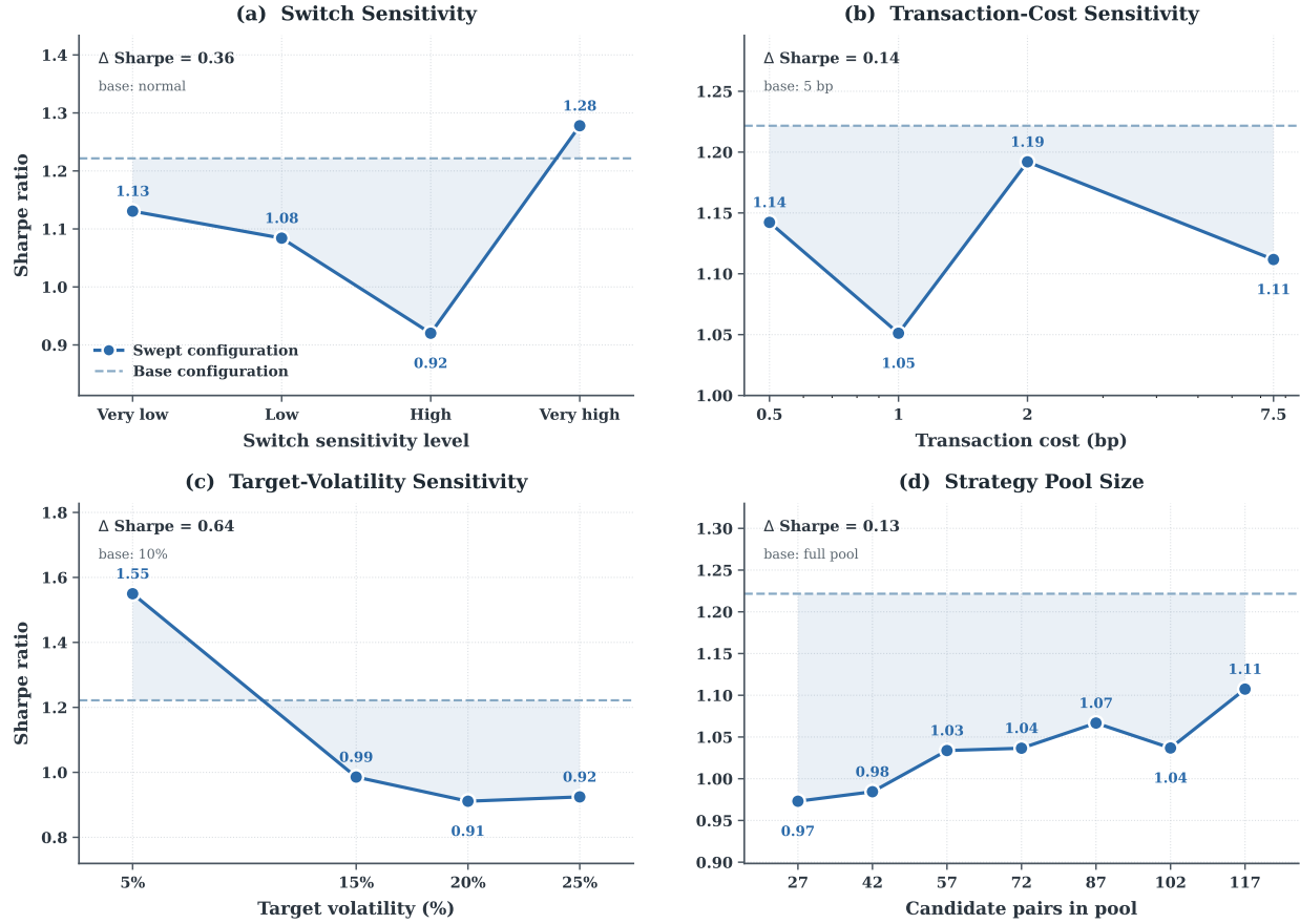
Figure 5: Sensitivity of VolRouter. We vary (a) switching sensitivity, (b) transaction cost, (c) target volatility, and (d) candidate-pool size one at a time. Dashed lines mark the canonical base configuration; the base need not be one of the displayed sweep points.
