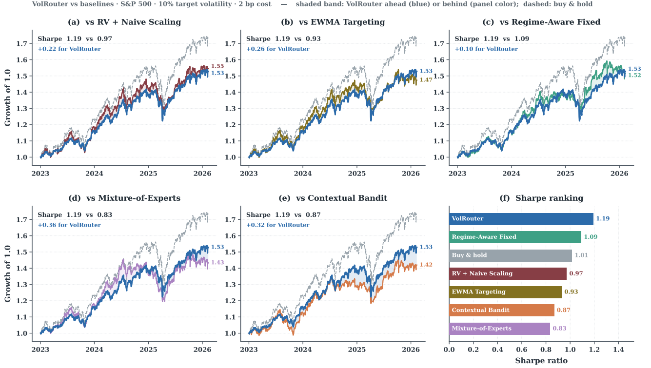
Figure 3: Path-level S&P 500 diagnostic under a 10% volatility target and 2 bp costs. Panels (a)–(e) compare cumulative wealth and panel (f) reports Sharpe ratios. This run is separate from the 5 bp headline setting in Table 1 and is used only to show when path-level differences accumulate.
