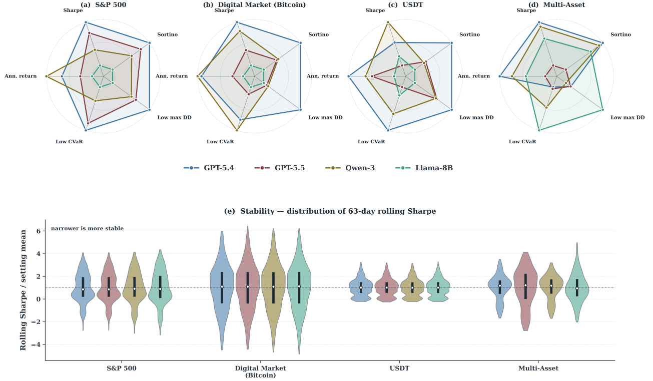
Figure 6: Router backbones across markets. Panels (a)–(d) compare normalized return and risk metrics; panel (e) shows 63-day rolling-Sharpe distributions after within-setting normalization. In the S&P 500 sweep, the regime series is held fixed, isolating downstream switch and pair-selection behavior.
