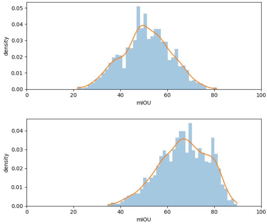
Figure 7: Distribution of the per-image IoU of U-Net on the CRACK500 test set, shown as histograms with kernel density estimates. Top: real training images only (Naive). Bottom: real training images and the synthetic data of the proposed pipeline.
