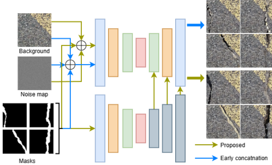
Figure 1: Mask conditioning by early concatenation with the network input, as in CDM [12] (blue arrows), and by a separate control branch, as in the proposed model (olive arrows), with results for the same masks. With early concatenation, the rendered cracks deviate from the mask shape. With the control branch, they follow the masks more closely.
