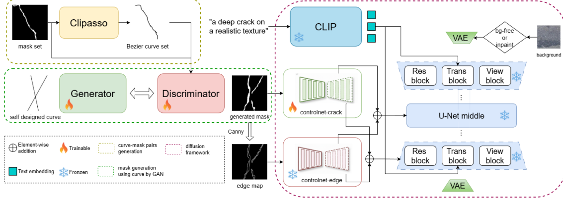
Figure 2: Overview of the pipeline. Top left: CLIPasso converts real crack masks into Bézier curves, which gives curve-mask pairs. Bottom left: a GAN trained on these pairs translates Bézier curves into crack masks. Right: ControlNet-Crack, conditioned on the mask, and ControlNet-Edge, conditioned on its Canny edge map, guide Stable Diffusion in background-free or inpainting mode.
