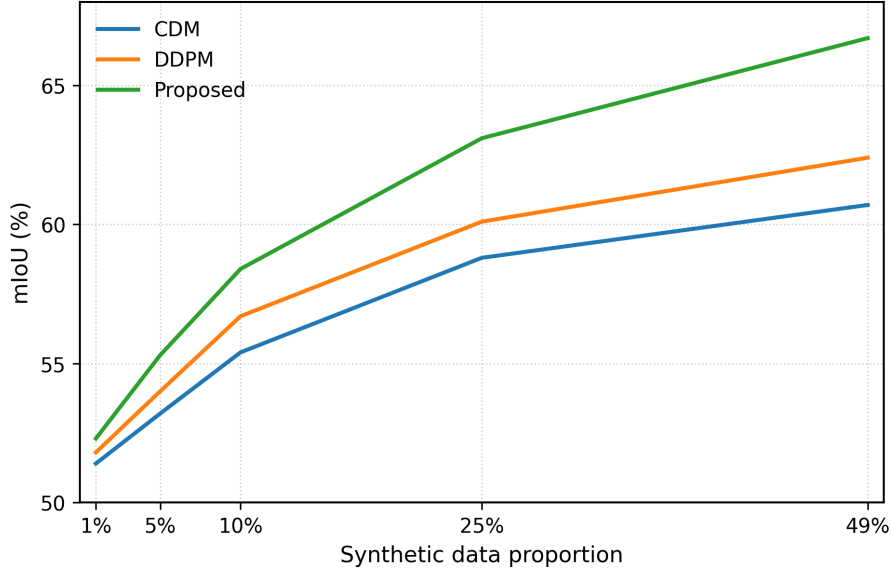
Figure 6: mIoU of U-Net on the CRACK500 test set versus the proportion of synthetic images in the training set for CDM (blue), DDPM (orange) and the proposed method (green). The 49% setting corresponds to Table 3.
