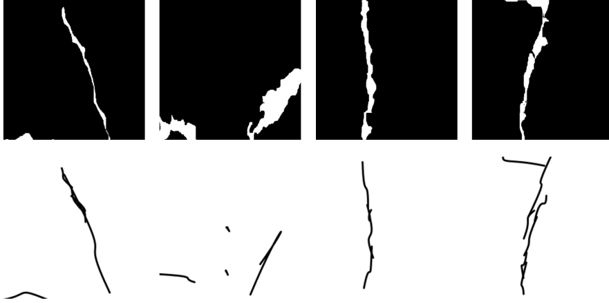
Figure 3: Examples of the inverse mapping from raster masks to Bézier curves. Top: Real crack masks used as input. Bottom: The corresponding Bézier curve sketches automatically generated by the CLIPasso model. This automated pipeline is used to create the paired dataset for training our mask synthesis GAN.
