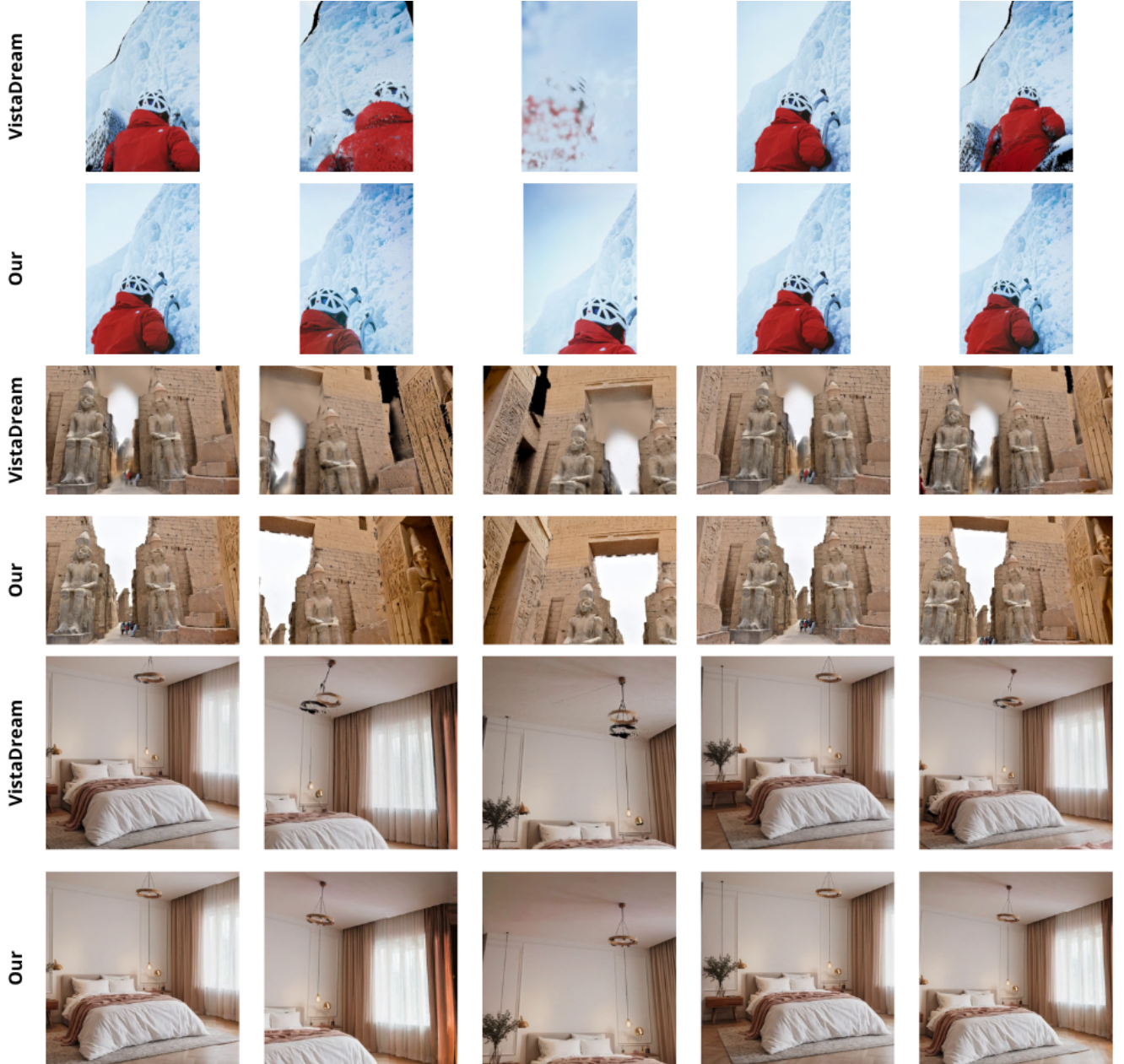
Figure 3. Qualitative comparison with VistaDream. Each pair of rows shows matched novel views rendered by VistaDream (top) and ORCA (bottom) along the same camera trajectory. VistaDream exhibits uncovered regions, Gaussian-like artifacts, and blurring in challenging viewpoints, whereas ORCA produces more complete and spatially coherent renderings while better preserving scene structure across views.
