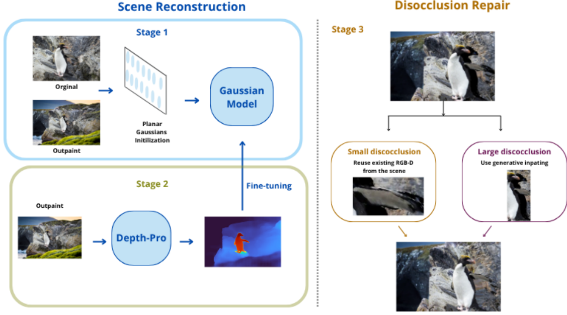
Figure 2. Starting from the original and outpainted images, we initialize and optimize a planar Gaussian scene representation. Monocular depth is then used to deform the learned Gaussian geometry, and the resulting representation is fine-tuned while keeping the deformed Gaussian positions fixed. During novel-view exploration, small disocclusions are repaired using RGB-D information already available in the scene, whereas larger unseen regions are completed with generative inpainting.
