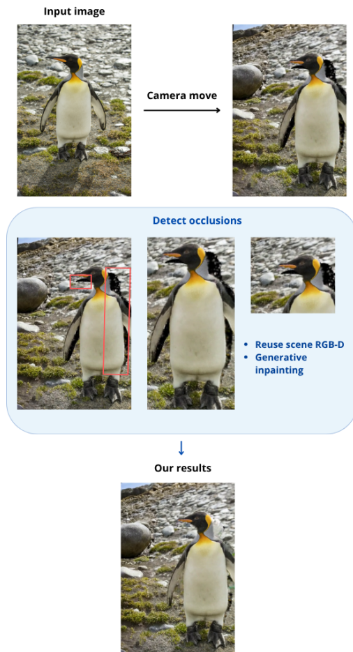
Figure 1. Camera motion reveals disoccluded regions that are not covered by the initial reconstruction. ORCA reuses existing scene information whenever possible and applies generative completion only to regions that cannot be reliably recovered from the reconstructed scene.
