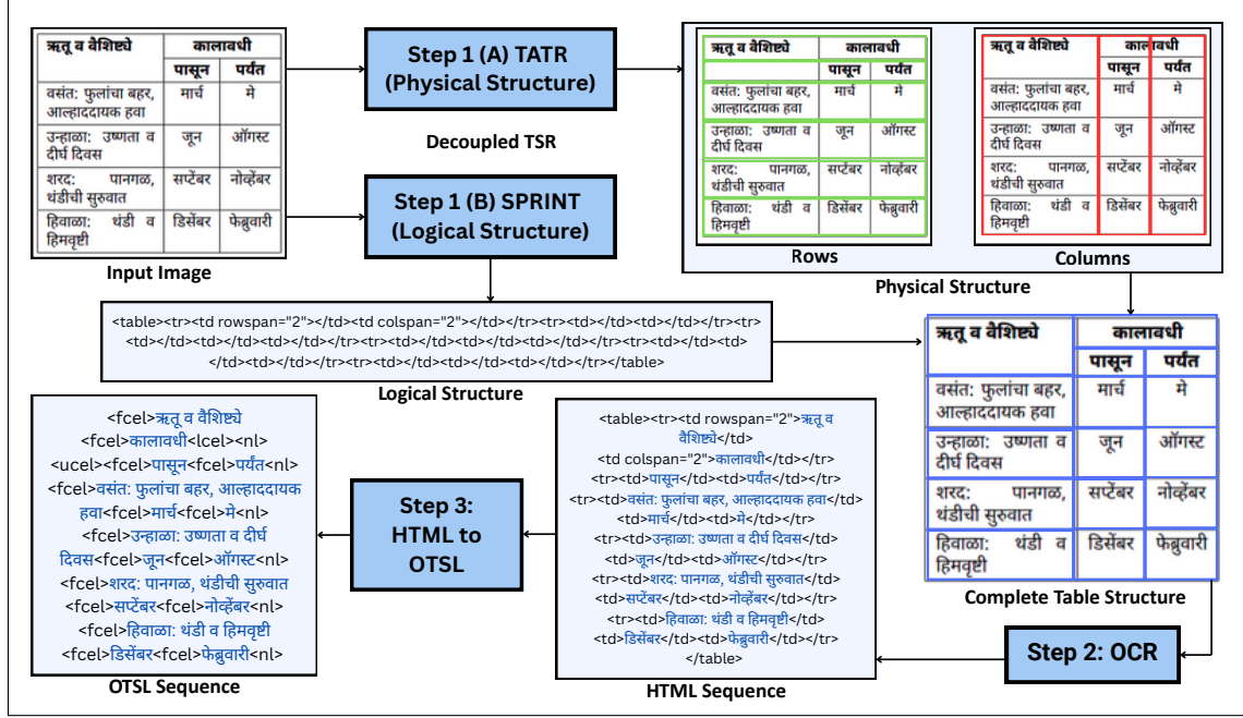
Figure 2. DELTA overview: given a table image, the system first performs decoupled TSR (physical structure through TATR and logical structure through SPRINT), followed by OCR to extract table content. The resulting HTML is converted into a compact OTSL sequence.
