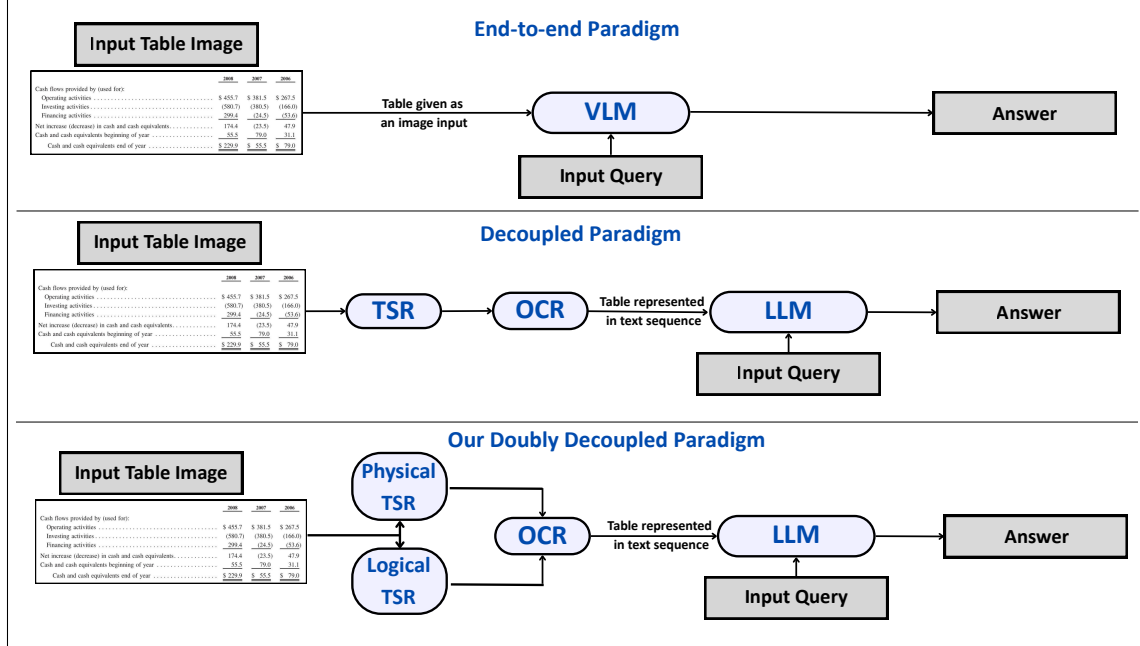
Figure 1. TabVQA paradigms: (i) end-to-end, where a VLM directly processes the table image and question; (ii) decoupled, where TSR + OCR extracts structure and content into text (HTML, OTSL) for an LLM; and (iii) our doubly decoupled approach, which further separates physical and logical TSR for better control. The steps following OCR remain the same as for the conventional decoupled approach.
