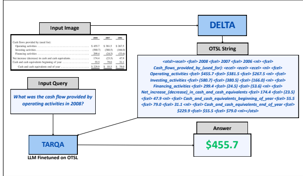
Figure 4. TARQA, an LLM fine-tuned on OTSL sequence, uses output from DELTA along with the query to generate answers.
