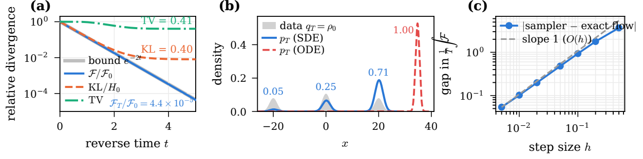
Figure 1: One-dimensional Gaussian mixture with exact scores, wrong initialization p_0 = N(10, 0.5^2) . (a) \mathcal{F}/\mathcal{F}_0 against the bound e^{-2t} of Theorem 3.2, \text{KL}/H_0 , and TV along the exact reverse SDE. (b) Terminal laws of the reverse SDE and of the probability-flow ODE from the same initialization. (c) Gap between the time-averaged \mathcal{F}(\hat{p}_t \| q_t) of the frozen-score integrator and its exact-flow counterpart \mathcal{F}(p_t \| q_t) versus step size (log-log).
