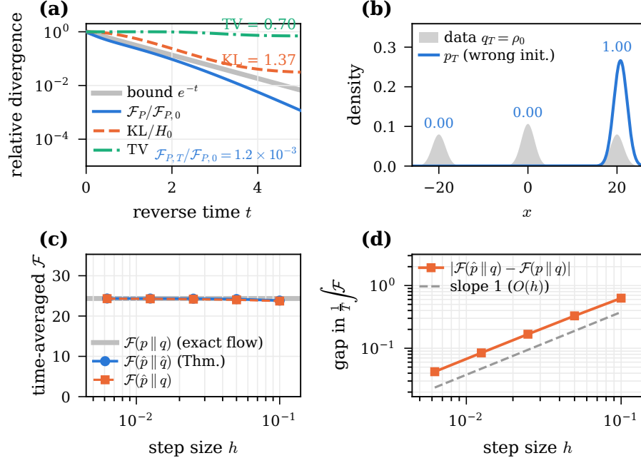
Figure 2: The critically damped experiment ( \gamma = 2 , \xi = 1 ), presented as in Figure 1. (a) Along the exact reverse flow, the modified Fisher divergence \mathcal{F}_P contracts faster than the guaranteed e^{-t} , KL decreases monotonically, and TV plateaus. (b) Terminal position marginal. (c) The frozen-score exponential integrator (5.4): the time-averaged \mathcal{F}(\hat{p} \parallel \hat{q}) of Theorem 5.5 (circles) and the time-averaged \mathcal{F}(\hat{p}_t \parallel q_t) against the exact marginals along the frozen-score SDE interpolation (squares) versus step size, with the exact-flow value \frac{1}{T} \int_0^T \mathcal{F}(p_t \parallel q_t) dt (gray). (d) Gap between the time-averaged \mathcal{F}(\hat{p}_t \parallel q_t) of (c) and its exact-flow counterpart \mathcal{F}(p_t \parallel q_t) versus step size (log-log; dashed: slope one), as in Figure 1(c).
