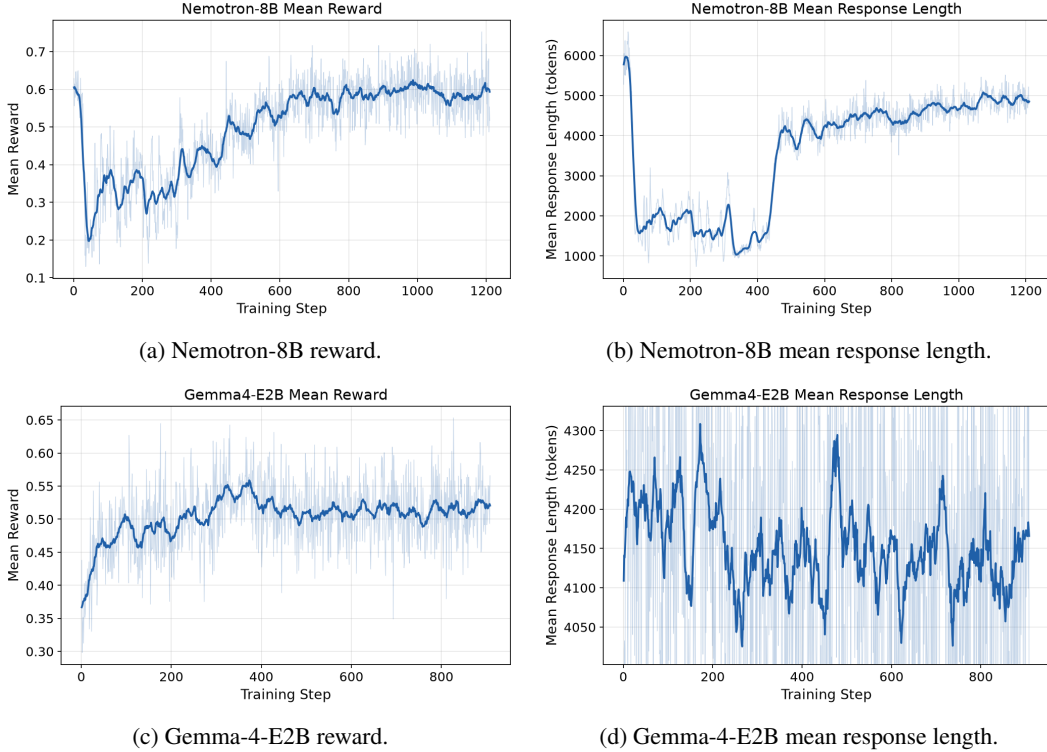
Figure 9: Length-penalty GRPO training curves .
