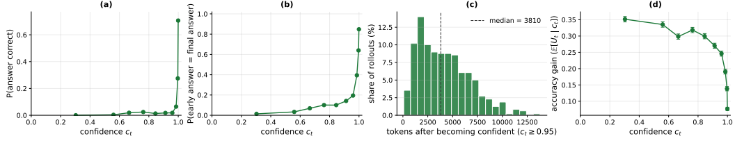
Figure 6: Gemma-4-E2B counterpart of Figure 2.
