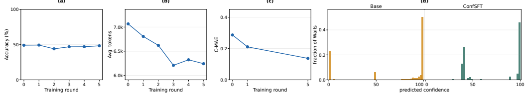
Figure 7: Gemma-4-E2B counterpart of Figure 4.
