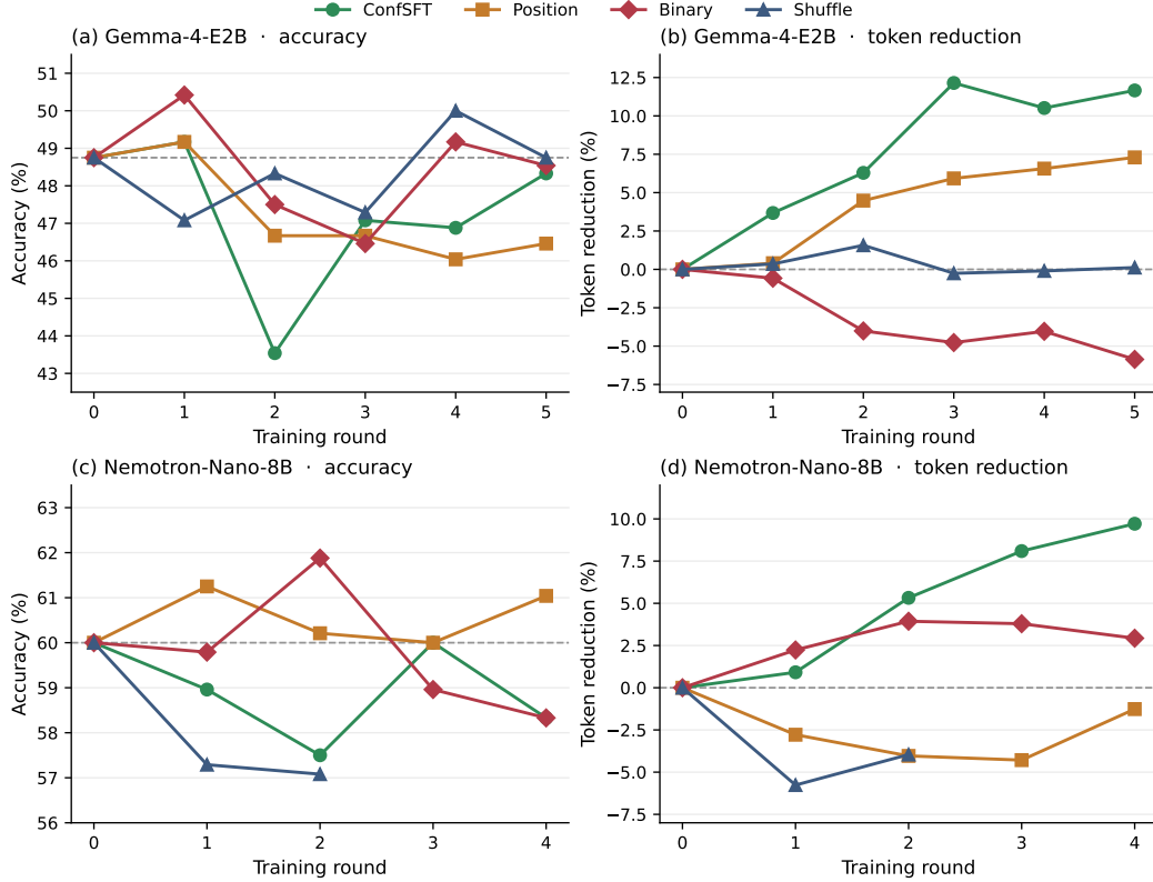
Figure 8: Accuracy (left) and token reduction (right) over training rounds for the four supervision signals in Table 2, AIME 2024 validation. Dashed lines mark the pre-SFT baseline.
