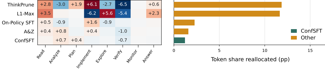
Figure 5: Different efficiency methods reshape reasoning in different ways. Following the Schoenfeld-style episode taxonomy, we compare each efficient policy with its corresponding base policy. Left: change in reasoning-token share for each episode, in percentage points. Right: total variation distance between the before- and after-training episode distributions.
