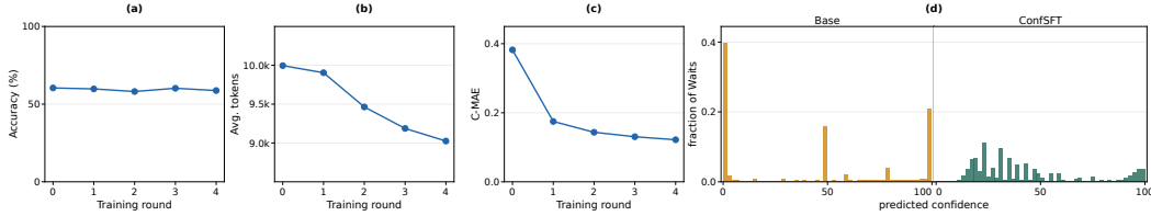
Figure 4: Training Dynamics. (a) Accuracy remain stable. (b) Generated tokens decrease. (c) Confidence predictions improved. (d) Confidence predictions become more graded.
