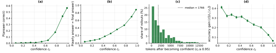
Figure 2: (a) Trial-answer correctness and (b) agreement with the final answer increase with confidence. (c) The model often continues generating after first reaching c_t \geq 0.95 . (d) The expected accuracy gain from further reasoning decreases with confidence.
