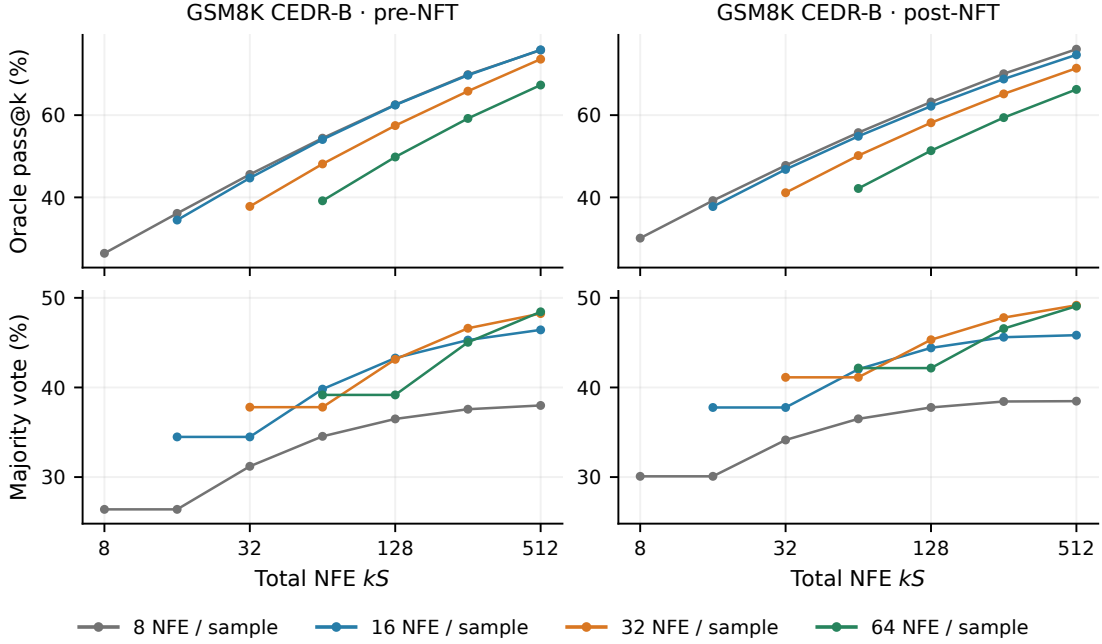
Figure 8: GSM8K CEDR-B before and after NFT. Upper panels show oracle pass@ k ; lower panels show majority-vote accuracy. Colors denote denoising NFE per sample. The same 64/32/16/8 sample cohorts and total budget of 512 denoising calls are used as in Figure 5. Table 18 gives every plotted value with problem-bootstrap SDs.
