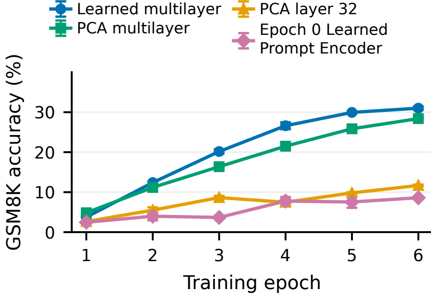
Figure 2: Representation and conditioning affect reasoning. CEDR-B learning curves on GSM8K, with 32 steps and t = \tau^2 . The first three variants retain Qwen conditioning; the fourth jointly trains a randomly initialized prompt encoder. Protocol: Appendix C.4; values and SDs: Table 12 (Appendix C.4).
