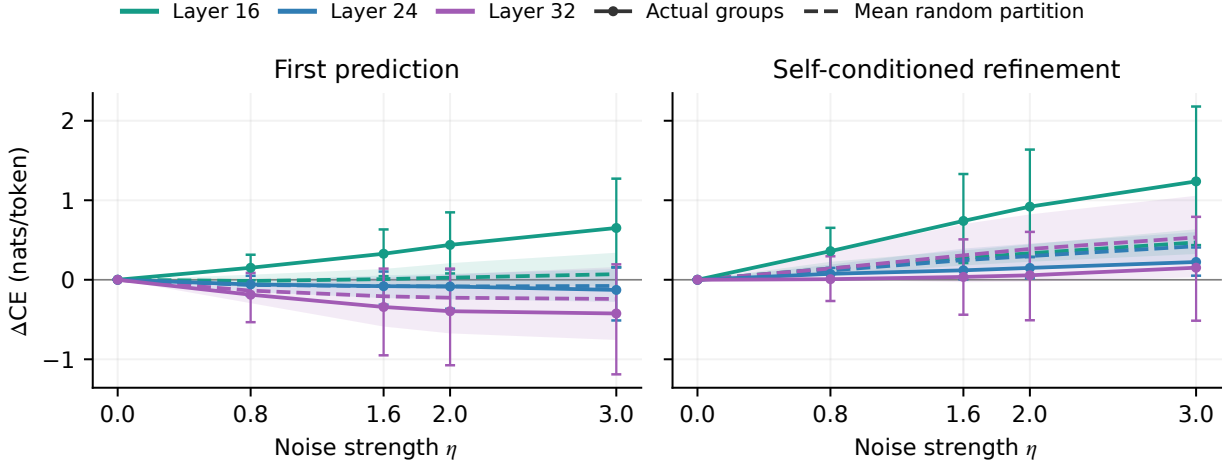
Figure 7: Layer groups expose distinct reconstruction sensitivities. CEDR-B epoch 18 on 64 GSM8K validation problems. Solid curves perturb actual layer groups; dashed curves average eight random partitions with matched widths, times, and injected Gaussian energy. Colors identify the corresponding layer or control slot. Decoder CE changes are relative to the same pass’s clean-input prediction: first without answer self-conditioning (left), then after one refinement on the same corrupted input (right). Bars show 95% CIs; shading is the range of random-partition means, not a confidence interval. Table 14 gives every plotted value.
