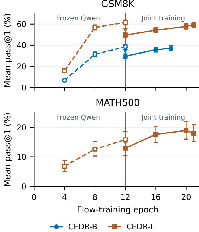
Figure 4: From teacher conditioning to learned prompts. Top: GSM8K; bottom: MATH500. Circles/squares denote CEDR-B/L; open/filled markers denote Qwen/learned prompt encoding. Red line: epoch-12 switch; arrows: immediate MSE-swap loss. Values and settings: Appendix B.3.
