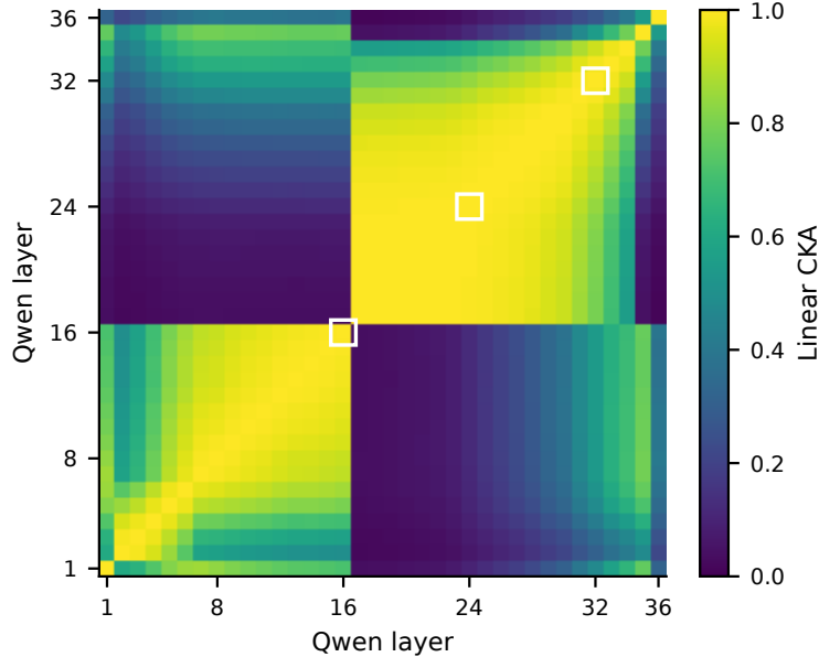
Figure 3: Qwen layer structure. Linear CKA of teacher-forced activations on the combined discovery and confirmation panels. White markers select layers 16, 24, and 32. The transition after layer 16 motivates retaining that layer, followed by regularly spaced deeper features.
