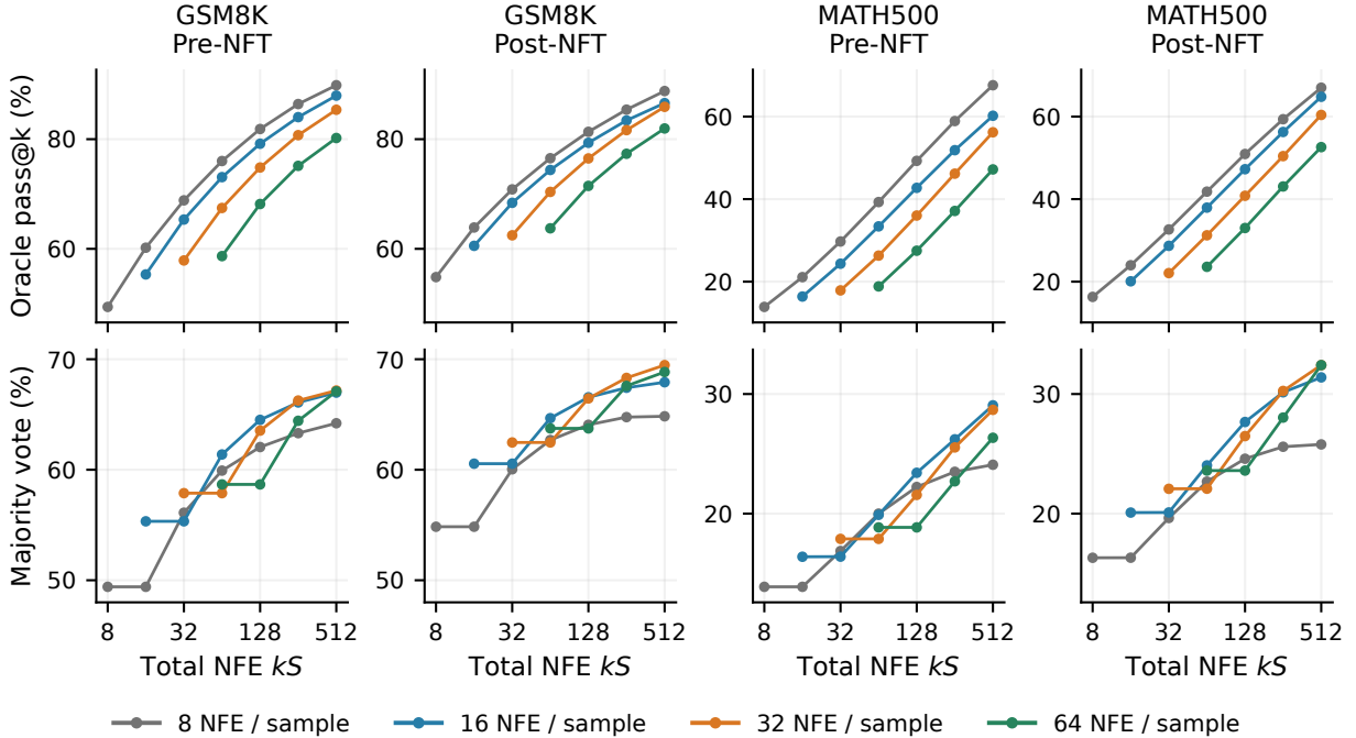
Figure 5: CEDR-L before and after NFT on GSM8K and MATH500, with SCCFG 2. Top: oracle pass@ k ; bottom: majority-vote accuracy. Colors denote denoising NFE per sample; the budget is kS . Numerical values appear in Appendix G.3; Appendix G.2 gives the corresponding CEDR-B curves.
