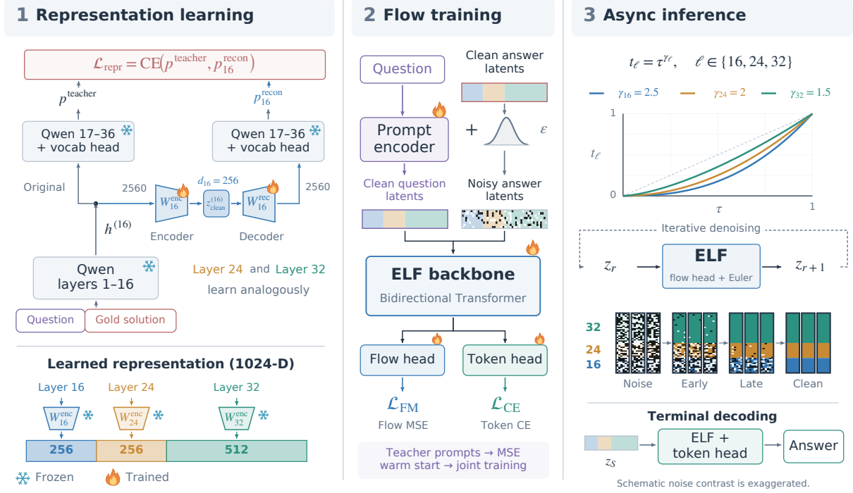
Figure 1: The CEDR training and inference pipeline. Left: Learn projections of Qwen layers 16/24/32 through teacher cross-entropy, then concatenate their outputs (Section 4.1). Center: Train the ELF backbone with flow and token-decoding losses and staged prompt learning (Sections 4 and 4.2). Right: Denoise the representation groups under asynchronous clocks, then decode the answer in parallel (Section 4.3).
