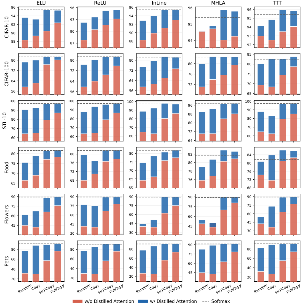
Figure B: Extended comparison results across linear operators at Tiny size. Each linear ViT is initialized under four weight-initialization settings: Random , Copy , MLPCopy , and FullCopy ; each w/ and w/o attention distillation. Results are reported with the Top-1 Accuracy (%) for all five linear ViTs (columns) on the six transfer datasets (rows) at Tiny size. In each panel, the red bar is the accuracy of the copy setting alone, the blue block is the additional gain from attention distillation, and the dashed line is the fine-tuned Softmax target.
