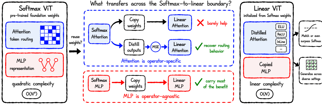
Figure 1: What survives the Softmax-to-linear boundary? We ask whether linear ViTs can benefit from pre-trained Softmax weights for initialization. We find that the attention weights are operator-specific that copying them barely helps. Their token routing behavior can instead be recovered by distilling the attention outputs, while the operator-agnostic MLP weights, which carry the learned representation, can be simply transferred by direct copying. Paired together, linear ViTs can match and even surpass the Softmax ones, consistently across diverse settings.
