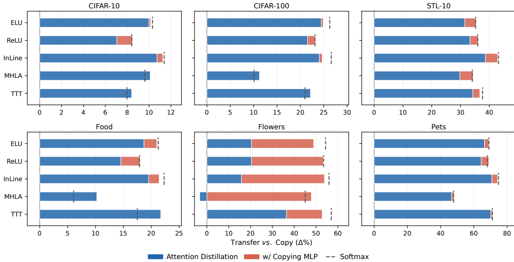
Figure 3: Distillation rescues attention-only copying. For each linear operator with ViT-Small, we report the accuracy gain over Copy : blue bars show the gain from distilling the attention on top of Copy , and red bars are the additional gain from further copying the MLP weights ( FullCopy ), leading the full setting to correspond to FullCopy w/ Distill . The dashed line marks the corresponding Softmax recovery target. Distillation effectively recovers most of the gap across linear operators on most datasets; further combining the copied MLPs can even reach the Softmax target.
