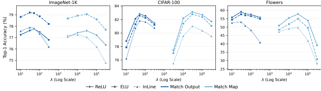
Figure 5: Loss ablation on matching attention outputs vs. attention maps. For Copy -initialized ViT-Small students, we compare MSE matching on attention outputs and attention maps with varying \lambda separately across datasets of different scales. Both matching targets show consistent accuracy trends under the \lambda -sweep. For ReLU and ELU, whose maps are proper distributions, the calibrated peaks are comparable. In contrast, for InLine, whose map is signed, map matching falls behind, suggesting that attention output matching is a more general and proper design.
