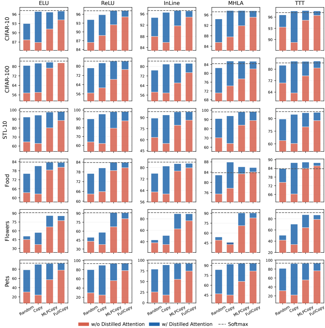
Figure A: Extended comparison results across linear operators at Small size. Each linear ViT is initialized under four weight-initialization settings: Random , Copy , MLPCopy , and FullCopy ; each w/ and w/o attention distillation. Results are reported with the Top-1 Accuracy (%) for all five linear ViTs (columns) on the six transfer datasets (rows) at Small size. In each panel, the red bar is the accuracy of the copy setting alone, the blue block is the additional gain from attention distillation, and the dashed line is the fine-tuned Softmax target.
