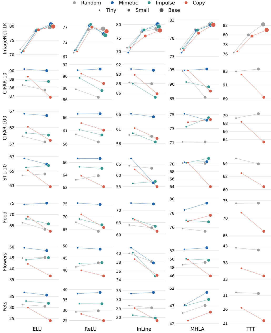
Figure 2: Attention-only Softmax-to-linear transfer barely helps. We begin by evaluating the attention-only initializations across five linear ViTs (columns) and seven datasets (rows). We report the Top-1 Accuracy (%); marker size denotes the model size (Tiny/Small/Base), and lines denote the same initialization across sizes. Across all operators, datasets, and sizes, Copy never stands out as the strongest attention-only initialization and remains at or near the Random -initialization tier.
