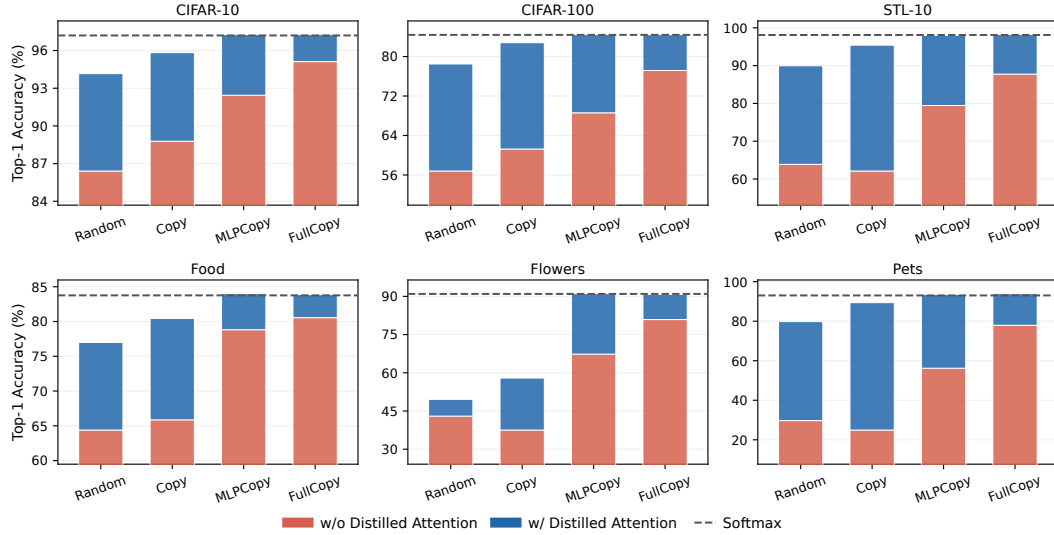
Figure 4: MLP weights survive Softmax-to-linear transfer. We selectively initialize the ReLU-based linear ViT-Small by copying from the pre-trained Softmax weights at the component level, yielding four weight-initialization settings: Random , Copy , MLPCopy , and FullCopy . For each, we report its plain accuracy and the accuracy with the distilled attention ( w/ Distill ). Red bars denote the accuracy of each initialization alone, and blue bars show the additional gain from the distilled attention. The dashed line marks the corresponding Softmax recovery target. Copying MLPs can already effectively carry most of the benefit of the pre-trained weights, while distilling the attention can lift every one of them and bring MLPCopy and FullCopy to match the Softmax level.
