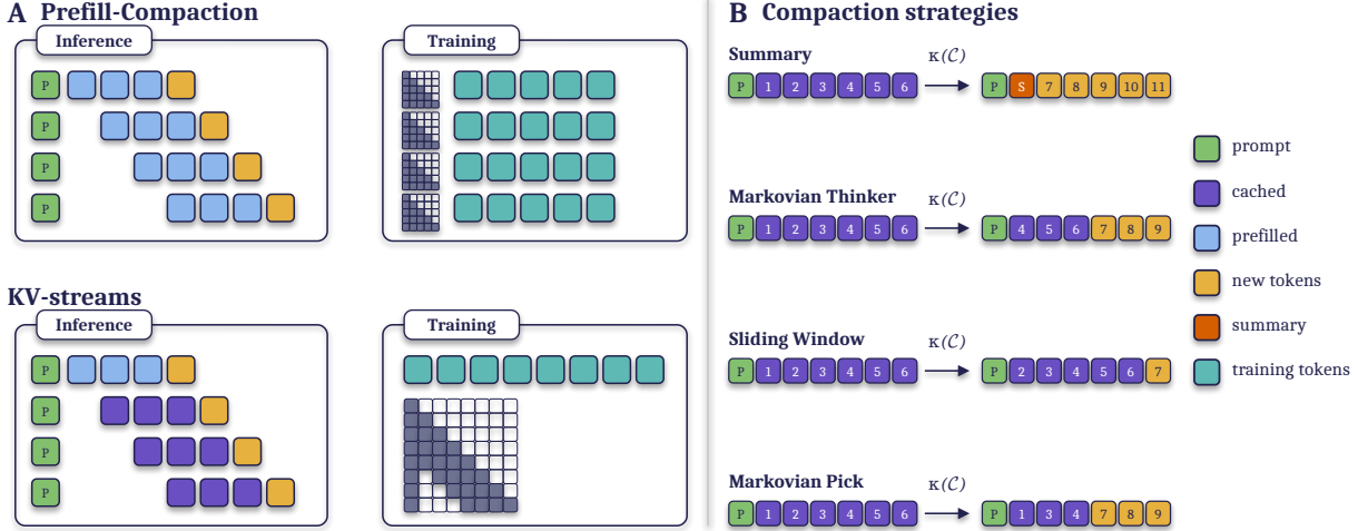
Figure 2: Compaction strategies and their training costs. (A) re-prefill compaction recomputes retained tokens and creates separate training traces. KV-streams preserves retained KV pairs and trains on a continuous trace with an attention mask that reproduces eviction. (B) context transformations under each strategy (P: prompt; S: summary).
