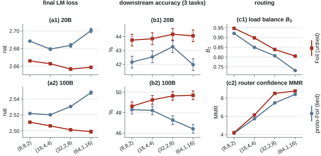
Figure 4: Tied versus untied attention at equal shape: loss (a), downstream accuracy (b) and routing (c). Horizontal axis: flattening steps from (8, 8, 2) to (64, 1, 16); each step to the right doubles E and L and halves D . Red squares: untied attention (Base and Foil-3, -2, -1); grey-blue circles: tied attention (Base-tied and proto-Foil-3, -2, -1). (a1, a2) Final loss at 20B and 100B tokens; error bars are twice the standard error of the paired difference from the (8, 8, 2) model of the same line. (b1, b2) Mean zero-shot accuracy over the three representative tasks, \pm 1 standard error. (c1, c2) Load balance B_2 and routing confidence MMR of the recurrent core at 20B tokens, from a single-seed probe without error bars; since both depend on E , only the two points at the same shape are compared. With tied attention the loss rises again after the first flattening step, while with untied attention it levels off at 20B and keeps falling at 100B; the gap is largest for the most flattened pair (0.049 nat at 100B). At every shape the untied model is both more balanced and more confident.
