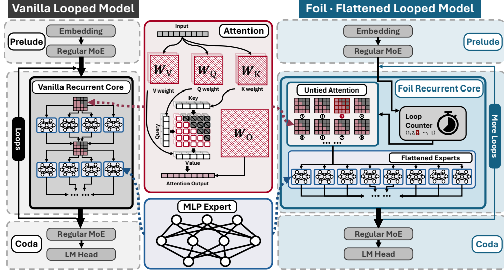
Figure 2: Vanilla looped MoE versus Foil . Both models share the same skeleton: a prelude (embedding and one regular MoE layer), a recurrent core applied for several passes, and a coda (one regular MoE layer and the LM head). The vanilla core ties both attention and experts across passes. Foil flattens the core—it keeps the total number of experts fixed while using fewer layers, more experts per layer and more passes—and unties the attention: the experts are shared across passes, but every pass has its own attention set, selected by the pass index. Both models call the same number of experts per token. When the core has several layers, every layer carries one attention set per pass; the ellipsis marks the remaining sets. Red: attention; blue: experts.
