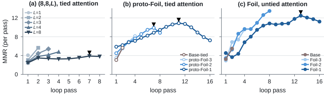
Figure 5: Routing confidence (MMR) per loop pass at 20B tokens (geometric mean over the core layers). (a) At fixed (E, D) = (8, 8) , more passes lower the confidence of every pass, and beyond L = 2 the model-level MMR falls from 4.15 to 3.36; (8, 8, 8) peaks at pass 7. (b, c) Along the flattening sequence, confidence generally rises over the passes; proto-Foil-2, proto-Foil-1 and Foil-1 reach a peak (black triangles) and then fall, whereas Foil-2, the Foil with the lowest loss at 20B, has no peak. After a peak, further flattening or more passes very likely gain least (Section 4.4).
