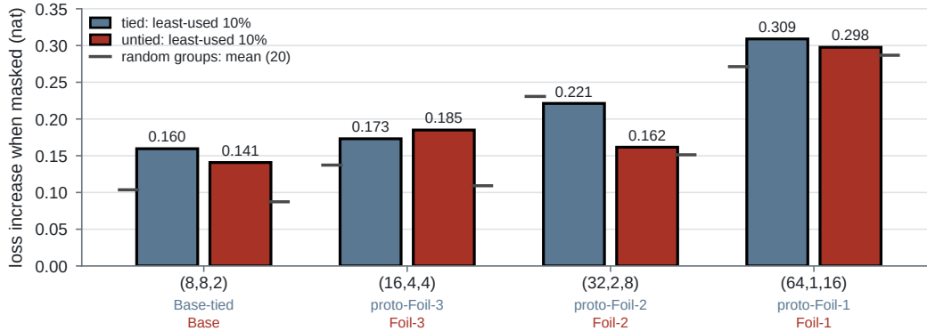
Figure 6: Masking the least-used experts at the 10% traffic tier, 20B tokens. For each shape, the left bar is the tied-attention model and the right bar the untied-attention model; bar height is the loss increase from masking the least-used group and the short dark dash beside it the mean loss increase of the 20 traffic-matched random groups. The ranges of the random groups are given in Table 12, the ratios to the random mean in Table 13.
