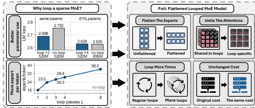
Figure 1: Motivation of designing Foil. Left: why loop a sparse MoE. (1) At equal parameters, looping lowers the loss, and matches non-looped models with much less parameters; (2) Tokens reaches more distinct experts the more passes it makes. Right: Foil’s design. (1) Flattens the experts, (2) Unties the attention. (3) Loops more times, (4) Keep parameters and compute unchanged.
