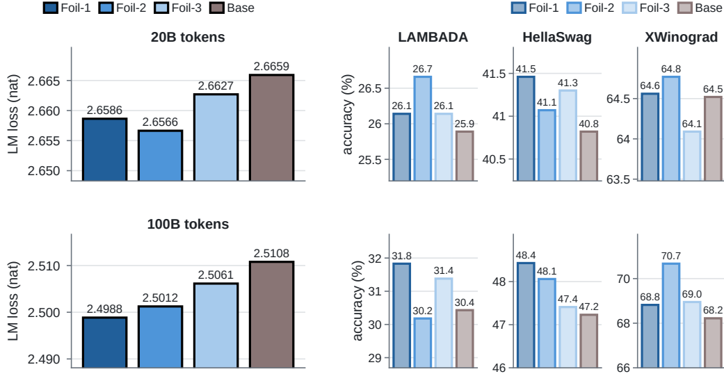
Figure 3: Flattening with untied attention: loss and downstream accuracy of the Foils and Base. Top row: 20B tokens; bottom row: after continued training to 100B tokens. In each row, solid bars on the left show the final loss (lower is better) and tinted bars on the right the zero-shot accuracy on the three representative tasks (higher is better), each panel with its own vertical axis; bars from left to right: Foil-1, Foil-2, Foil-3, Base. At 20B all three Foils are below Base ; at 100B the loss falls monotonically with flattening and Foil-1 ends 0.012 nat below Base. Downstream accuracy is on par or slightly better; further tasks are in Appendix E.
