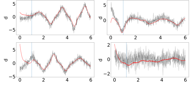
Fig. 5. (Coupled nonlinear oscillator) Test-set rollouts from Eq. (3) for the predicted disturbance as functions of time. Black: disturbance proxy y(t) ; red: rollout prediction \hat{d}(t) . The proxy y is visibly noisier, while \hat{d} is smooth. Mean squared error is 2.54 overall and 0.88 after discarding the first second of each trajectory as a burn-in period (vertical dashed line).
