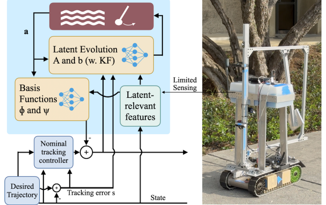
Fig. 1. Proposed adaptive control architecture and experimental platform. Left: block diagram of the controller. A latent state is estimated online via a Kalman–Bucy-style filter from the disturbance proxy y , using a latent-state evolution model parameterized by (A, b) . The basis functions (\Phi, \psi) map latent-relevant features \phi to an adaptive disturbance-rejection term that augments a nominal tracking controller. The quantities (A, b, \Phi, \psi) are parameterized by neural networks and learned using a statistically principled training procedure. Right: tracked mobile robot used for experimental validation.
