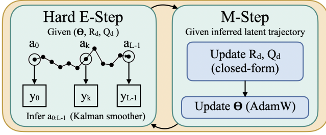
Fig. 2. Statistically principled training via hard-EM with exact latent inference. The procedure alternates between a hard E-step and an M-step: given current parameters (\theta, R_d, Q_d) , the hard E-step infers the latent trajectory \mathbf{a}_{0:L-1} for each data window, and the M-step updates the noise covariances (R_d, Q_d) from residual statistics and updates the network parameters \theta .
