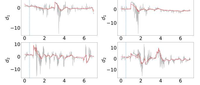
Fig. 3. (Tracked vehicle) Test-set rollouts for the predicted disturbance \hat{d} \in \mathbb{R}^2 as functions of time, on two different test-set trajectories. Black: disturbance proxy y(t) ; red: rollout prediction \hat{d}(t) . The proxy y is visibly noisier. The average prediction MSE was 3.53; it was 3.49 after discarding the initial half second for each trajectory as a burn-in period (vertical dashed line).
