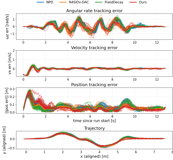
Fig. 4. (Tracked vehicle) Tracking runs under four controllers.
