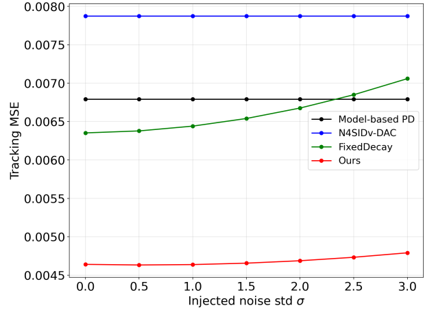
Fig. 6. (Coupled nonlinear oscillator) Robustness sweep for tracking control under additional Gaussian noise injected into the sparsely provided disturbance proxy y (averaged over 30 reference trajectories, with each trajectory being 20 seconds long). Mean tracking MSE is plotted versus the added noise level \sigma , where \sigma = 0 denotes the baseline noise setting. The proposed dynamical-representation controller performs the best. As \sigma increases, the neural adaptive controllers degrade because the disturbance proxy becomes increasingly corrupted. The simpler N4SIDv-DAC baseline resulted in a flat graph because the fitted discrete-time A , B_1 , and B_2 satisfied \|A\| \approx 0.09 \ll 1 , \|B_1\| \approx 0.08 \ll 1 , \|B_2\| \approx 0.005 \ll 1 and hence the disturbance compensation mostly came from \hat{d} \approx D_1 \phi + D_2 u .
