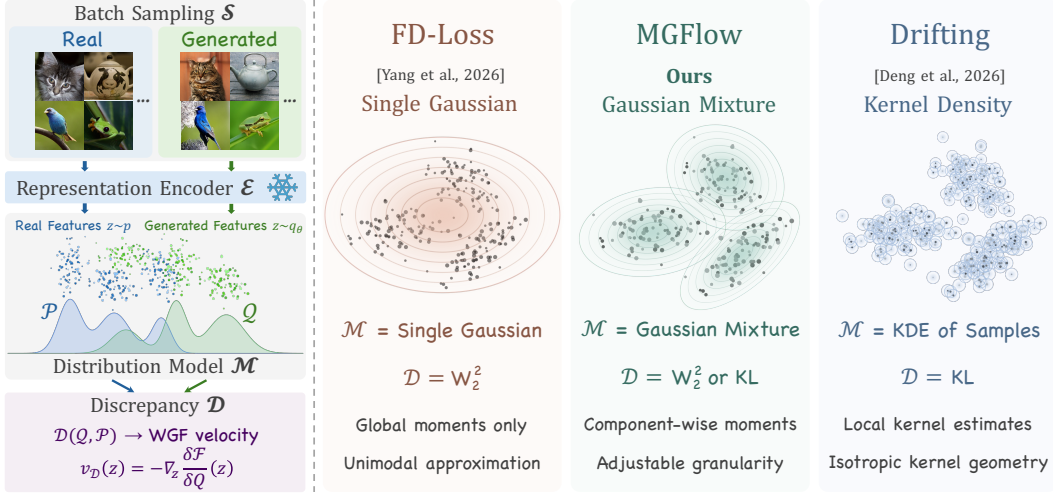
Figure 2: A unified view of distributional training. Left: sampling \mathcal{S} , encoding \mathcal{E} , distribution modeling \mathcal{M} , and matching discrepancy \mathcal{D} define the paradigm. Right: FD-Loss, MGFlow, and Gaussian-kernel Drifting use Gaussian, GM, and KDE representations, respectively. Their matching objectives induce feature-space velocity fields through the Wasserstein gradient flow of their respective distributional objectives.
