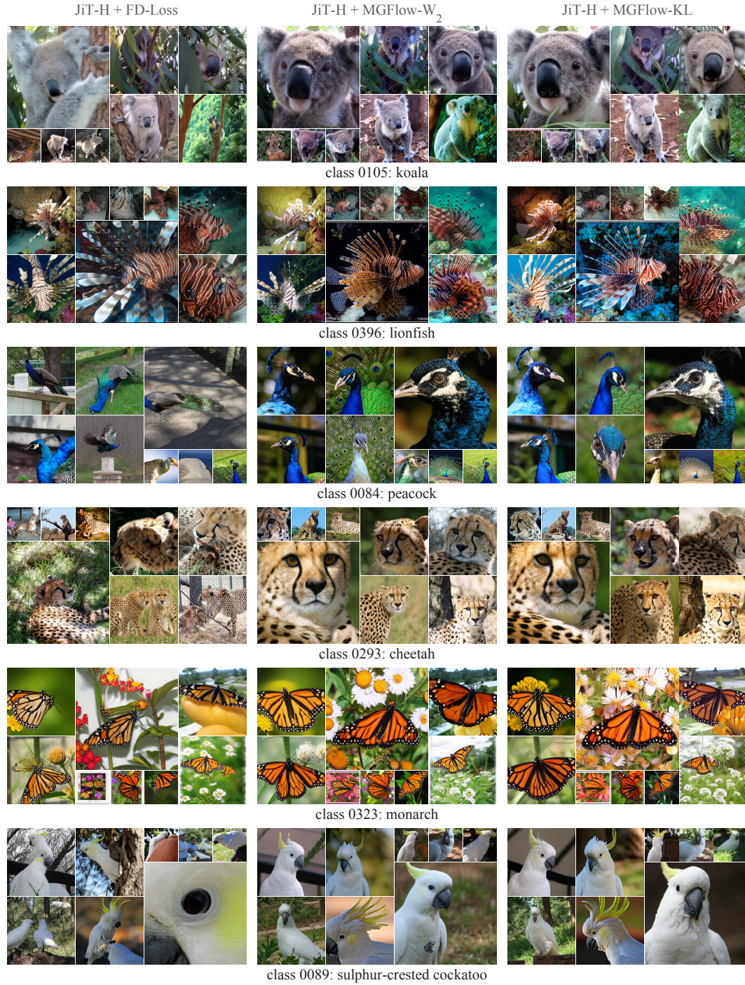
Figure 6: Additional uncurated ImageNet 256 \times 256 samples from JiT-H. FD-Loss (left), MGFlow- W_2 (middle), and MGFlow-KL (right), all with one NFE. Corresponding images use identical input noise.
