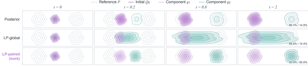
Figure 3: Toy experiment with component assignment and transport. Score matching with K = 2 moves 2048 particles. Dashed contours show the reference P . Shading and contour counts indicate weights. LP fixes component weights, but global velocity collapses modes. Only LP-paired achieves correct transport.
