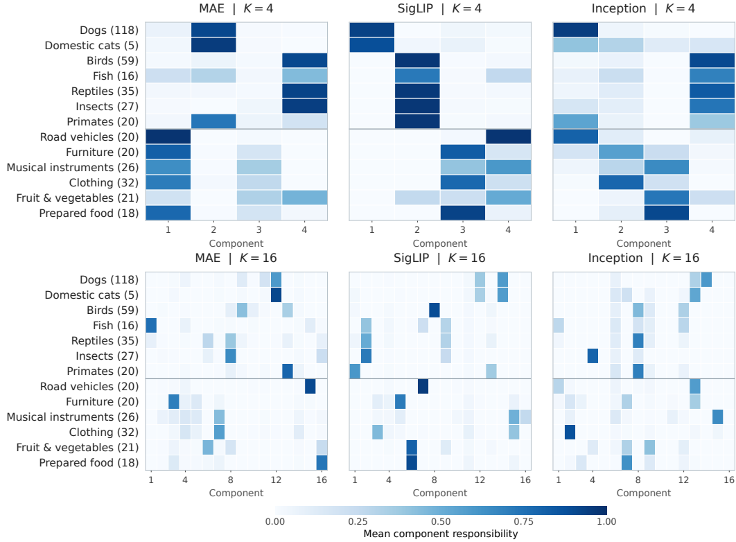
Figure 4: Semantic groups across independently fitted mixtures. Rows show mean posterior responsibilities for 13 label-defined groups covering 417 ImageNet classes, using 200 images per class. We average r_{ck} equally over the classes in each group; parentheses give the number of classes. Component indices are local to each GM, not aligned across panels.
