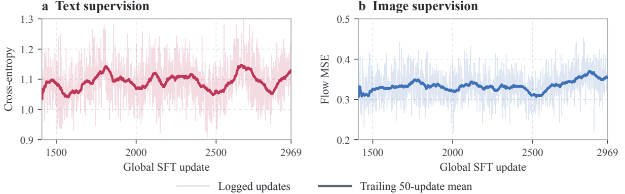
Figure 6 The supervised parent, recorded continuation phase. Text cross-entropy and image flow-MSE from global SFT updates 1410–2969. Faint lines show logged update values and solid lines show trailing 50-update means.
