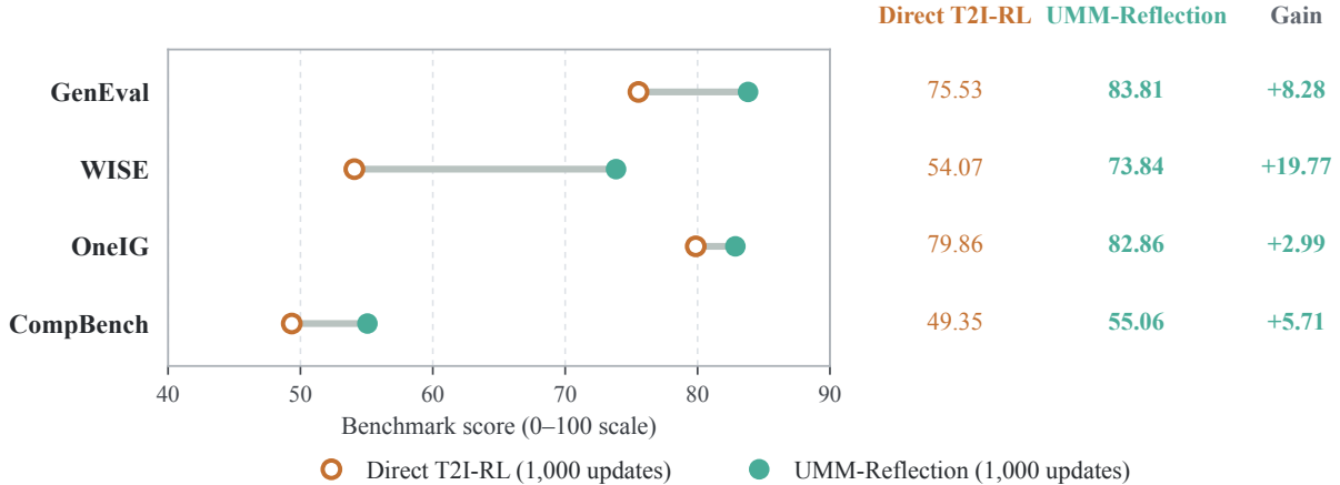
Figure 7 Completed direct-T2I RL control. Hollow orange points denote direct T2I-RL at 1,000 updates; green points denote UMM-Reflection at 1,000 updates. Gain is the within-benchmark score difference. Each benchmark keeps its own metric on a 0–100 scale; scores are not averaged across benchmarks. The systems differ in initialization and training/inference compute (Appendix A).
