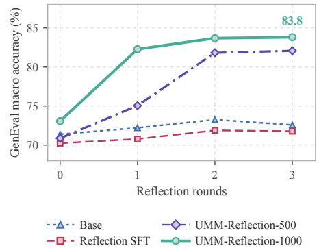
Figure 4 Test-time scaling on GenEval. Macro accuracy versus reflection rounds. Other benchmarks: Appendix Figure 9.
