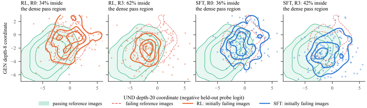
Figure 5 Image trajectories in the backbone’s own correctness readout. Each point is one initially failing image, placed by two held-out linear probes for “passes the verifier”: the understanding stream at depth 20 ( x ) and the generation stream at depth 8 ( y ), the depths where each stream’s probe AUC peaks. Green filled contours mark verifier-passing reference images and red dashed contours verifier-failing ones; orange and blue contours summarize the RL and SFT images. Read the panels in pairs, from R0 to R3 for the same policy: RL (left pair) and SFT (right pair). Percentages are the share inside the dense pass region (Table 5).
