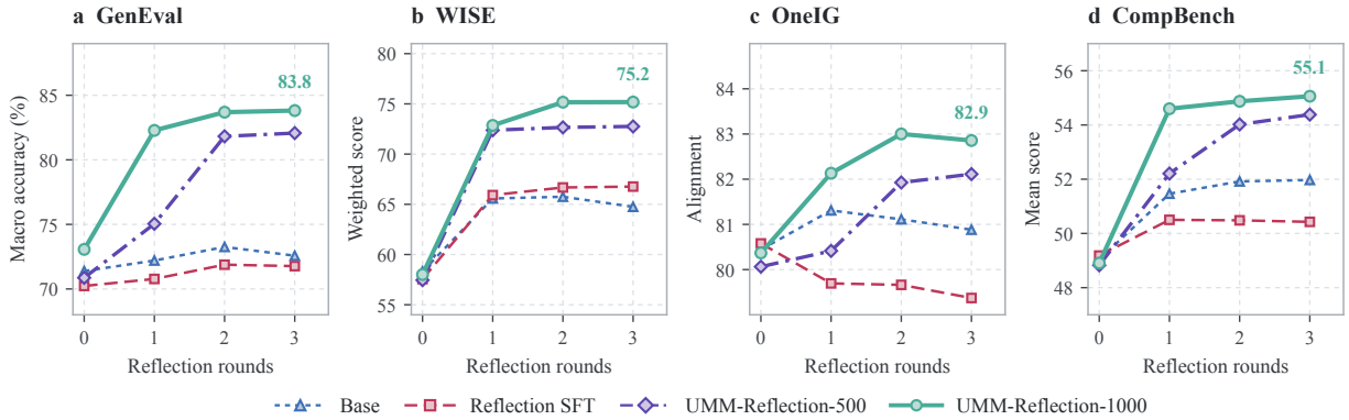
Figure 9 Multi-round test-time scaling on four benchmarks. Scores (0–100) versus reflection rounds. Blue dotted lines denote Base, pink dashed lines reflection SFT, purple dash-dotted lines UMM-Reflection-500, and green solid lines UMM-Reflection-1000.
