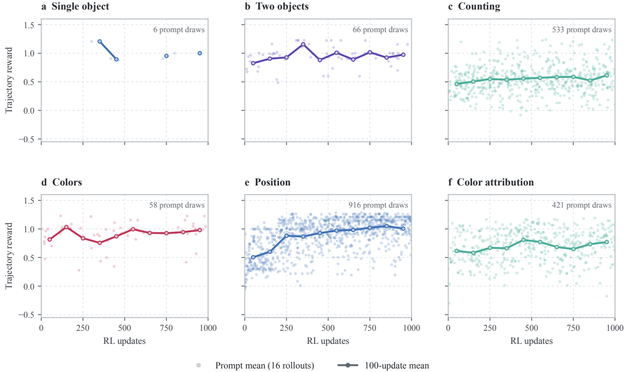
Figure 20 Training reward by GenEval family. Light points are the mean whole-trajectory reward of the 16 rollouts for one prompt; lines are 100-update means. Prompt draws per family follow the training pool composition; single object has six draws and its line is left open.
