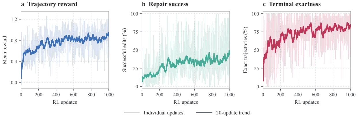
Figure 8 Learning dynamics of the 1,000-update RL run. (a) Mean trajectory reward. (b) Successful repairs per edit from an incorrect state. (c) Fraction of trajectories reaching terminal exactness under the training verifier. Faint lines are individual updates; solid lines are trailing 20-update trends, with rates pooling numerators and denominators over the window.
