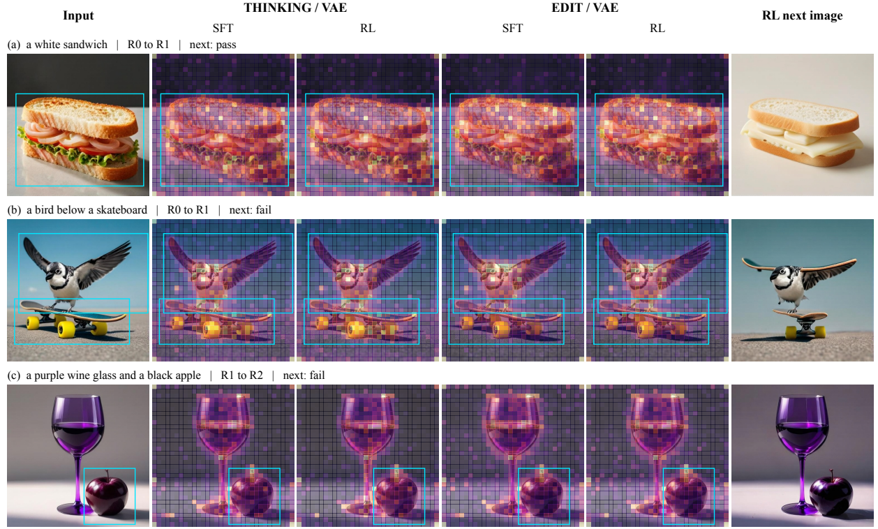
Figure 10 Attention over VAE image tokens is preserved after RL. Three cases show paired SFT/RL attention of THINKING and EDIT tokens onto 32 \times 32 VAE keys, averaged over 28 layers. Maps use a shared 99th-percentile cap; cyan boxes are pre-annotated error regions.
