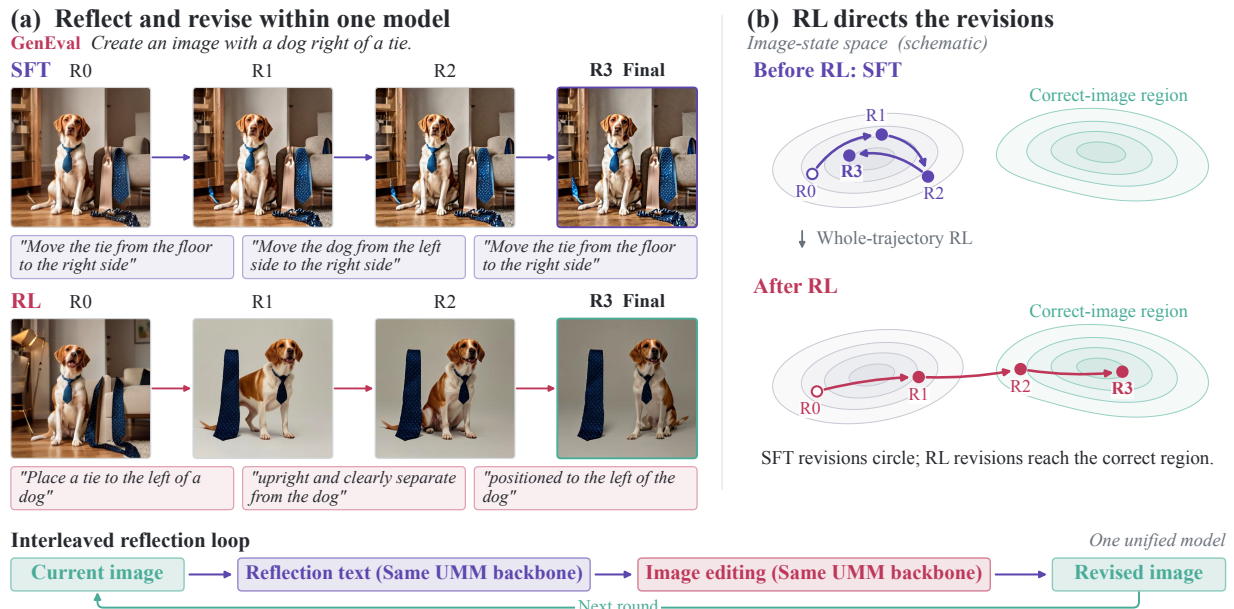
Figure 1 Native reflection before and after RL. Left: SFT and RL on the same prompt and seed. SFT already produces meaningful revisions (16 SFT rollouts contain a correct repair for 78% of failing training images; Appendix I), but one trajectory often circles, as here (tie, dog, tie). RL concentrates the policy on revisions that reach the correct region (right; measured in Figure 5).
