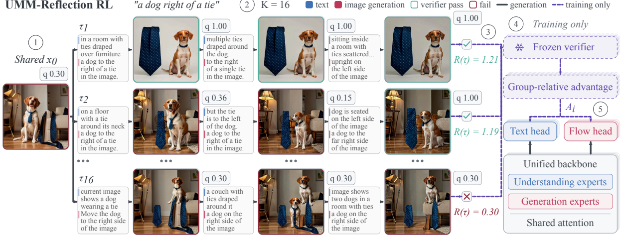
Figure 2 UMM-Reflection RL. (1) K=16 rollouts share one detached initial image x_0 . (2) Each interleaves the model’s own reflection (verbatim) with its renders for up to three rounds. (3) A frozen verifier scores every image ( q ) and trajectory ( R(\tau) ). (4) Group normalization gives one advantage A_i per trajectory, (5) which updates both the text and flow heads. Green/red frames: verifier pass/fail; dashed: training only.
