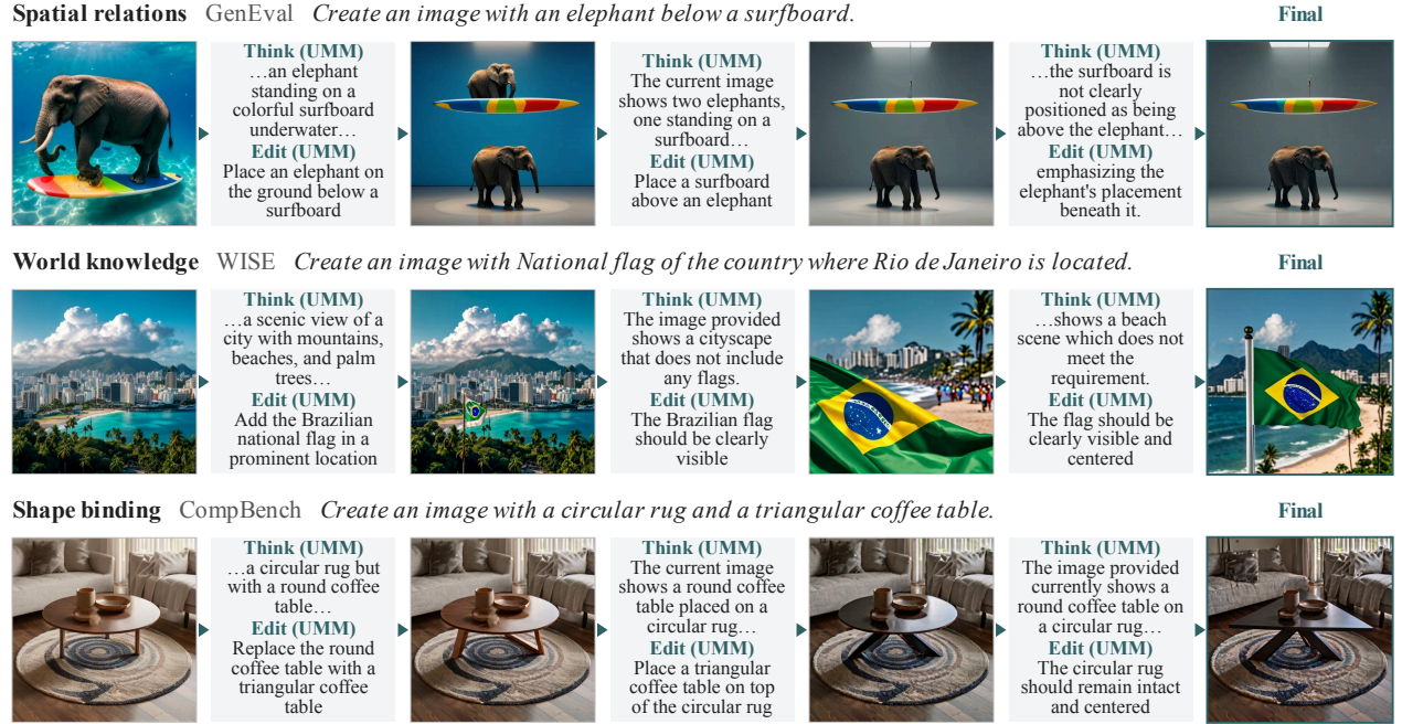
Figure 12 Reflection trajectories of UMM-Reflection. Examples from GenEval, WISE, and CompBench show how step-by-step reflection and revision help the model produce images that match the prompt. Each row reads left to right: the image, then the unified model’s own reflection on it ( Think : what is wrong; Edit : the instruction it issues), then the image it renders from that instruction. All text is verbatim model output.
