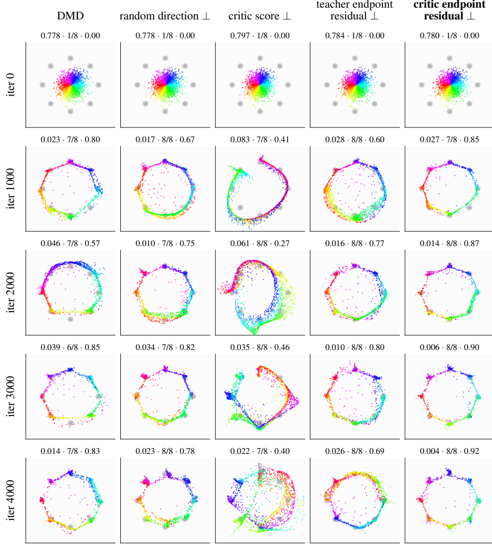
Figure B2: Generated samples of the five 2D variants over training. Columns are the five variants of Section B.1. Rows are iterations 0, 1,000, . . . , 4,000 of the same runs as Figure 4. Point color encodes the angle of the latent z , visualizing how latent directions map to target modes. Each panel lists the energy distance ( \downarrow , lower is better), the number of covered modes ( \uparrow ), and the on-mode fraction ( \uparrow , higher is better) at the shown iteration. The student–critic-endpoint-residual column (PDMD) covers all eight modes from iteration 2,000 onward and stays tight. The critic-score column covers the modes but does not concentrate. The teacher-residual column shows the instability near iteration 3,000.
