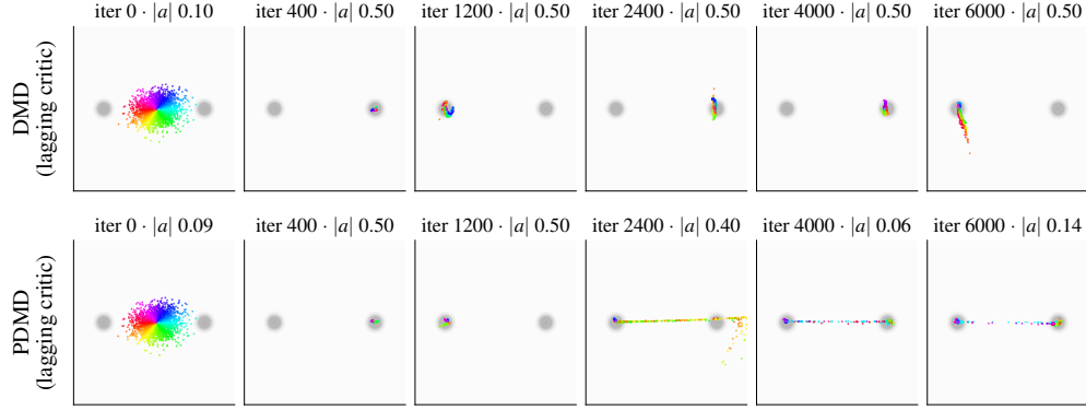
Figure B3: Two-mode collapse process under a lagging critic (seed 0). Rows are plain DMD and PDMD; columns are training iterations. Each panel lists the iteration and the imbalance |a| ; |a| = 0 is the balanced solution and |a| = 0.5 is full collapse. Both variants start from a collapsed transient at iteration 400. Plain DMD stays locked on one mode for all 6,000 iterations. PDMD transports mass back between the modes (iteration 2,400 shows samples in transit) and settles near balance. The main text shows the collapsed DMD endpoint in Figure 5.
