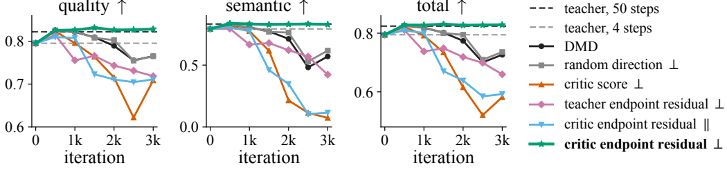
Figure 10: Quantitative ablation study: training dynamics of MiniMax-H3 on VideoGen-Eval. PDMD holds its total score; the others decline.
