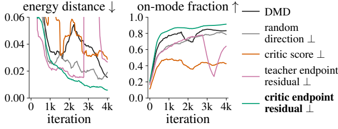
Figure 4: 2D comparison of projection directions (20-point moving average). Left: energy distance to the target. Right: fraction of samples within 3\sigma of a mode center. Among the tested directions, only the PDMD projection stabilizes training and improves both metrics over DMD.
