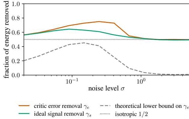
Figure B1: Direct measurement of the removal ratios on the ring of eight. Along the PDMD run of Section B.1: the fraction of critic-error energy \gamma_e and of ideal-signal energy \gamma_s that the projection removes, against the noise level. The grey dashed line is the theoretical lower bound \|e\|^2/(\|e\|^2 + \text{tr } \Sigma(q)) of Equation (10) on \gamma_e . Each curve is a mean over the snapshots from iteration 100 to 4,000. The dotted line marks the mean energy fraction 1/2 removed by a uniformly random rank-one deletion from a fixed vector in the plane.
