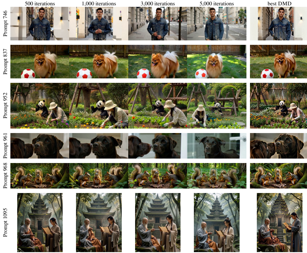
Figure D4: PDMD with a 1.25\times larger student step also does not degrade over 5,000 iterations. The first four columns are checkpoints of the single PDMD run of Section D.4 . The last column, set slightly apart, is the best DMD checkpoint over a learning-rate search, the DMD † row of Table 2 . Rows are labelled with the VideoGen-Eval prompt id; every panel is the frame at 80% of the clip, with the same prompt, seed and sampler throughout.
