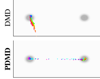
Figure 5: Two-mode distillation with lagging critic . This run illustrates DMD collapse (top) and PDMD coverage of both modes (bottom).
