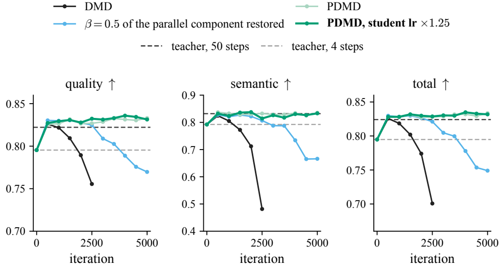
Figure D3: A larger student step and a partial projection on MiniMax-H3 at 4 NFE. Quality, semantic, and total scores of every 500-iteration checkpoint up to 5,000 iterations on the 387 VideoGen-Eval prompts. DMD is the corresponding variant in Figure 10. The light green curve shows PDMD at the base learning rate, as far as it was scored, and the dark green curve shows PDMD trained with a 1.25\times larger student learning rate (Section D.4). The blue curve shows the run that restores half of the residual-parallel component removed by PDMD, using Equation (D1) with \beta = 0.5 (Section D.3). Iteration 0 is the undistilled base model at 4 NFE. Horizontal lines show the teacher scores at 50 and 4 sampling steps.
