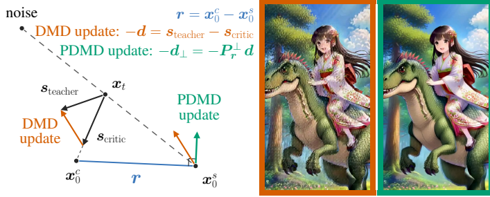
Figure 3: DMD and PDMD updates. DMD moves the student along -d . The critic score s_{\text{critic}} , the online-learning part of d , carries hidden error. PDMD projects out the component of d parallel to the known residual r to suppress critic error, because r is the critic error estimate. The two frames decode one real update target: the PDMD target contains fewer artifacts than the DMD target , while keeping 83% of the update norm.
