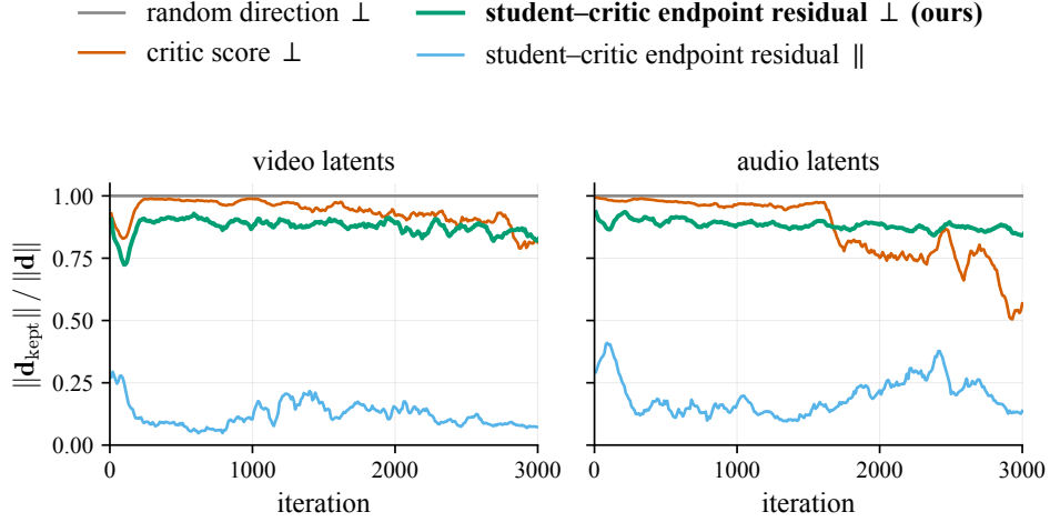
Figure D2: Retained fraction of the DMD update norm on MiniMax-H3 at 4 NFE. d_{\text{kept}} is the component the variant keeps, as a 100-iteration running mean. Left: video latents. Right: audio latents.
