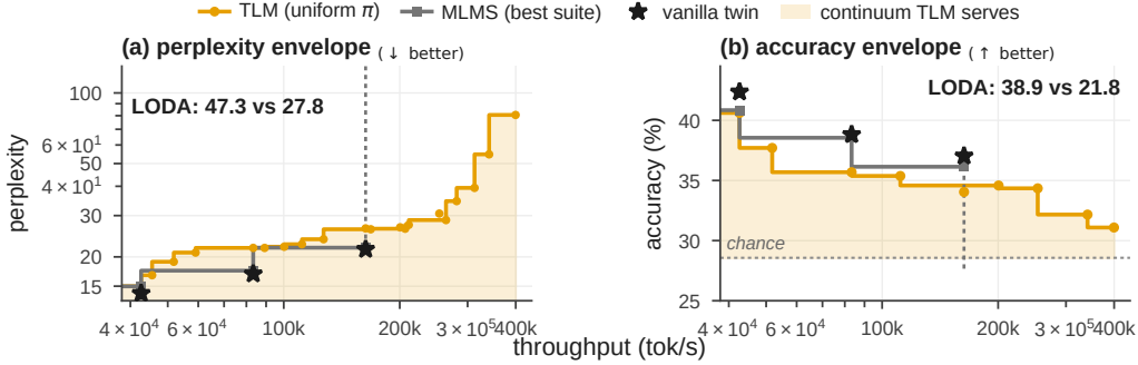
Figure 3: One TLM is a continuum of models; suites and vanilla training yield isolated points. Each marker is an operating point the method actually trains. TLM-uniform (amber) serves every prefix throughput in the range; the shaded band is the continuum it delivers. MLMS (grey squares) and vanilla twins (stars) exist only at their training sizes; MLMS’s exits edge TLM’s prefixes at k=11, 16 (the price of coverage) and it collapses off-exit (dashes). Envelopes give the best quality served at each throughput (log scale; faster rightward; a faster model can always be throttled down). (a) Validation perplexity (log–log; lower is better). (b) Mean 7-benchmark accuracy (higher is better); the band above the chance floor (dotted) is exactly TLM’s \text{LODA}_{\text{acc}} . LODA (area under each envelope; perplexity uses a clamped normalised quality) is annotated per method: TLM wins on both.
