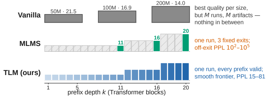
Figure 1: One training run, a valid language model at every depth. Top : vanilla LLMs train a separate standalone model per budget (our 50M/100M/200M twins, annotated with validation perplexity) — the best quality per size, but M runs, M artifacts, and nothing in between. Middle : MLMS (Godey & Artzi, 2026) nests the budgets in one 20-layer cascade but supervises only three fixed exits (green); every other prefix is untrained and collapses (hatched). Bottom : a Telescopic Language Model trains one random prefix per step against the full target, so every prefix of the same cascade is a valid language model (gradient: deeper prefixes are larger models). The result is a continuum of operating points from one run, with the full-size peak close to a separately trained twin (14.99 vs. 13.98 perplexity).
