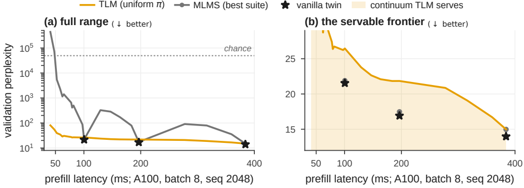
Figure 4: One run serves any latency; the suite serves three. Validation perplexity (lower is better) against measured prefill latency (one A100, batch 8, sequence 2048, bf16). (a) TLM-uniform (amber) is a valid language model at every latency, while MLMS (grey) is servable only at its three trained exits (circles) and collapses off-exit, rising to 10^2 – 10^5 PPL up to the dotted chance line. (b) Zoom on the servable range: the band is the continuum TLM serves at every latency; MLMS’s exits sit below TLM at k=11 and k=16 , its only valid points. Stars: vanilla twins.
