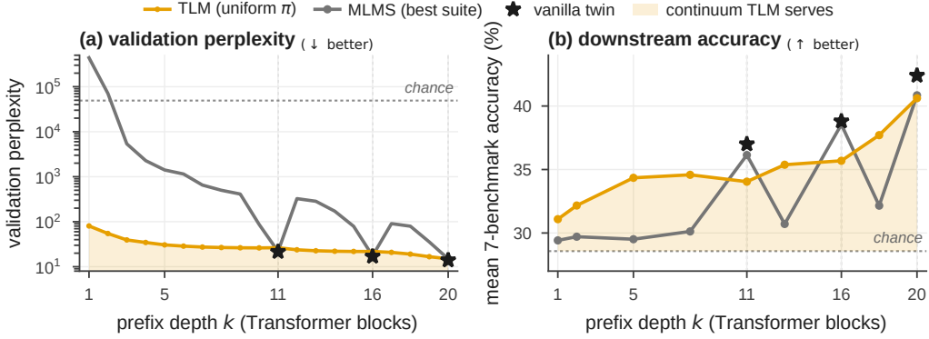
Figure 2: One training run, a valid model at every depth. TLM (amber) is a valid language model at every one of its twenty layer prefixes; the shaded band is the continuum it serves. MLMS (grey) is valid only at its three trained exits (dashed) and collapses elsewhere; at those exits it remains stronger, the price of coverage (§4.2). (a) Validation perplexity of every prefix (log scale, lower is better; dotted: chance): TLM decreases smoothly across the whole range while MLMS falls to 10^2 – 10^5 between its exits. (b) Zero-shot downstream accuracy (higher is better): TLM’s continuum improves with depth while MLMS’s off-exit prefixes sit at chance; the band is TLM’s above-chance quality at every depth. Stars: independently trained vanilla twins (the per-size ceiling). Area under the loss–budget frontier (AULB): TLM 3.28 vs. MLMS 5.73–5.90.
