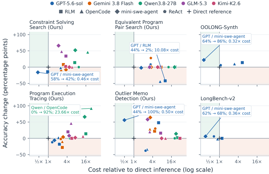
Figure 4: Harness effects relative to direct inference on OOLONG-Synth, LongBench-v2, and our suites. External benchmarks use GPT-5.6-sol. The reference is zero accuracy change and 1\times cost. Green denotes higher accuracy at lower cost; pink denotes lower accuracy at higher cost.
