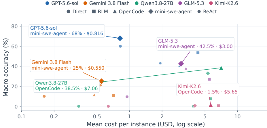
Figure 3: Macro-average accuracy and estimated cost across the four tasks (Table 2). Color denotes model; shape denotes harness. Callouts and larger markers mark each model’s best accuracy. ReAct appears where available.
