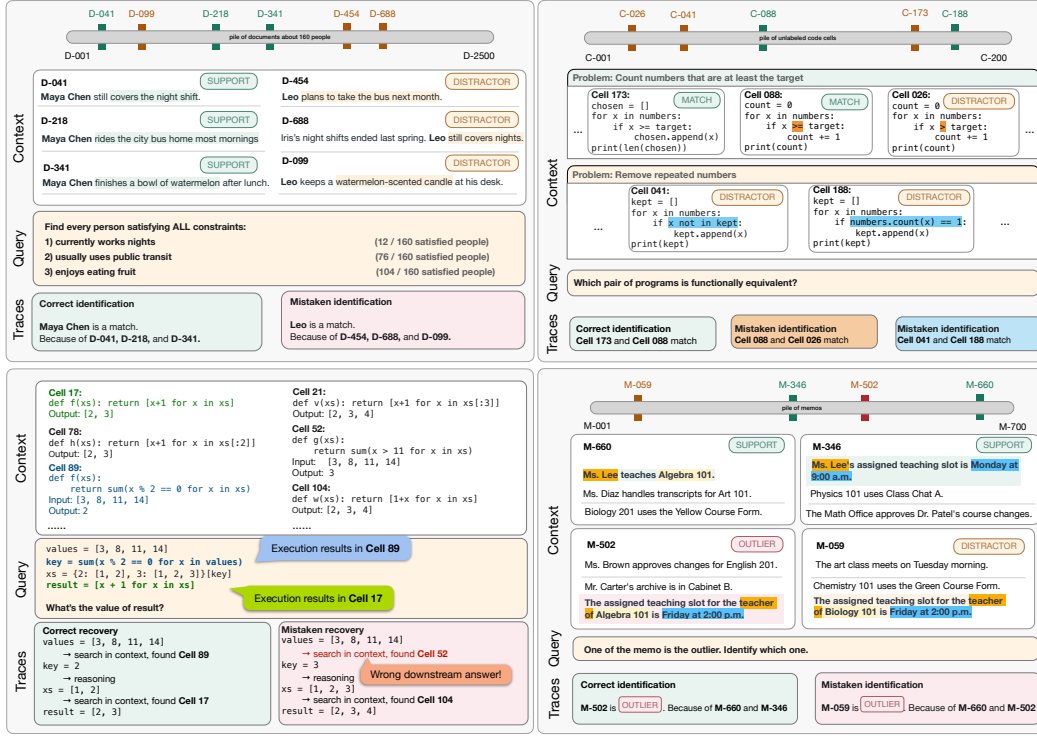
Figure 2: Examples from our benchmark. Top left: Constraint Solving Search combines evidence from documents. Top right: Equivalent Program Pair Search distinguishes equivalent programs from near matches. Bottom left: Program Execution Tracing requires reading prior outputs and matching code semantics. Bottom right: Outlier Memo Detection identifies a conflict using supporting memos.
