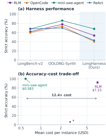
Figure 1: LONGHARNESS (ours) reveals harness differences in both accuracy and cost.
