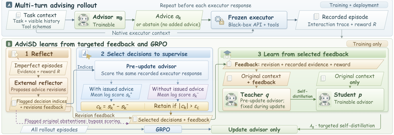
Figure 1 | Overview of ADVISD. (A) Multi-turn advising. Before each executor response, the advisor provides advice or abstains; the frozen executor uses its native context and any issued advice. (B) Training from targeted feedback. Reflection proposes corrections at advice decisions in imperfect episodes. Among flagged decisions, ADVISD retains original abstentions and those whose scores with and without issued advice differ by more than a calibrated threshold. The pre-update advisor computes both on the same recorded executor response. At retained decisions, a feedback-conditioned copy of the pre-update advisor teaches the trainable advisor, which sees only the original context. This self-distillation supplements GRPO on all episodes.
