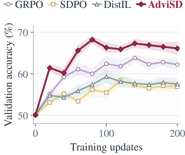
Figure 3 | Training progress on BFCL-v3. Validation accuracy across training updates with Claude Sonnet 4.6 as the frozen executor. Mean \pm sample standard deviation over three independent training runs. AdvISD stays ahead of the baselines from update 20 onward.
