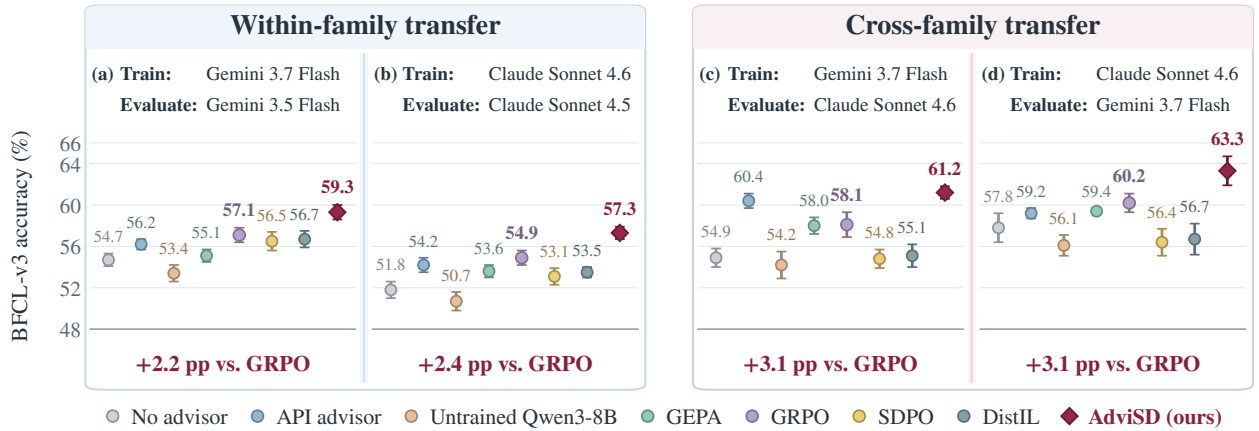
Figure 2 | Cross-version and cross-family BFCL-v3 transfer without retraining (Q3). Train/Evaluate labels identify executors; API advisors use the evaluation executor’s model. Dots show means; intervals indicate \pm sample SD. Gains show ADVISD minus GRPO in % points. All panels share a 48–66% accuracy scale.
