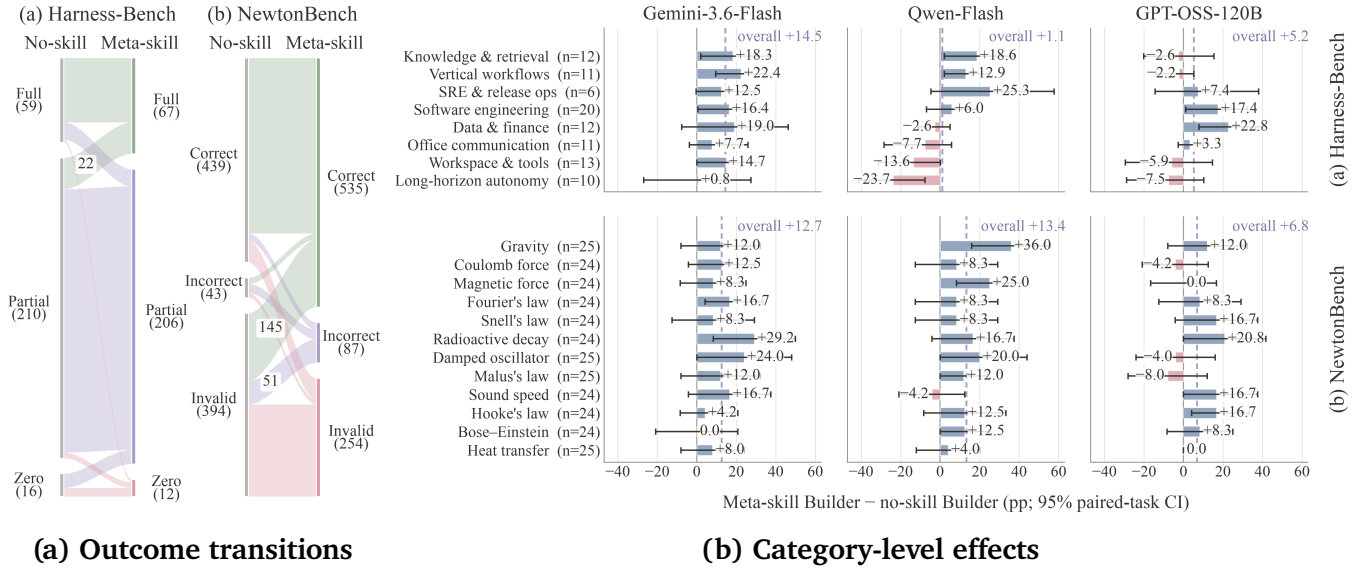
Figure 4: (a) Outcome transitions from no-skill to full-bank meta-skill Builders, aggregated over three Targets. Band widths represent paired-task counts; in-band numbers highlight the largest cross-outcome flows. “Zero” includes zero scores and construction failures; “Invalid” includes missing or unparseable submissions and construction failures. (b) Category-level effects across all six settings. Rows represent Harness-Bench task categories and NewtonBench physical mechanisms; columns represent Targets. Bars show score differences between full-bank and no-skill Builders with unadjusted 95% task-bootstrap confidence intervals. Purple dashed lines indicate setting’s overall effect.
