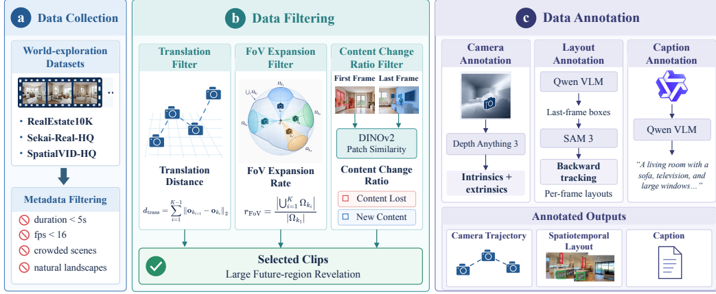
Figure 2: Data Curation Pipeline. (a) World-exploration video collection and metadata filtering. (b) Clip selection based on translation distance, FoV expansion, and content change. (c) Annotation of camera trajectories, spatiotemporal layouts, and captions.
