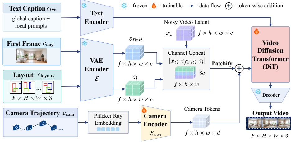
Figure 3: Model Architecture. Layout latent is channel-concatenated with the noisy video latent and first-frame latent. Camera tokens are injected into the DiT stream through token-wise addition. Color-referenced layout local prompts are appended to the global caption.
