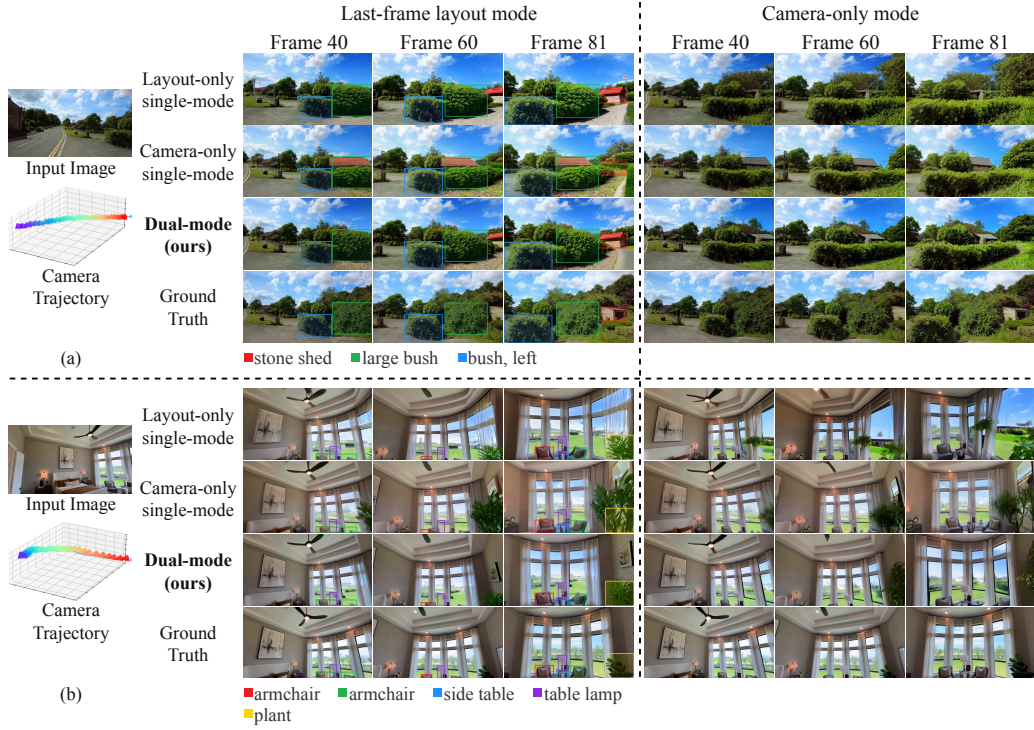
Figure 8: Dual-mode OPSD Comparison. The last-frame-layout mode uses both the camera trajectory and last-frame layout, whereas the camera-only mode uses only the camera trajectory. Last-frame-layout single-mode OPSD follows the prescribed layout, but yields lower video quality than dual-mode OPSD in camera-only inference, while camera-only single-mode OPSD preserves camera control but often fails to realize the specified future layout. In contrast, dual-mode OPSD maintains strong camera control in both inference settings while faithfully following the future-layout condition when provided.
