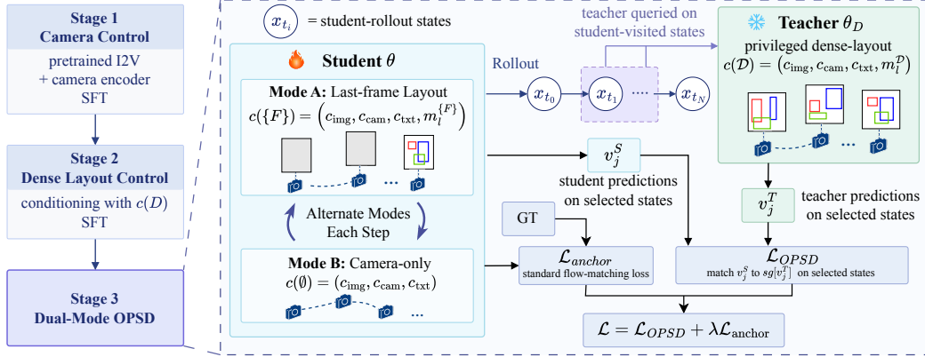
Figure 4: Dual-mode OPSD. The student alternates between last-frame-layout and camera-only modes and distills selected rollout states from a frozen dense-layout teacher with a flow-matching anchor loss. The student and teacher are both initialized from \theta_D .
