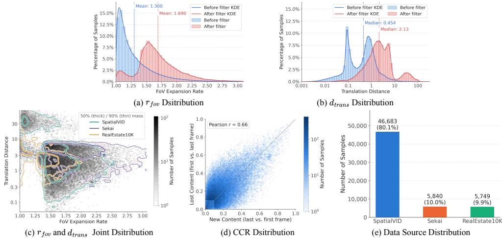
Figure 6: Visualization of data distribution. (a, b) Distributions of the camera-motion metrics over all candidate windows before filtering (blue) and over the final layout training set (red). Filtering removes the mass of near-static windows and shifts both metrics toward larger viewpoint changes. (c) Joint distribution of the two camera-motion metrics in the training set, with 50% and 90% mass contours per source dataset. (d) Joint distribution of the two content change ratios. The two directions are correlated and complementary but not redundant. (e) Number of training clips per dataset.
