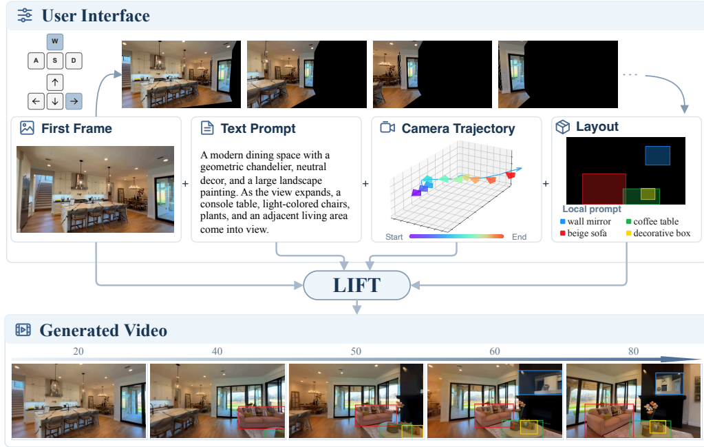
Figure 1: Given a first frame, users can navigate from the first-frame view along a desired camera path and specify layouts using bounding boxes with local text prompts in the final frame. Then, LIFT generates the intended shot that transitions from the input image to the user-defined last-frame layout following the prescribed camera trajectory.
