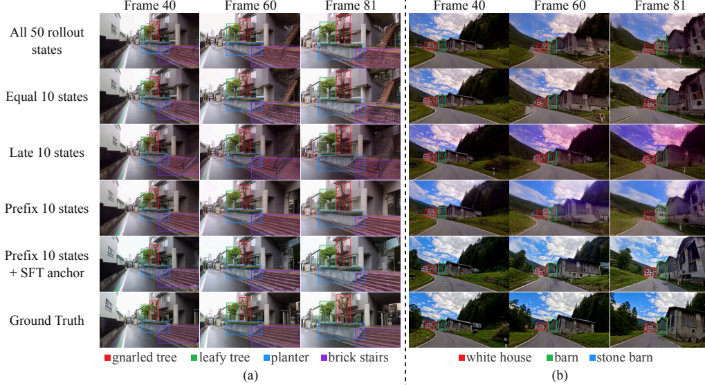
Figure 10: Comparison of different ODE state sampling in OPSD. Distilling only on the late 10 states (the third row) yields the weakest layout following, indicating that global layout structure is mainly determined during the early high-noise stage. Prefix-state distillation provides stronger layout control, while adding the SFT anchor further prevents drifting and visual-quality degradation.
