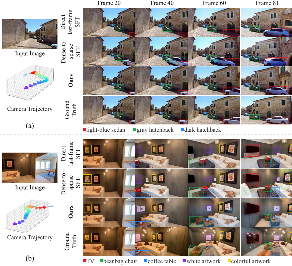
Figure 7: SFT and OPSD Comparison. (a) Direct last-frame SFT largely ignores the sparse layout condition, leaving the target sedan absent until the final frame, while dense-to-sparse SFT introduces it too early and with inaccurate spatial alignment. In contrast, OPSD produces a trajectory that better matches the ground-truth evolution. (b) Direct last-frame SFT fails to realize several conditioned objects, whereas dense-to-sparse SFT improves object presence but still exhibits poor temporal alignment before the last frame. OPSD more faithfully follows both the target layout and its temporal evolution.
