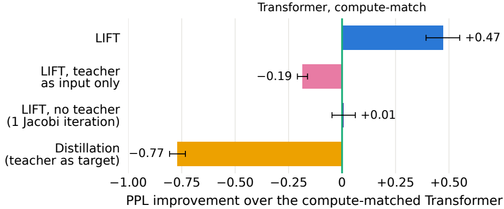
Figure 5: Teacher ablation at 135M: spending LIFT’s extra forward pass. Each bar is a model’s perplexity improvement on the full C4 validation subset over the compute-matched Transformer, which spends that compute on more tokens (the zero line; right is better): the mean over three training seeds of the per-seed difference, with whiskers of \pm 1 sd.
