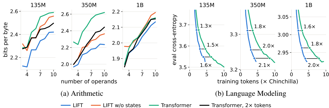
Figure 3: LIFT performance on arithmetic and language modeling. (a) LIFT shows a consistent advantage on arithmetic that persists as task complexity increases, outperforming a baseline trained on 2 \times more tokens. (b) Throughout training, LIFT is more token-efficient than a vanilla Transformer, and the advantage grows with training: each horizontal segment marks the additional tokens the Transformer needs to reach the same loss.
