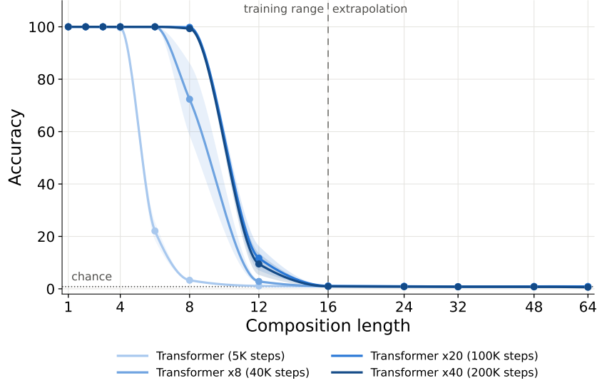
Figure 4: The same two-layer Transformer on S_5 at four training budgets, darker lines for longer training. Bands show standard error over three seeds. Training beyond 100K steps ( 20\times ) brings no further gain.
