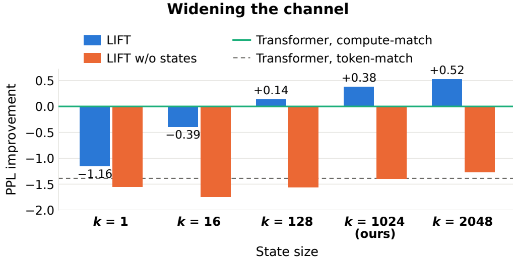
Figure 6: Channel width at 135M: improvement in perplexity over the compute-matched Transformer (the zero line; up is better) for k from 1 to 2048, with the model’s own states fed back (LIFT) and for the same model run without states (LIFT w/o states). Dashed: the token-matched Transformer. Every step in k is beyond the paired bootstrap 95% interval over evaluation sequences (Table 6’s protocol).
