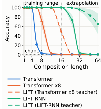
Figure 2: S_5 accuracy at increasing task lengths N (linear for N \leq 16 , logarithmic for N > 16 ), of Transformers (solid lines) versus LIFT models (dashed lines). Standard error is over seeds.
