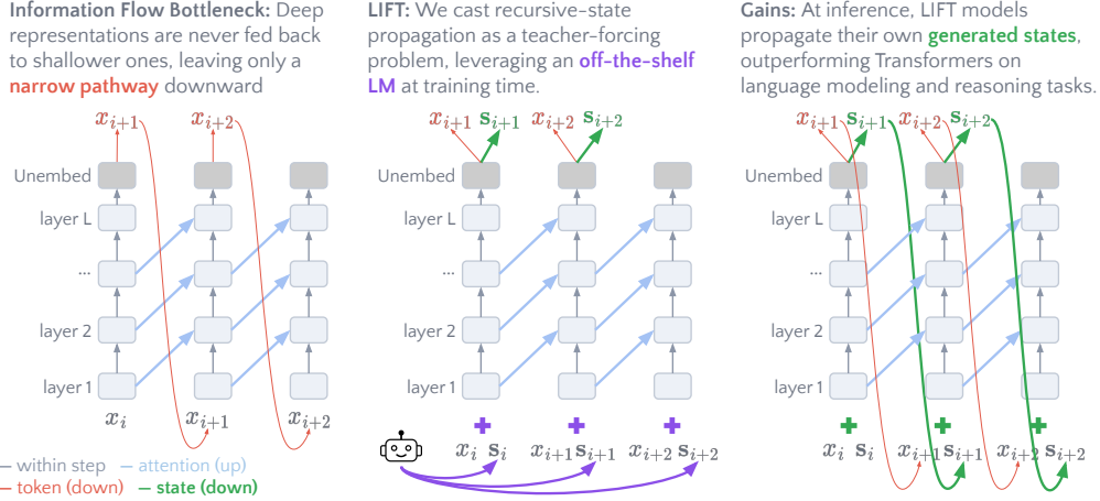
Figure 1: We remove the information flow bottleneck in Transformers (left) by introducing the LIFT architecture and pretraining approach (middle), which allows state propagation at inference (right).
