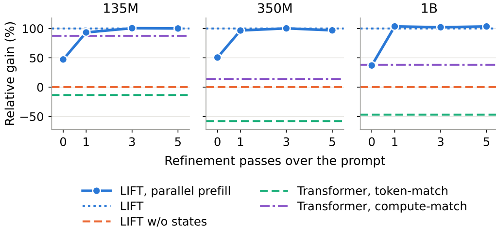
Figure 7: Relative gain of LIFT with parallel prefill (blue points) by the number of refinement passes over the prompt, against LIFT (100%) and LIFT w/o states (0%). The token- and compute-matched Transformers are placed on the same scale; below 0%, a model is behind LIFT w/o states.
