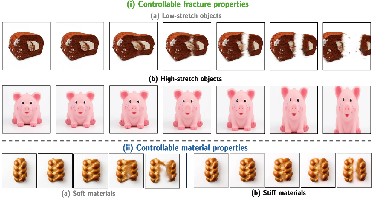
Figure 6: Controlled deformation and tearing. (i) Generated sequences for objects with low- and high-stretch fracture settings. (ii) Changing material stiffness for the same object produces different deformation and tearing behavior.
