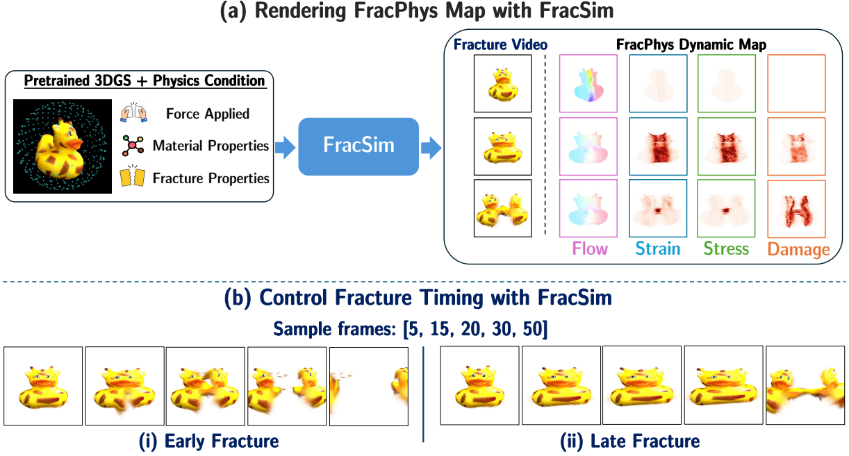
Figure 2: FracSim generates physically plausible fracture dynamics spanning deformation to structural failure. (a) Alongside RGB video, FracSim outputs FracPhys map. (b) Our damage model enables explicit control over fracture timing under fixed forces and material properties.
