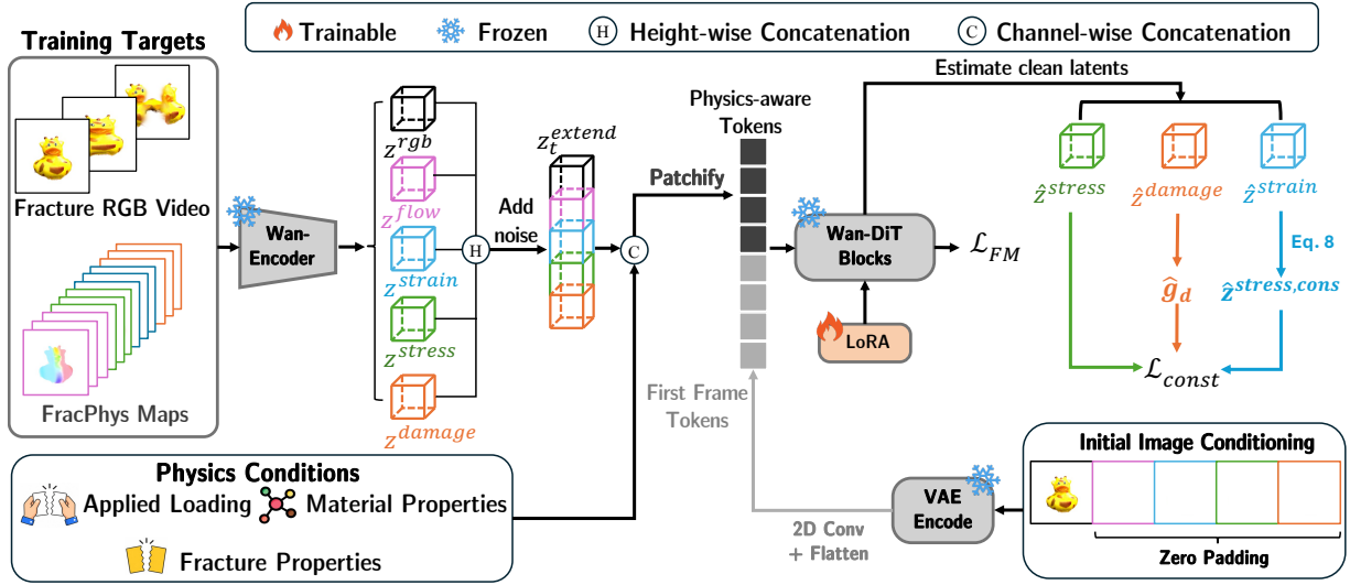
Figure 3: FracGen overview. RGB fracture videos and FracPhys Maps are encoded by a frozen VAE and concatenated along the spatial height dimension for joint generation. Applied loading, material properties and fracture properties provide channel-wise conditioning. The initial object image supplies reference tokens. We adapt the transformer with LoRA using flow-matching supervision and a physics-informed latent consistency regularizer coupling strain, stress, and damage representations.
