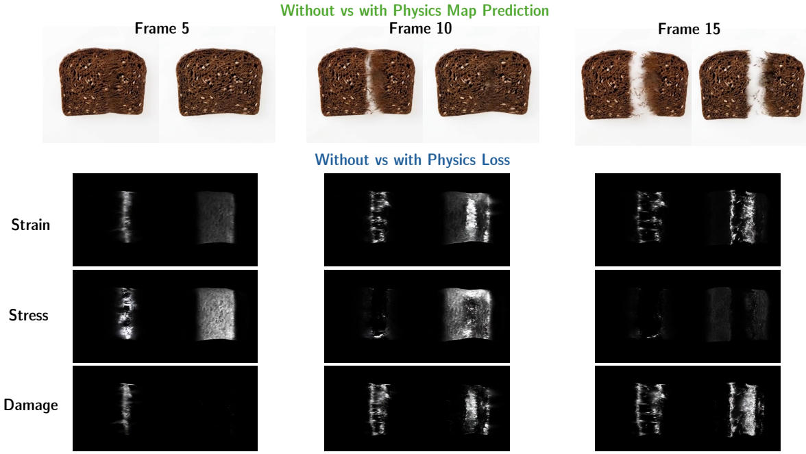
Figure 11: Ablation Studies. Comparison results for ablating the effect of physics map prediction and physics consistency loss.
