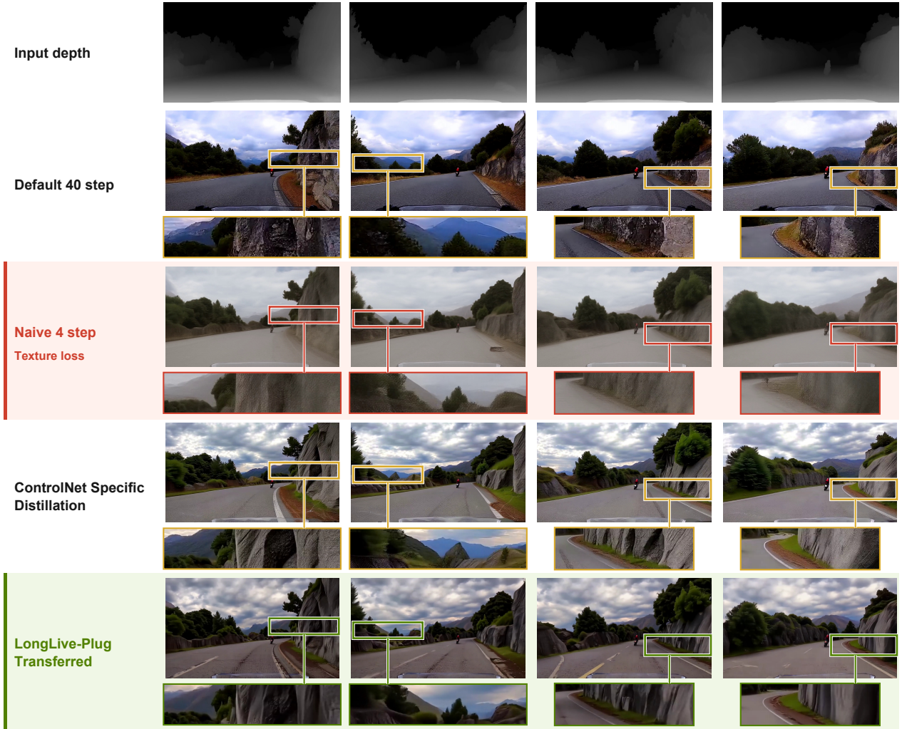
Figure 9 | Keyframe comparison on Wan2.2-Fun-5B-Control. Four matched keyframes compare input depth and four generation methods. Boxes mark identical image coordinates across methods, magnified in the strips below each output. Red highlights the naive four-step row’s smeared rock, foliage, and road details and low contrast. Columns match conditioning frame indices (depth at 30 fps, outputs at 24 fps). The transferred output uses an additional base-distilled adapter variant.
