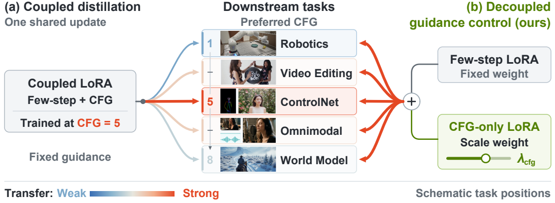
Figure 2 | Decoupled guidance control through an additional CFG-only LoRA. (a) Scaling a single distilled LoRA changes the entire update, including its learned guidance and few-step behavior. (b) Adding a separately weighted CFG-only LoRA lets us adjust guidance for each target while keeping the few-step adapter weight fixed. Arrow colors and widths schematically illustrate guidance compatibility, with the warmest coupled-transfer arrow at CFG 5. CFG-only LoRA scaling provides an adjustable guidance control.
