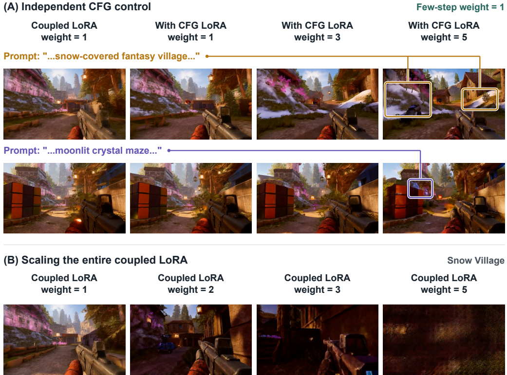
Figure 6 | Independent CFG control on SCOPE. (A) The coupled LoRA alone at weight 1 shows little response to the prompts. Adding a separately weighted CFG LoRA strengthens the boxed prompt attributes while the coupled LoRA weight remains at 1. Colored lines link each box to its corresponding prompt text. (B) Scaling the entire coupled LoRA instead degrades generation. Frames are matched across weights within each row. All runs use four-step sampling with distilled CFG; (A) and (B) use different coupled checkpoints.
