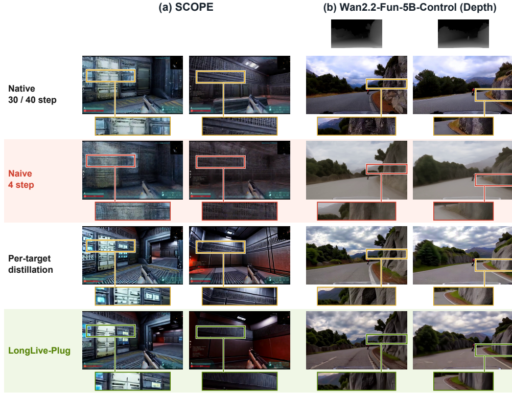
Figure 4 | Matched transfer comparisons on SCOPE and Wan2.2-Fun-5B-Control (Depth). Two matched frames per task compare native (30/40 steps), naive four-step, per-target distilled, and LongLive-Plug outputs. Naive four-step sampling produces blurry, low-quality videos, whereas LongLive-Plug maintains high visual quality at four steps. Depth thumbnails condition ControlNet; boxes and strips show matched regions across methods. LongLive-Plug uses an additional base-distilled adapter variant. Appendix B gives full four-frame comparisons and alignment details.
