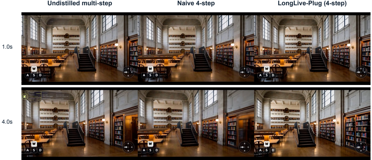
Figure 13 | H3 camera transfer includes a quality–control trade-off. Left: undistilled multi-step inference. Middle: naive four-step sampling. Right: four-step inference with LongLive-Plug. In the museum-crane example, S4 retains clearer architectural detail and a visible upward-camera response. In the library-yaw example, S4 remains sharp but its change in framing is attenuated relative to D/E4. HUD elements are inherited from the supplied anchor images. These cases have no generated-video pose regression metric and do not establish precise trajectory adherence.
