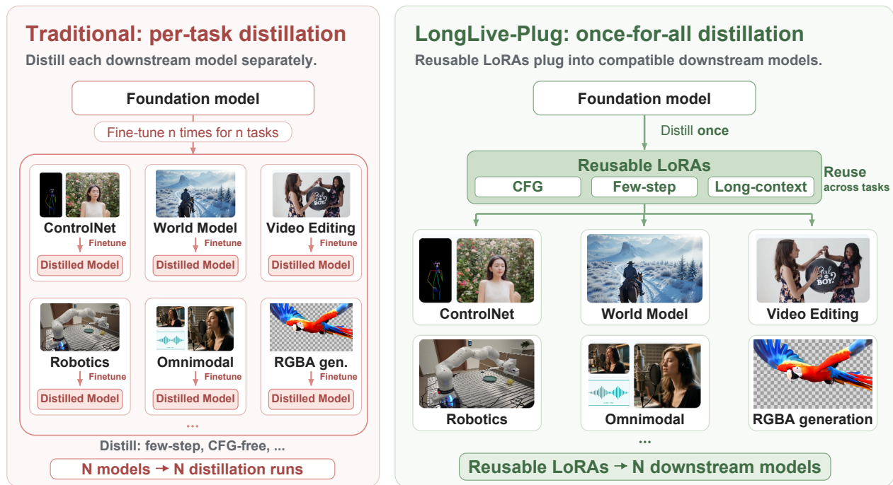
Figure 1 | Once-for-all distillation with plug-and-play deployment. Conventional pipelines separately distill every downstream model (left). LongLive-Plug distills CFG, few-step, and long-context capabilities into reusable LoRAs on each base model, then transfers them to compatible downstream models without target-specific training (right).
