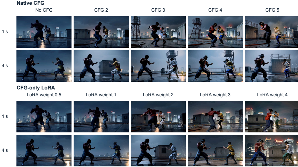
Figure 15 | Native CFG and CFG-only LoRA on Rooftop Martial Arts. Matched frames at 1 and 4 s compare native CFG (top: no CFG and scales 2–5) with CFG LoRA (bottom: weights 0.5, 1, 2, 3, 4). The prompt, seed, and native schedule are fixed; LoRA outputs use one conditional forward pass per step. LoRA weights are not calibrated native CFG scales.
