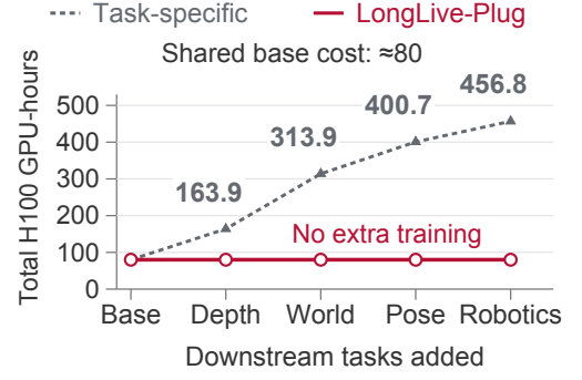
Figure 3 | Cumulative distillation cost. Both curves include the shared base cost of approximately 80 GPU-hours.
