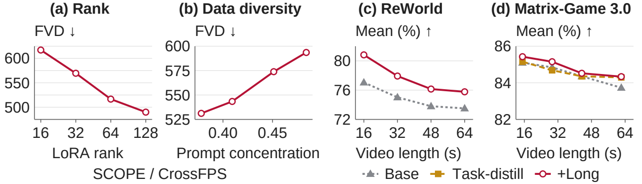
Figure 7 | Rank, data diversity, and long-context transfer. (a–b) Higher rank and more diverse prompts (lower concentration) improve FVD after transfer. (c–d) Mean of seven VBench dimensions after transfer to ReWorld and Matrix-Game 3.0, respectively. Long-context comparisons are within each model. Our transferred long-context LoRA improves quality during long AR rollouts.
