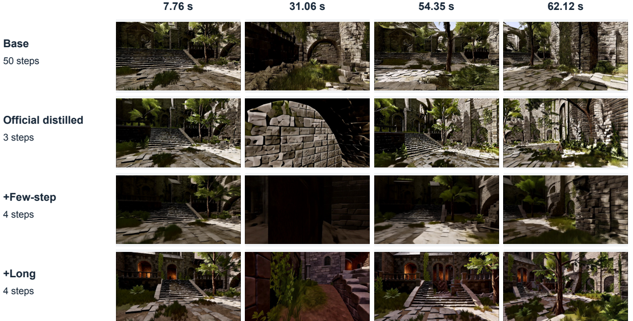
Figure 21 | Long-context transfer to Matrix-Game 3.0: overgrown temple. The same methods and timestamps as Fig. 20 compare stone architecture and vegetation. The +Long frames preserve visible stone-block boundaries, steps, and foliage late in the rollout, while appearance and layout vary across methods.
