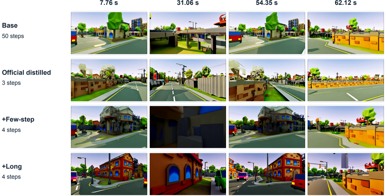
Figure 20 | Long-context transfer to Matrix-Game 3.0: animated city. Columns show native frames 132, 528, 924, and 1,056 (zero-based), spanning early, middle, and late stages of the same 62.18 s rollout. The +Long output retains distinct facade edges and street objects at late times.
