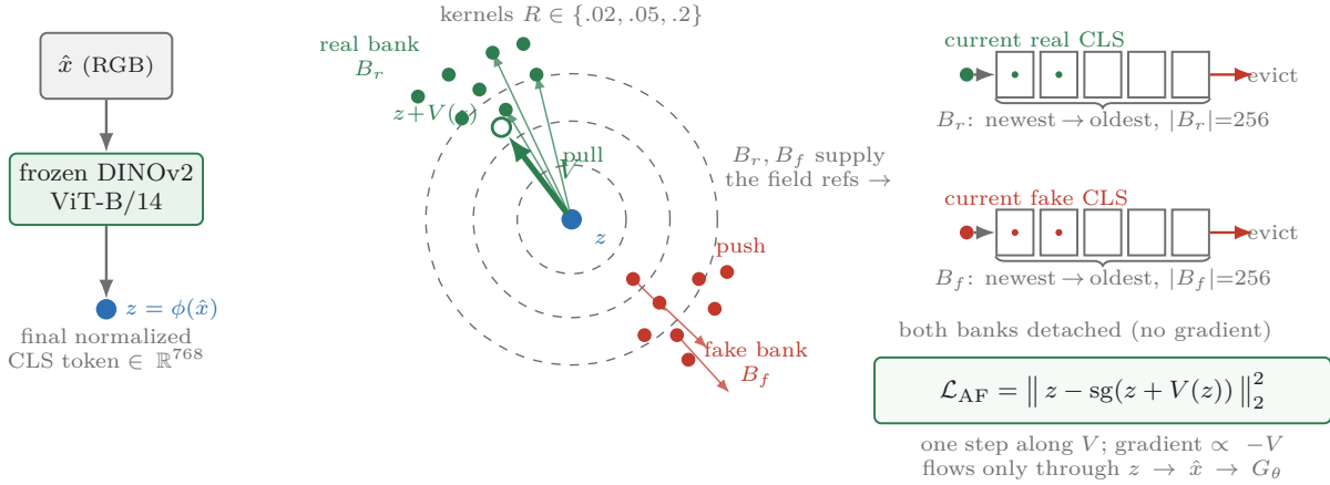
Feature extraction Attract–repel vector field in DINOv2 CLS space Rolling banks & Anchor-Field loss
