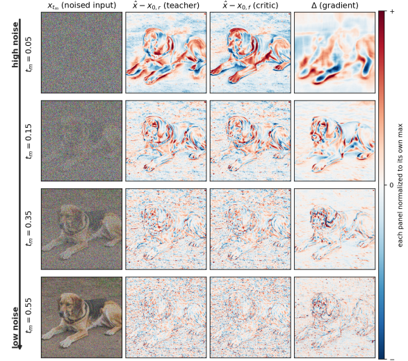
Figure 4 Eq. 1 terms across t_m ; \Delta exhibits broader coherent patterns at high noise and sparse fine-scale patterns near clean. Each panel is independently normalized for spatial visualization; colors are not comparable in magnitude across cells.
