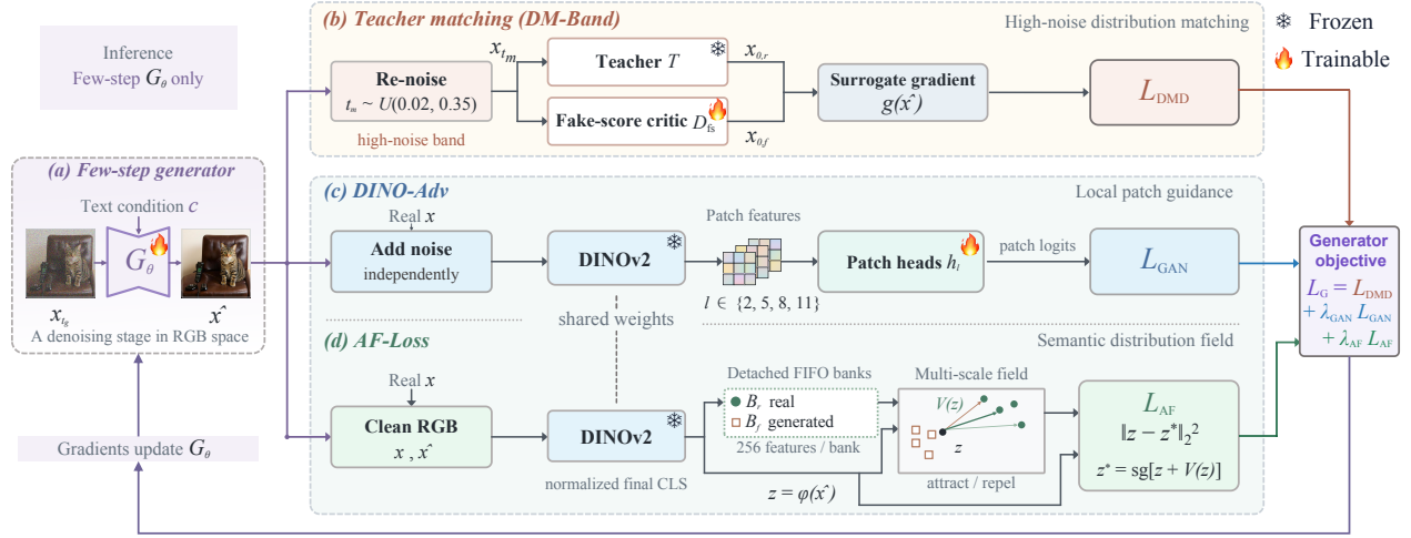
Figure 2 Overview of the proposed DMA 2 framework. DM-Band restricts teacher matching to a diagnostically selected high-noise range. For real-data guidance, DINO-Adv and AF-Loss share a frozen DINOv2 encoder and provide local patch guidance and a parameter-free semantic distribution-field target, respectively. Only G_\theta , the fake-score critic, and the adversarial heads are trained; all auxiliary components are removed at inference.
