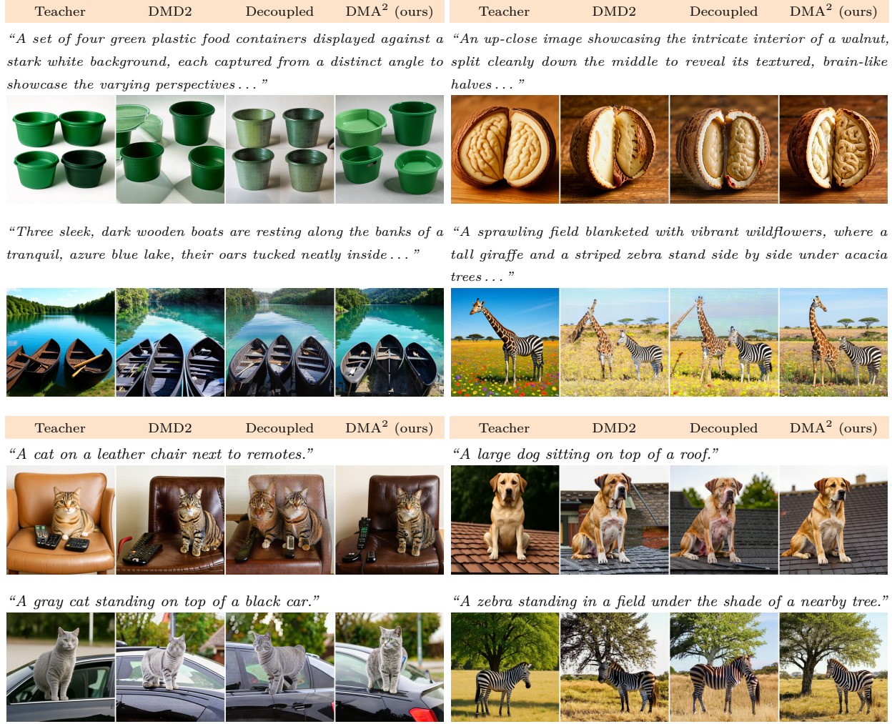
Figure 6 Qualitative comparison at four steps. Top block: long, densely specified DPG-Bench prompts (abbreviated with “...”); bottom block: short COCO captions. DMA 2 preserves object count and composition and recovers fine structure, across both long and short text.
