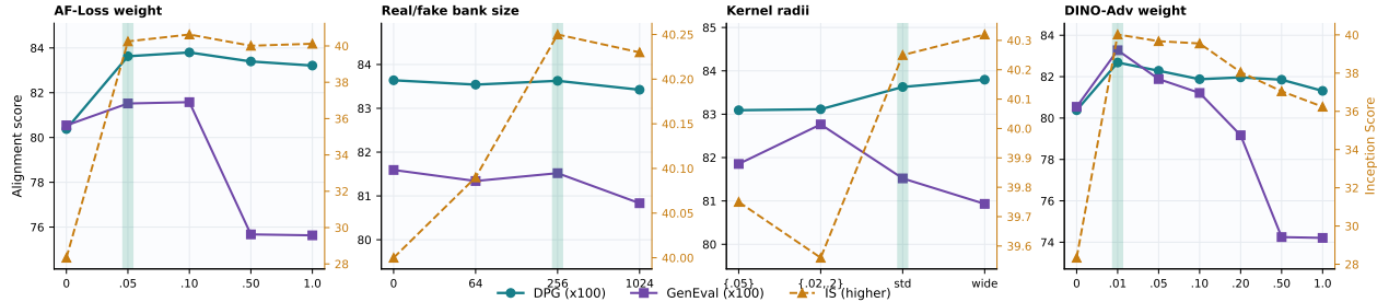
Figure 7 Hyperparameter sensitivity in DPG, GenEval, and IS; green bands mark defaults. These are OFAT sweeps around an anchor that is not the full model, so their default and zero-weight points are not directly comparable to the Table 2 component ablation (anchor protocol in Appendix D).
