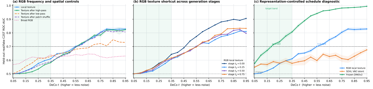
Figure 3 Separability diagnostic (C2ST). Each panel plots a held-out classifier’s real/fake separability ( y -axis: ROC-AUC over 1,536 matched real/generated pairs, 0.5 is chance) against the DeCo matching level t ( x -axis; larger t is less noise). The panels vary the setup: (a) the RGB input transform (raw texture, high-pass, low-pass, 32 \times 32 patch shuffle); (b) the generation stage t_g \in \{0, .25, .5, .75\} ; (c) the input representation (RGB, the SDXL latent, frozen DINOv2). RGB separability changes sharply with t and is high only near clean, whereas the SDXL latent stays flat and DINOv2 stays separable into the high-noise band.
