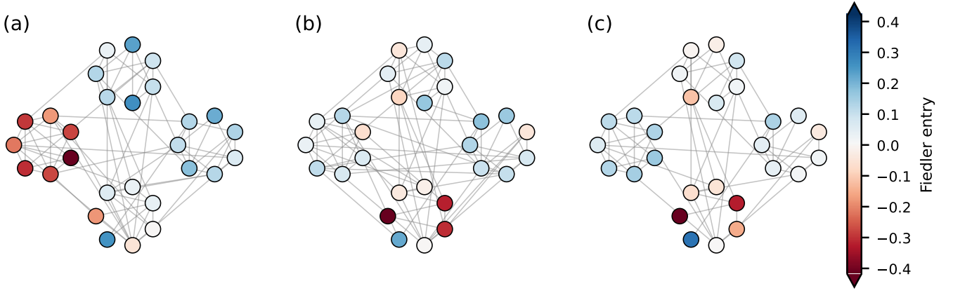
Fig. 1. Two reconstructions of community instance g5 ( n = 28 ); layout and node color are fixed from the original graph, so only the edge sets differ. (a) Original. (b) Preserves the edge count (ECR = 1) while adding and deleting 19 edges each, certified mixed from scalar summaries. (c) Verbatim return of the prompted sublist. EMD and edge-count summaries can thus obscure the edit mechanism; neither reconstruction is implied to be faithful.
