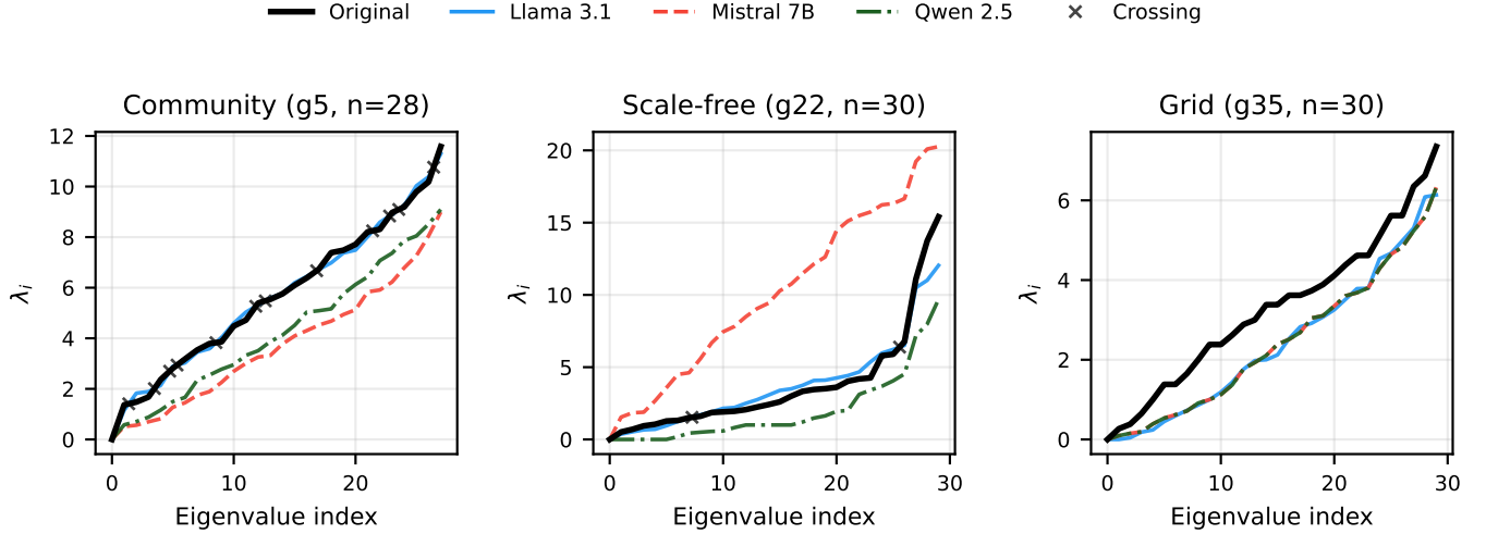
Fig. 3. Sorted Laplacian spectra for one medium instance per family; crossings mark X > 0 (Proposition 12). The two crossing curves are the certified reconstructions of g5 and g22. In g35 the Mistral and Qwen curves coincide (identical edge lists) while the Llama curve is mixed yet spectrally dominated, the one corpus instance whose added and deleted edges are vertex disjoint.
