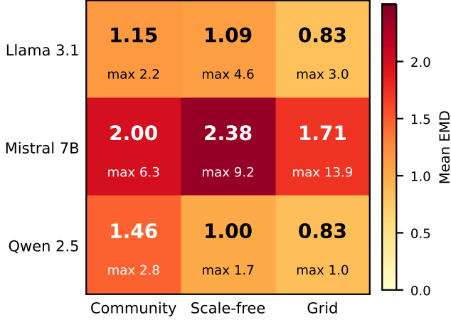
Fig. 4. Mean EMD and cell maximum over 15 outputs per model-family cell. The Qwen row largely tracks the benchmark density profile; the Mistral grid cell is driven by one instance.
