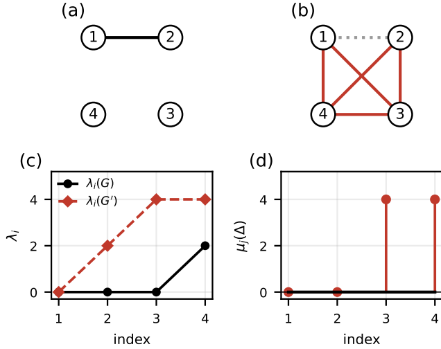
Fig. 2. The mixed edit of Example 9. (a) G . (b) G' = K_4 minus \{1, 2\} ; hallucinated edges solid red, deleted edge dotted gray. (c) Pointwise dominance without a crossing, attaining the lower bound of (3). (d) The perturbation spectrum is nonnegative although the edit is mixed.
