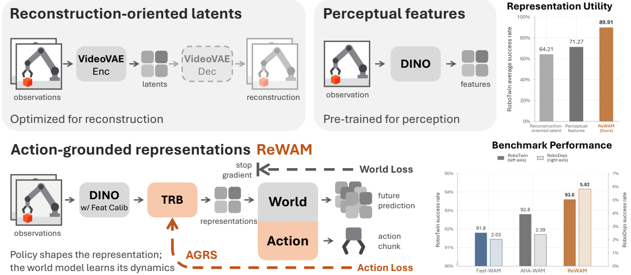
Figure 1: Overview of representations for world-action modeling. Top-left: Video-VAE latents are optimized for visual reconstruction. Top-right: Frozen DINO features inherit priors from perceptual pre-training. Bottom: ReWAM uses a Temporal Representation Bottleneck (TRB) to form compact world states from calibrated DINO features. Action-Grounded Representation Shaping (AGRS) trains the TRB through asymmetric routing of action-loss gradients, while the world model learns state transitions.
