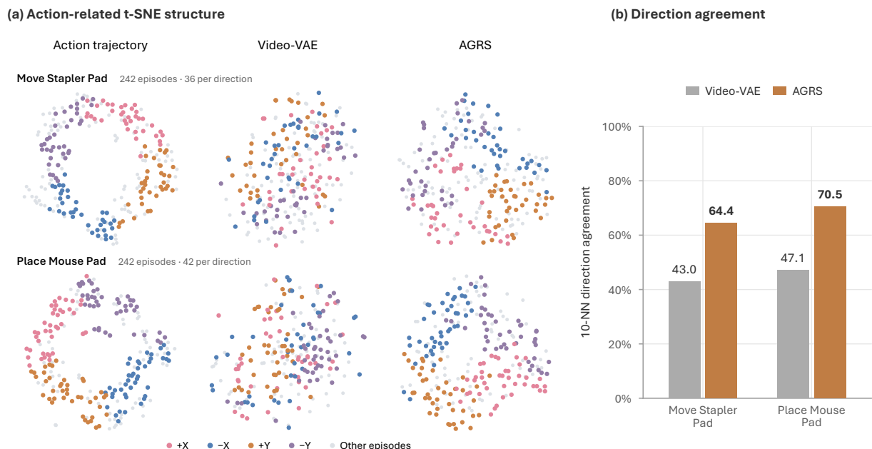
Figure 2: Action-related structure in representation variations. (a) Independent t-SNE projections of commanded end-effector trajectories, Video-VAE variations, and AGRS variations (left to right) for Move Stapler Pad (top) and Place Mouse Pad (bottom). Each task shows the same 242 transitions in all three projections; colors identify motion directions in balanced subsets, with the remaining transitions in gray. (b) Mean direction agreement among ten nearest neighbors in the original representation space. AGRS shows higher agreement than Video-VAE on both tasks.
