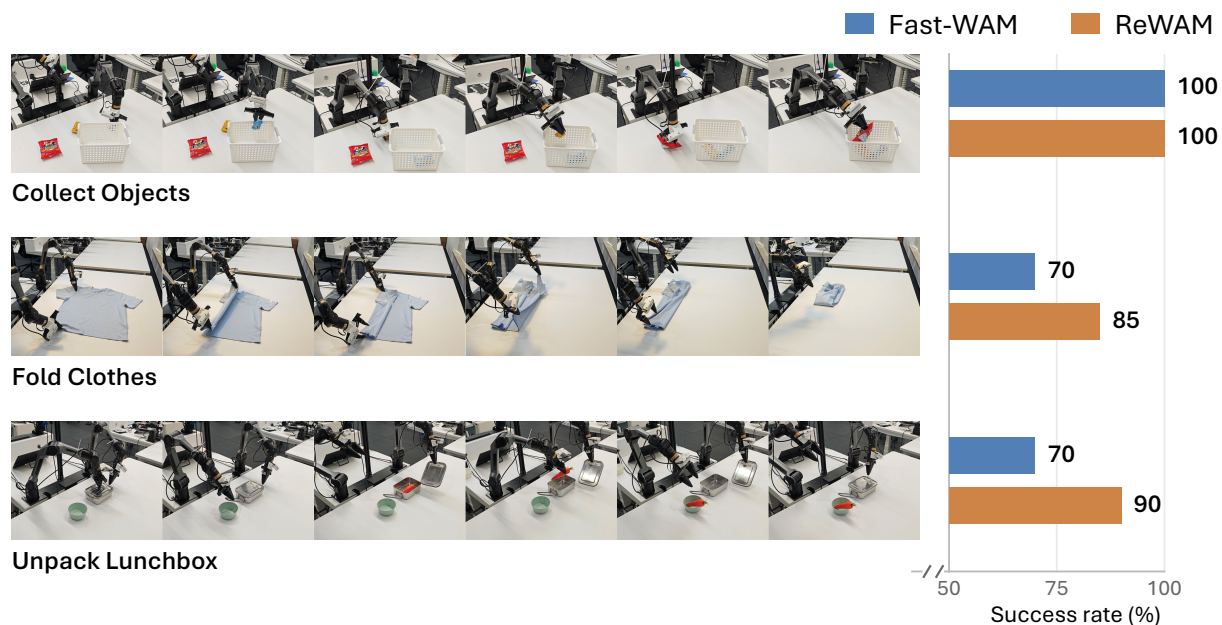
Figure 3: Real-robot task success. Task photos and success rates over 20 trials per task. ReWAM achieves 91.7% average success versus 80.0% for Fast-WAM. The horizontal axis starts at 50%.
