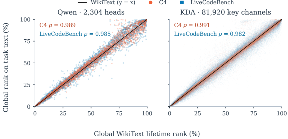
Figure B3: Global lifetime rankings remain similar across text sources. Qwen (2,304 heads) and KDA (81,920 key channels) are ranked separately, from shortest to longest gate half-life. Each point compares its global WikiText rank percentile with its C4 (orange-red) or LiveCodeBench (sky blue) percentile. The thin black diagonal is WikiText compared with itself ( y = x ). Spearman coefficients use the complete population in each panel.
