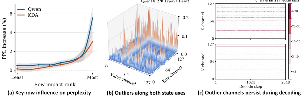
Figure 2: Spatial structure of recurrent states. (a) Key rows are ranked by readout impact and divided into eight groups. Quantizing one group at a time to INT4 generally causes larger perplexity increases for higher-impact groups. (b) A representative Qwen state exhibits obvious outliers in both key rows and value columns. (c) Channel RMS relative to the median across 2048 decoding steps. The outliers remain prominent throughout decoding.
