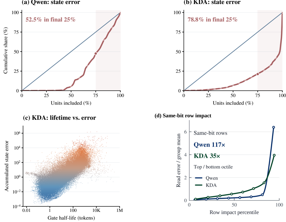
Figure B1: Gate lifetime and key-row impact of recurrent state. (a–b) Cumulative INT6 squared error (red) and unit count (blue), ordered by increasing gate half-life within each layer or head. The longest-lived quarter accounts for 52.5% of Qwen error and 78.8% of KDA error across all 2,304 heads and 81,920 channels. (c) KDA half-life versus accumulated INT6 error for 79,864 channels after excluding near-zero errors; color encodes error. (d) Held-out equal-norm readout-error contrast across row-impact octiles within fixed-precision groups, using independent WikiText ranking.
