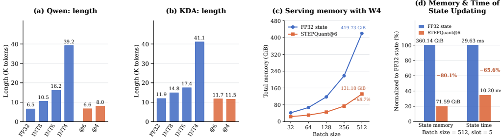
Figure 3: Generation length and serving efficiency of STEPQuant. (a–b) Mean generated tokens across seven tasks, weighting tasks equally. Blue bars show FP32 and uniform INT8/6/4. Orange bars show STEPQuant@6bit/@4bit (marked @6/@4). Lengths include thinking, incorrect answers, and capped outputs. (c) Total serving memory of Qwen with W4 weights across different batch sizes. (d) Normalized recurrent-state memory and updating time of Qwen at batch size 512.
