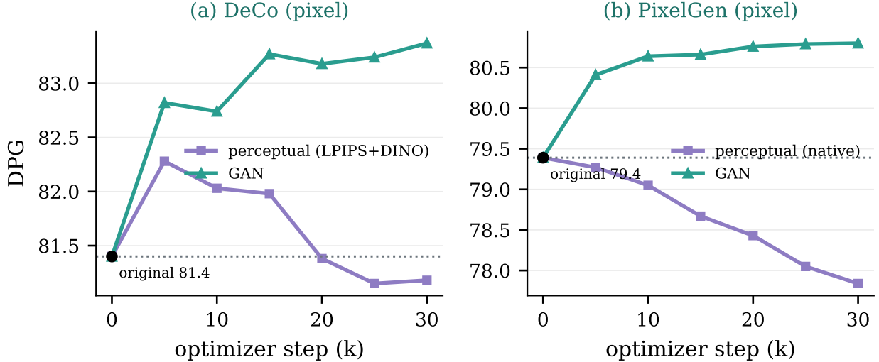
Figure 4 DPG Score (Hu et al., 2024) trajectories initialized from the official, pre-SFT checkpoints. The GAN curves use an image-only DINOv2 discriminator. (a) DeCo; (b) PixelGen.
