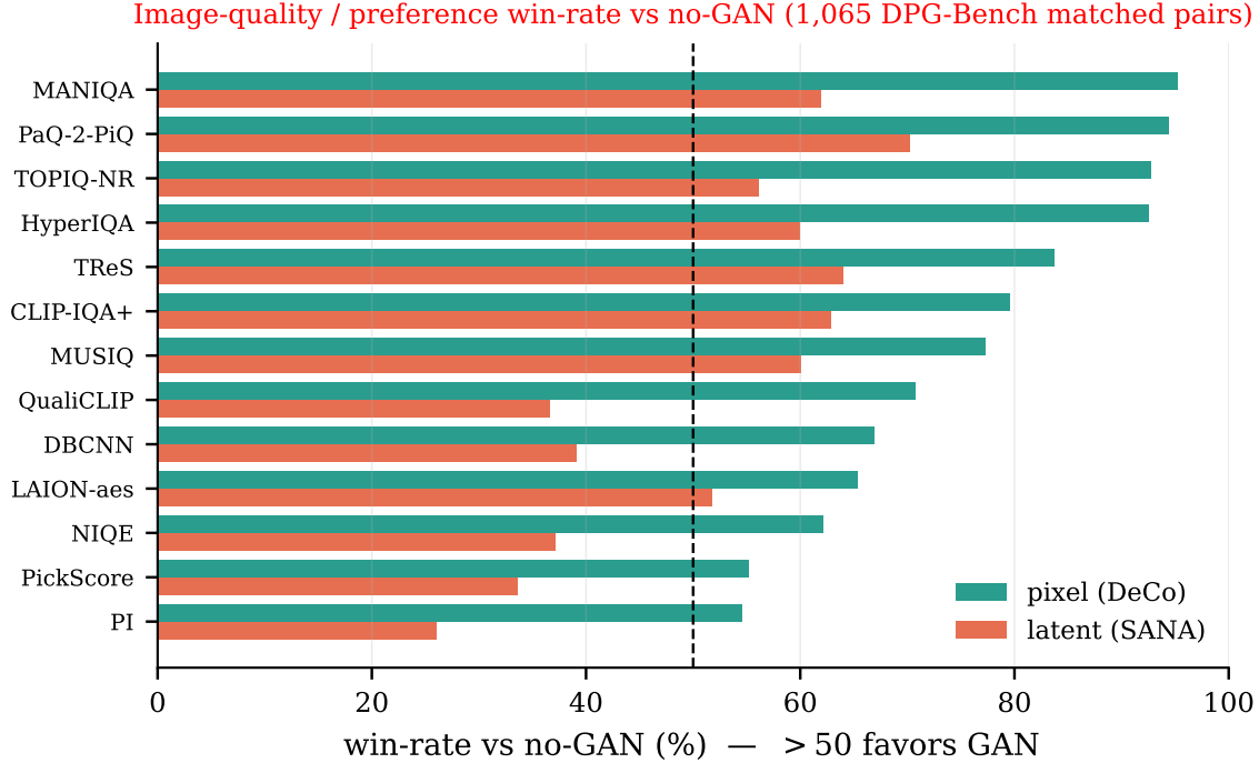
Figure 6 Image-quality / preference win-rate vs. no-GAN (1,065 DPG-Bench matched pairs (Hu et al., 2024)). The pixel diffusion’s GAN (DeCo) is preferred across metrics, well above the latent diffusion’s GAN (SANA).
