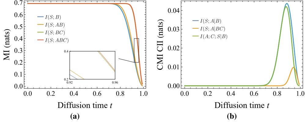
Figure 4: Exact numerical evaluation of the Gaussian-mixture information measures with specific values given in E.3. (a) Mutual information curves for the four spatial regions. The cliff diagnoses the symmetry-breaking phase transition. Inset: zoomed-in region near critical window. (b) Local and global conditional information gaps I_t(S; A|B) , I_t(S; A|BC) , and their difference which gives conditional interaction information I_t(A; C; S|B) . The peak diagnoses the non-locality transition.
