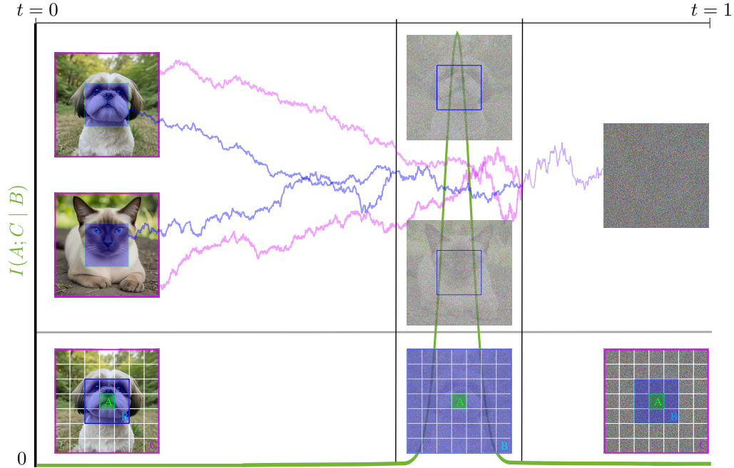
Figure 1: Semantic speciation locates the window in which local denoising breaks down. Denoising trajectory is from t = 1 (right) to t = 0 (left). The upper panel depicts a semantic speciation from white noise to cat or dog for local region (blue) and global region (magenta); the corresponding thresholds define a speciation window (black vertical lines). The noisy images in the window depict generation times in which the semantic identity is visible in the whole image, but invisible in a local patch (blue box). In the lower row, A is the patch to denoise (green), B its minimal surrounding context (blue) for below-threshold denoising, and C the rest of the image (magenta). The green curve depicts I_t(A; C | B) whose peak characterizes a breakdown of exact denoising using local context alone. Under the common-cause hypothesis, Theorem 1 places the threshold-defined nonlocality window inside the speciation window.
