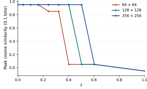
Figure 3: Label–reconstruction similarity remains high at early diffusion times and then falls toward zero. The sharp drop occurs first for the 64 \times 64 crop, then for the 128 \times 128 crop, and last for the full image.
