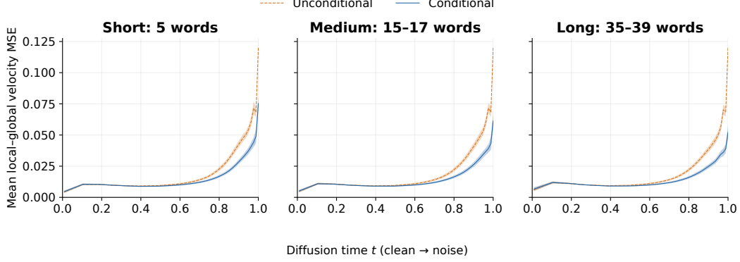
Figure 2: Semantic conditioning reduces the average local–global prediction gap in SD3. A smaller conditional gap means that restricting distant image–token interactions changes the model prediction less when semantic information is supplied. This is consistent with the common-cause interpretation: the description explains part of the shared image structure that would otherwise require distant context.
