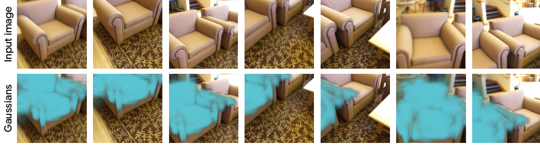
Figure 3: Visualization of clustered Gaussian from summary tokens. We visualize the Gaussians clustered from a set of Gaussian summary tokens via K-means over the summary tokens (cyan indicates the Gaussians belonging to one cluster). Similar summary tokens are mapped to the same object without any explicit clustering supervision.
