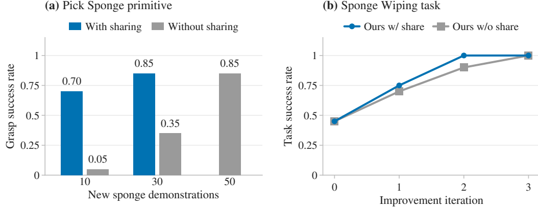
Figure 4: Sharing skill data reduces new teaching and supports policy improvement on new tasks. Left: cube-picking data improves sponge grasping at matched new-demonstration counts. Right: shared pick-and-place primitives support Sponge Wiping improvement with fewer new demonstrations than unshared primitives.
