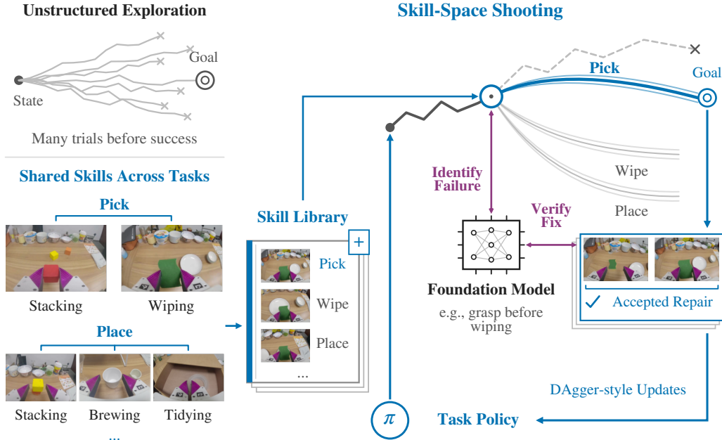
Figure 1: Skill-space shooting uses reusable skills to search for corrections that improve a task policy. We treat learned skills as candidate continuations from a state the policy has reached. We employ “shooting” across these skills, with foundation-model knowledge guiding which behavior to try and whether it successfully repairs the failure. Accepted repairs then train the policy for future attempts, closing the improvement loop. Sharing skills across tasks extends this source of corrective supervision while reducing the need for new teaching.
