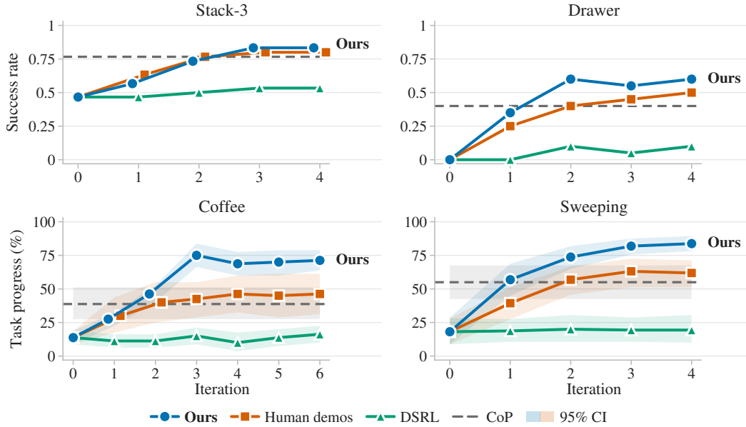
Figure 3: Skill-space shooting improves policies over iterations, even from zero observed initial successes. Baselines are latent-space RL (DSRL), additional demonstrations (HUMAN), and fixed primitive composition (COP). Top panels report full-task success; bottom panels show temporal progress with bootstrap 95% intervals.
