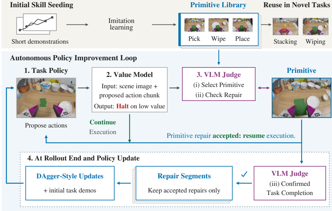
Figure 2: Trials of reusable skills supply corrective supervision for the task policy. A value model detects likely failures, and a VLM selects a skill and verifies its repair before the task policy resumes. Accepted repair segments from completed tasks train the next policy, which collects the next round of experience.
