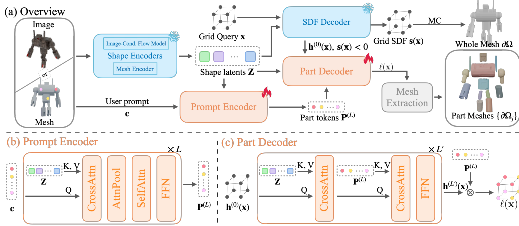
Figure 2: Method overview. (a) Given a mesh or an image, a shape encoder first encodes it to shape latents \mathbf{Z} ; the prompt encoder processes user prompts by attending to shape latents \mathbf{Z} to get part tokens \mathbf{P}^{(L)} ; the part decoder scores query points \mathbf{x} with the part tokens to predict their part assignments; mesh extraction converts these predictions into exclusive and exhaustive closed part meshes. (b, c) One layer of the prompt encoder and the part decoder, respectively.
