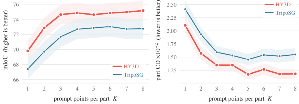
Figure 6: Segmentation quality against the number of prompt points per part K , for both backbones, with mIoU (left) and pCD (right). Both metrics improve steeply up to three points and change little beyond.
