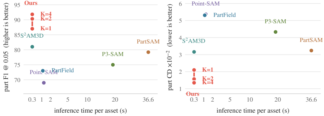
Figure 7: Segmentation quality against inference time per asset, pF1@.05 (left) and pCD (right), with our model at K \in \{1, 2, 4\} . Ours is the most accurate at close to the lowest time, and raising K improves quality at no cost in time.
