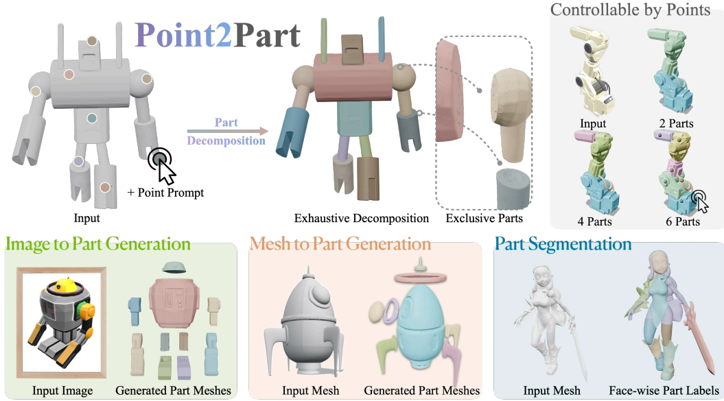
Figure 1: Unified 3D Partitioning from Point Prompts. (Top) We support 3D point prompts to specify desired parts and partition the input into closed, exhaustive, and mutually exclusive parts. (Right) Users can interactively control the partition through point prompts. (Bottom) We support image-to-part generation, mesh-to-part generation, and part segmentation within a single model.
