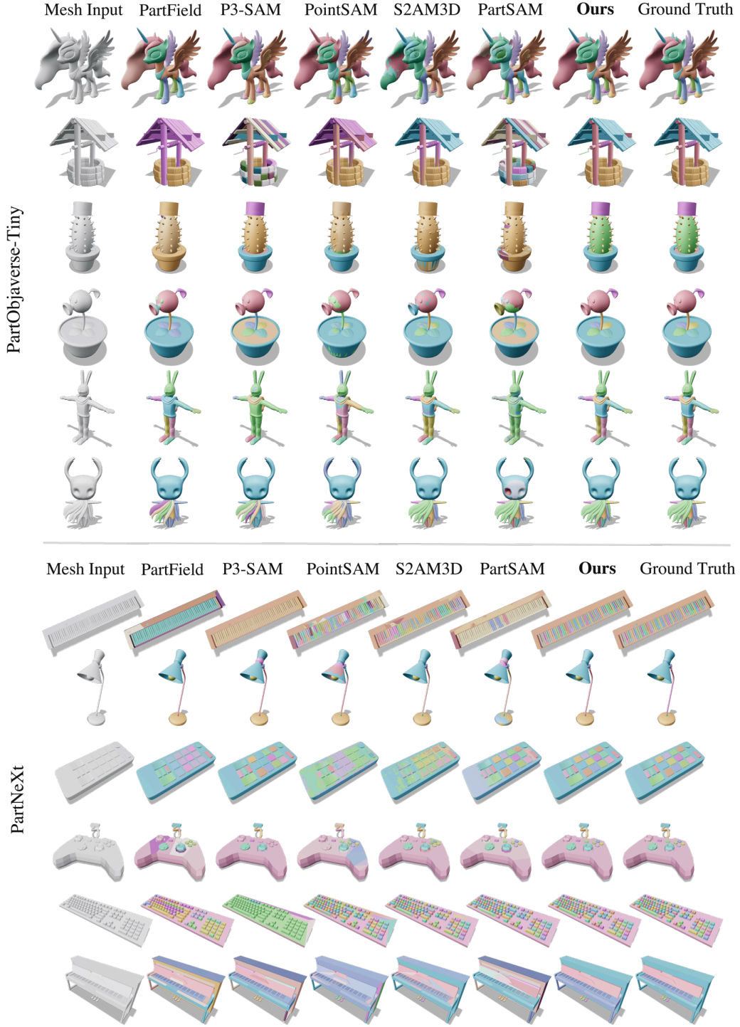
Figure 10: Part segmentation on PartObjaverse-Tiny (top) and PartNeXt (bottom). One point prompt per part, against the segmenters in Table 2 and the ground truth. Ours keeps small repeated parts separate, such as the spikes, keys, and buttons, where the baselines merge or fragment them.
