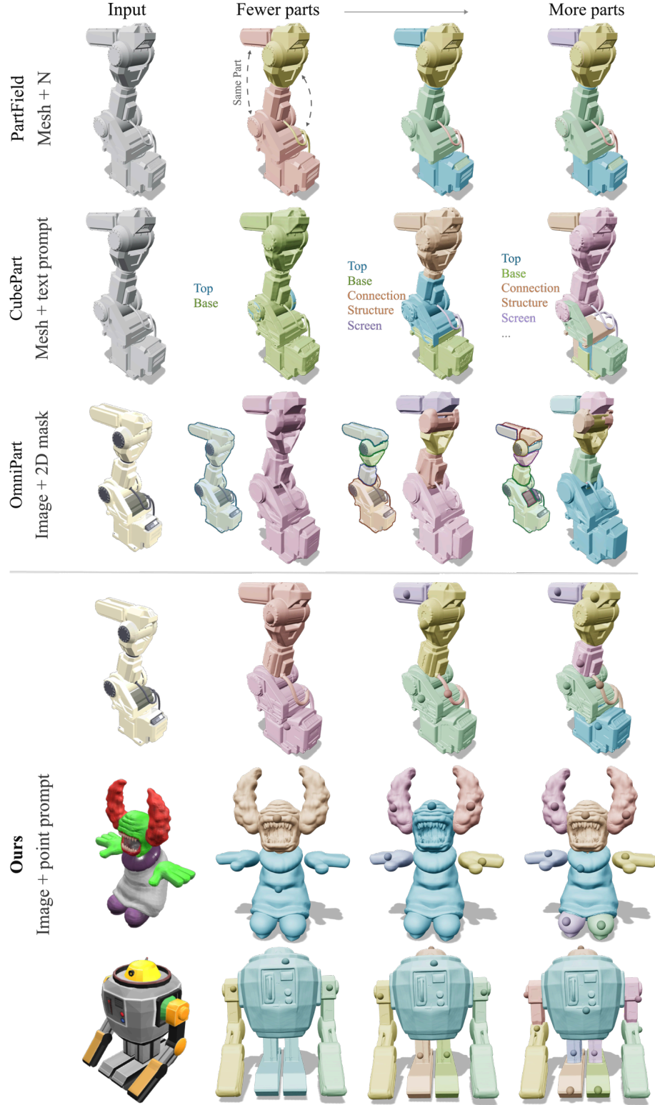
Figure 14: Controlling the decomposition. Objects are decomposed at three granularities, from fewer parts to more parts, through the specification each method takes: a part count for PartField, part names for CubePart, 2D masks on the image for OmniPart, and one point per part for ours. The top shows the same sample under every method; the bottom shows ours on two further samples.
