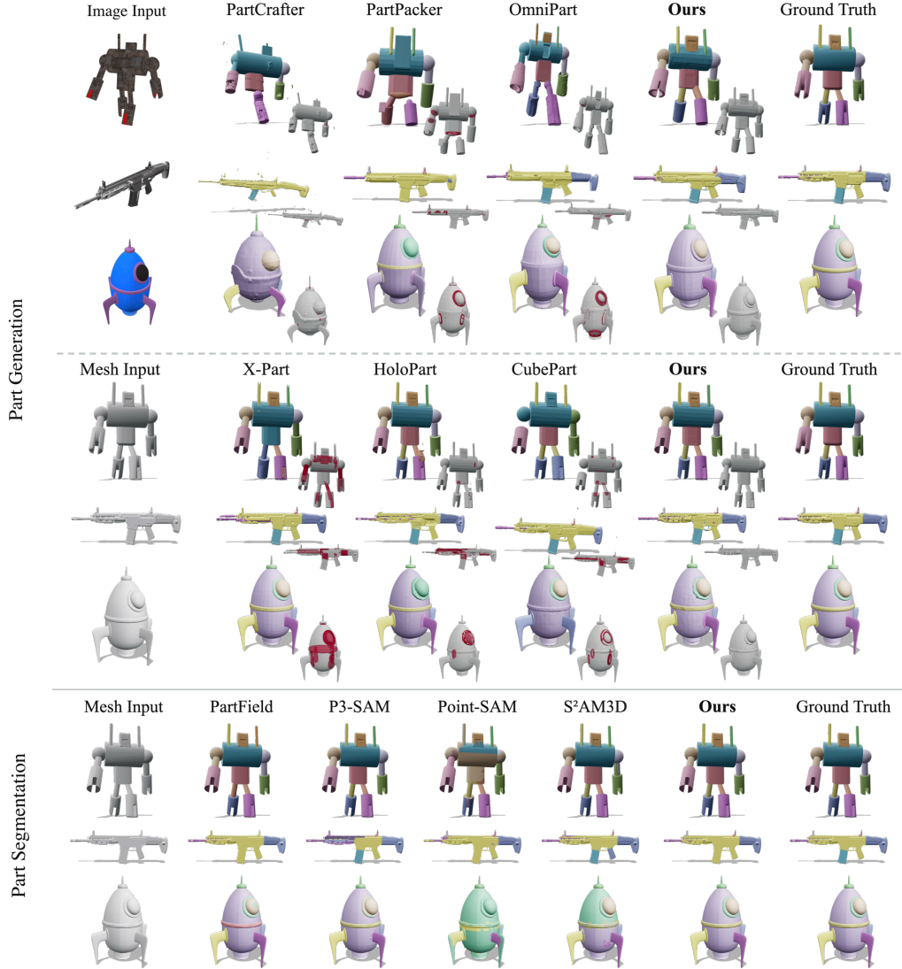
Figure 3: Qualitative comparison of our method with SOTA methods on the three tasks. Part generation from an image (top) and from a mesh (middle), and part segmentation (bottom). The grey mesh beside each generated result marks in red the volume claimed by more than one part. Prior methods overlap, drop, split, or merge parts, while ours matches the ground truth.
