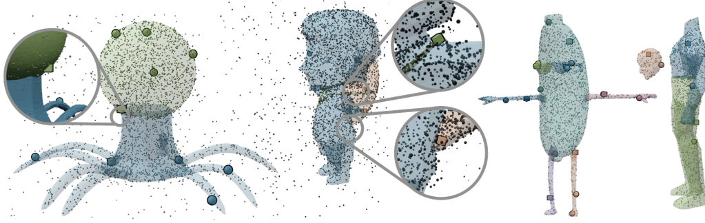
Figure 4: Training query sampling and prompt points. Small points are the sampled queries, colored by part; the larger markers are the prompt points, with balls and cubes marking two prompt sets for the same parts.
