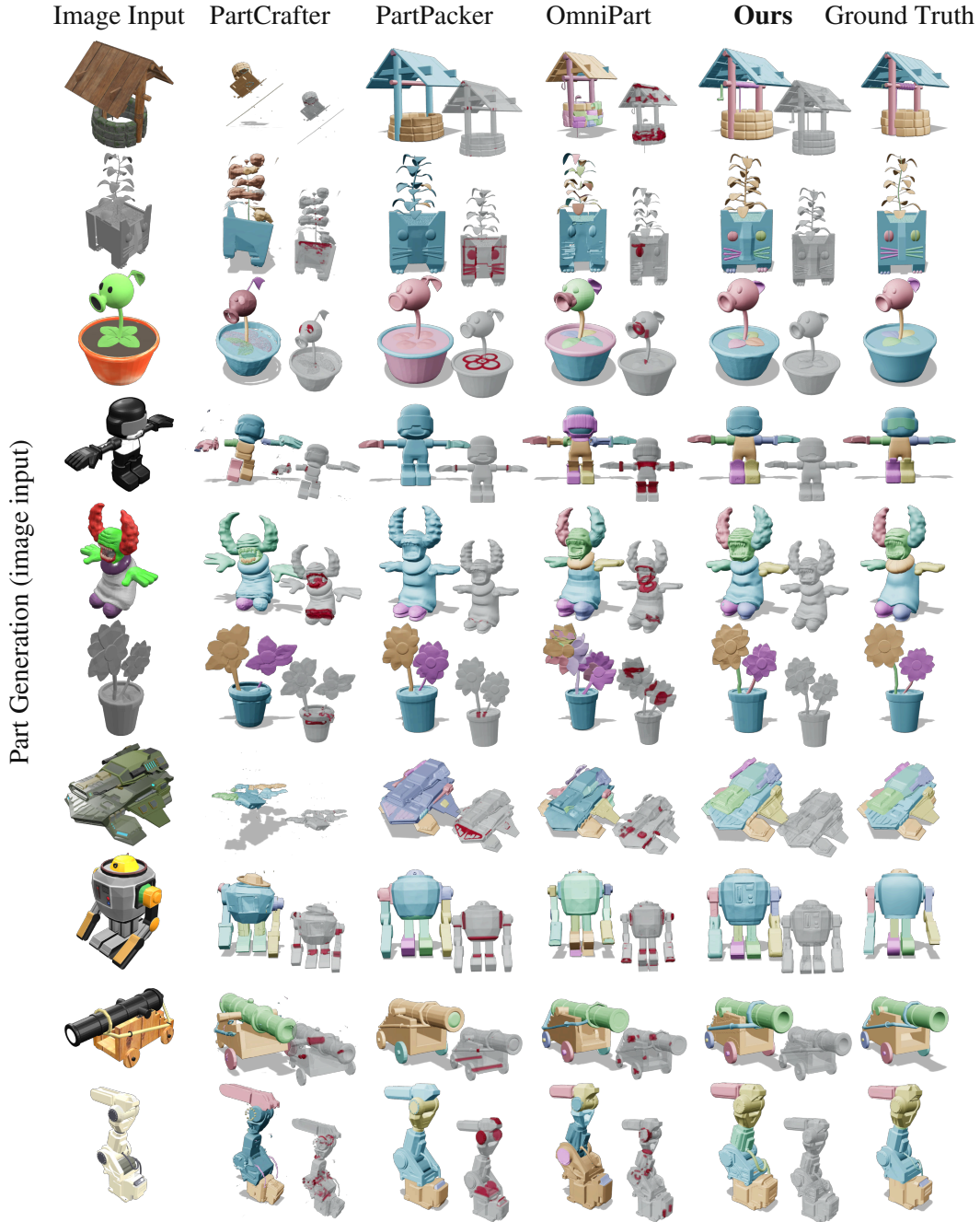
Figure 13: Part generation from a single image on further assets. Compared against the generators in Table 1, with the volume claimed by more than one part marked in red beside each result. The baselines interpenetrate at the joints or return a fragmentary object, whereas our parts meet with negligible overlap and follow the ground-truth decomposition.
