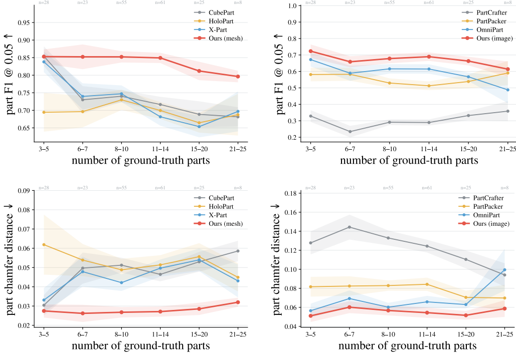
Figure 5: Part quality against the number of ground-truth parts, from a mesh (left) and from an image (right), with part quality metrics.
