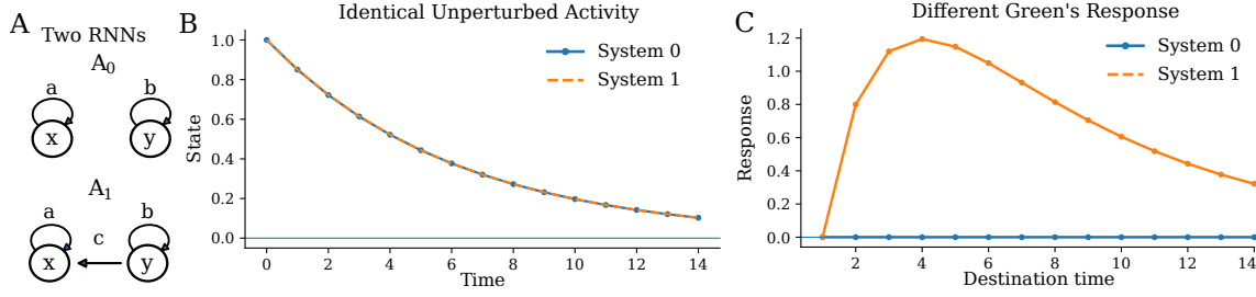
Figure 1: Routing is not determined by activity or local spectrum. Two linear recurrent systems generate the same unperturbed trajectory and have the same eigenvalues, but differ in whether a perturbation in y can influence x . The finite-horizon Green’s operator records this source-to-destination difference directly.
