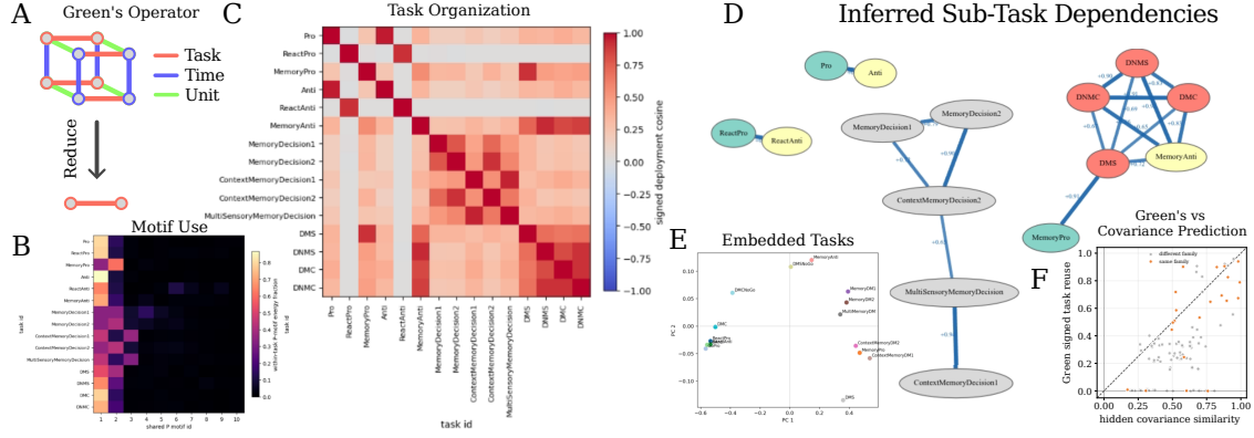
Figure 2: Task-level reductions of the Green’s operator expose computational reuse. A , reducing the full task/time/unit response operator gives a task-level view of perturbation reuse. B–E , known motif organization, pairwise Green-response similarity, strongest inferred relations, and a low-dimensional embedding provide complementary views of task organization. F , Green-response similarity and hidden-state covariance are related but non-equivalent; points distinguish task pairs from the same versus different families.
