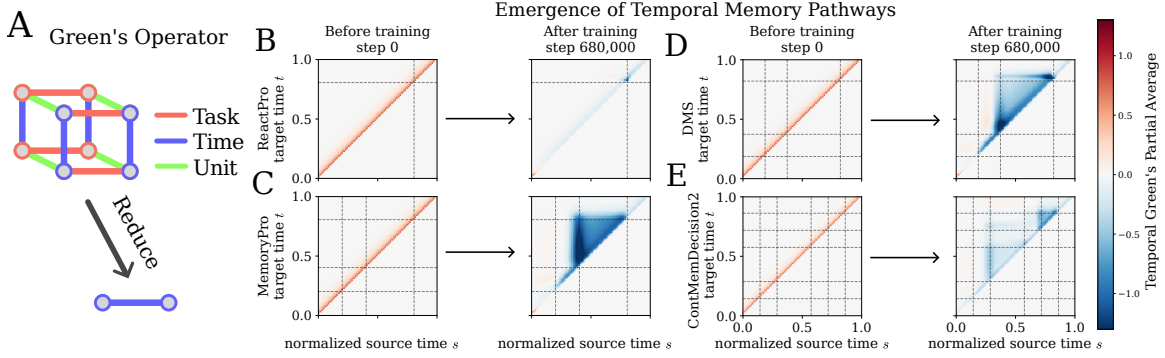
Figure 3: Task-specific temporal response pathways emerge during training. A , reducing the task-conditioned Green’s operator while retaining source and target time gives a temporal routing map. B–E , signed uniform-direction Green-response projections before training (step 0) and after training (step 680,000) for ReactPro, MemoryPro, DMS, and ContMemDecision2. Reactive computation remains comparatively local, while memory tasks develop delay-spanning pathways. Exact Frobenius-energy controls are given in Appendix D.
