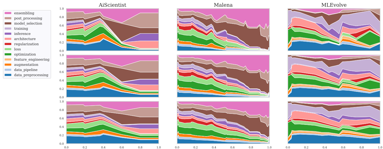
Figure 13 Category-share-decay curve on aptos2019 alone, at half-lives 0.1, 0.15, and 0.2 (rows, top to bottom). As in Figure 6, the x-axis is checkpoint fraction through the run ( \in [0, 1] ) and the y-axis is the decayed share of technique-category tags at that point.
