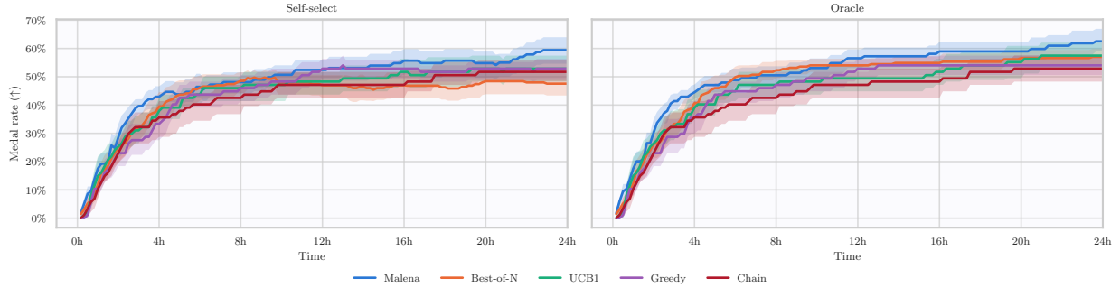
Figure 3 Performance evolution at 24h budget. Trajectories are extracted by selecting the best submission available at different times, aggregated in the default29 task set. Left: self-select medal rate. Right: oracle-best medal rate. Malena achieves the highest medal rate. Chain, Greedy and UCB1 perform similarly.
