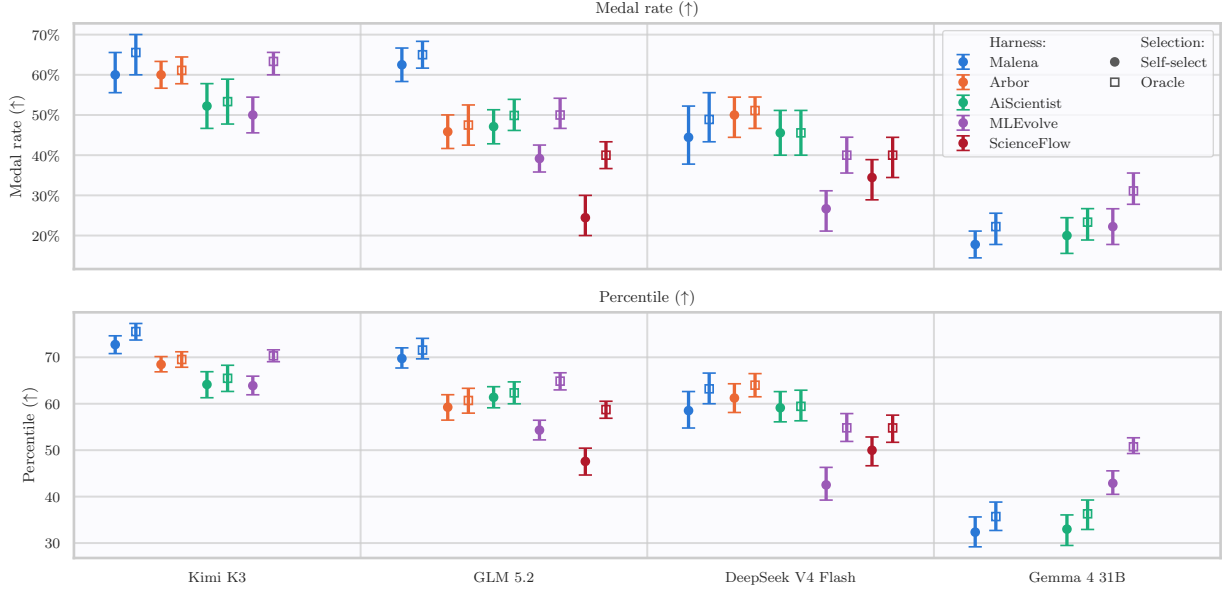
Figure 1 Performance across backbones and harnesses. Any-medal rate (↑, top) and mean percentile (↑, bottom), self-select (filled) vs. oracle (open), macro-averaged over the full fixed30 set at 24h time budget. Brackets are 95% bootstrap CIs. Backbones are grouped along a single shared x-axis; color identifies the harness.
