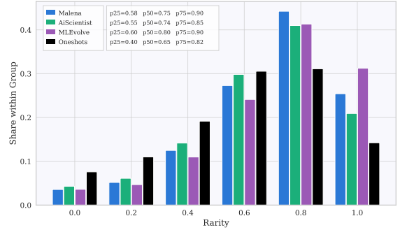
Figure 5 Per-technique rarity by method. Rarity of a technique is computed once per task over every method/backbone group’s runs combined (see Appendix E.2).
