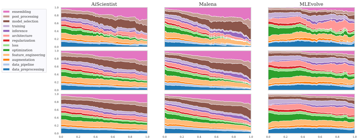
Figure 12 Pooled category-share-decay curve (all labeled tasks) at half-lives 0.1, 0.15, and 0.2 (rows, top to bottom) – smaller half-life is a more local, noisier snapshot of recently-introduced techniques. As in Figure 6, the x-axis is checkpoint fraction through the run ( \in [0, 1] ) and the y-axis is the decayed share of technique-category tags at that point.
