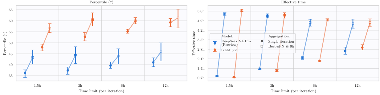
Figure 7 Impact of per-iteration time limits. Average percentile and effective-time obtained by Oneshot iterations under different per-iteration time budgets in the default29 set. Circled points represent single-iteration performance, while boxes indicate Best-of-N performance at six hour budgets. Error bars represent 95% CIs across our fixed 29-task set. The effective time measures the time taken for the run to finish. Best-of-N aggregates may remain below the target of 6h in the case of failing iterations that would exceed the maximum budget allocated.
