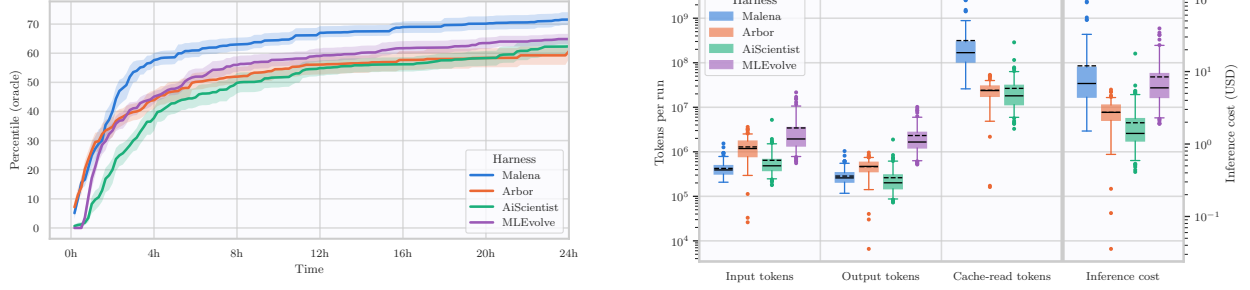
Figure 4 Left: oracle best-so-far percentile vs. wall-clock time, macro-averaged over fixed30 tasks, for different harnesses. Right: per-run distribution over all seeds of cumulative input, output and modelled cache-read tokens by the end of each run, plus a fourth group giving the resulting per-run USD cost (right-hand axis). Each box’s solid black line indicates median; dashed line indicates mean. MLEvolve’s cache is always exactly 0, since its tree-search nodes are independent LLM calls. All results shown are at the GLM 5.2 backbone.
