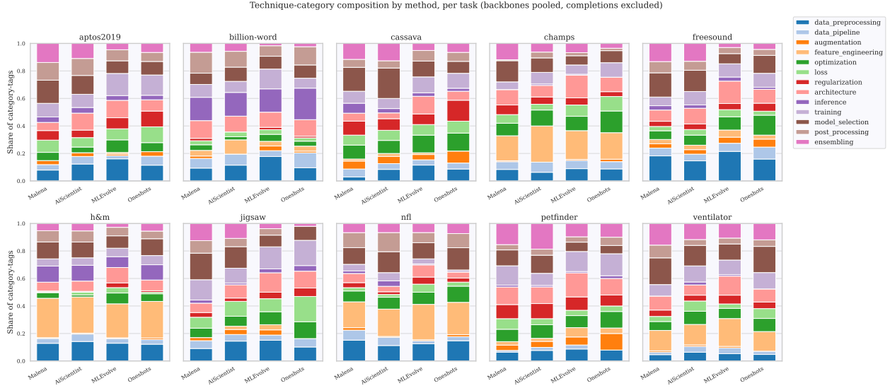
Figure 15 Technique-category composition of each method’s technique repertoire, per task (backbones pooled, completions excluded). The x-axis is method (Malena, AiScientist, MLEvolve, Oneshots); the y-axis is share of category-tags. Bar segments are shares of category-tags (a technique tagged with multiple categories counts toward each), not shares of techniques.
