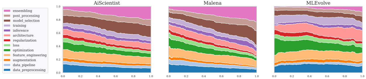
Figure 6 Category composition of techniques used so far, over the course of a run, one column per method. The x-axis is checkpoint fraction through the run ( \in [0, 1] ); the y-axis is the decayed share of technique-category tags at that point (stacked, summing to 1). Each technique contributes to a checkpoint’s composition with exponential decay by recency, giving a balanced view of the solution’s techniques that still favours ones added recently. Per-task and alternate half-life versions are in Appendix E.3.
