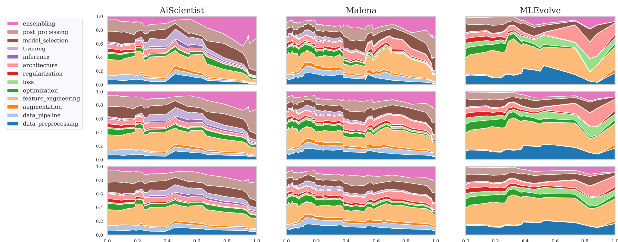
Figure 14 Category-share-decay curve on nfl alone, at half-lives 0.1, 0.15, and 0.2 (rows, top to bottom). As in Figure 6, the x-axis is checkpoint fraction through the run ( \in [0, 1] ) and the y-axis is the decayed share of technique-category tags at that point.
