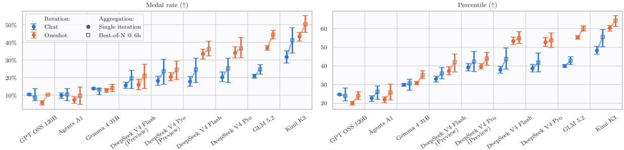
Figure 2 Impact of a coding agent environment. Average percentile and medal rate obtained by Chat and Oneshot iterations under different LLM backbones in the default29 task set. Circles represent single-iteration performance, while squares indicate Best-of-N performance at six-hour budgets.
