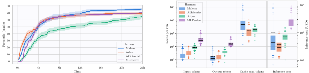
Figure 10 Left: oracle best-so-far vs. wall-clock time at Kimi K3 for Malena, Arbor, AiScientist, and MLEvolve. Right: per-run distribution of cumulative input, output(+reasoning), and modeled cache-read tokens, plus a USD-cost group at Kimi K3 pricing, for Malena, Arbor, AiScientist, and MLEvolve. MLEvolve’s cache group is omitted (always exactly 0, same reason as the GLM 5.2 figure).
