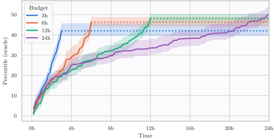
Figure 8 Behaviour of Malena under different time budgets. Average oracle percentile obtained by Malena on the default29 split with a DeepSeek V4 Pro (Preview) backbone model. Trajectories are extracted from the full run by scoring the submissions available at each time. Dotted lines are shown after a timeout target is hit, and maintain the performance achieved.
