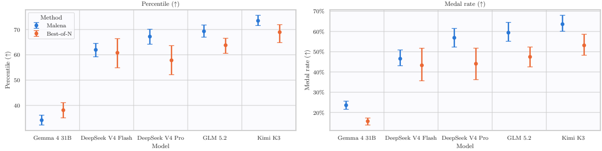
Figure 9 Malena model ablation. Average percentile and medal rate obtained by the Malena iteration and Best-of-N Oneshot iterations at the 24h time budget in the default29 set. Error bars represent 95% CIs across our fixed 29-task set.
