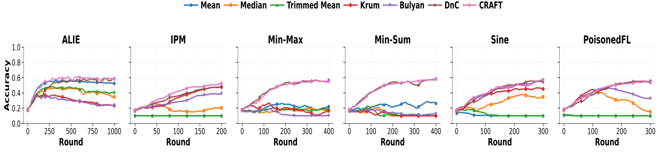
Fig. 7: CIFAR-10 accuracy under model-poisoning attacks.
