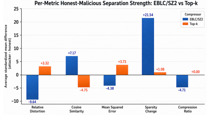
Fig. 3: Per-metric honest-malicious footprint separation for EBLC/SZ2 and Top- K .
