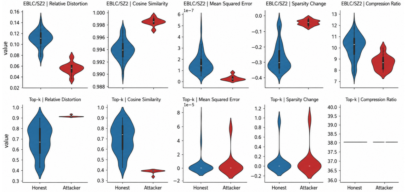
Fig. 13: Per-metric footprint distributions for honest and malicious clients under EBLC/SZ (top row) and Top- K (bottom row). EBLC/SZ exhibits separation across multiple footprint coordinates, whereas Top- K is informative mainly in a narrower subset of metrics.
