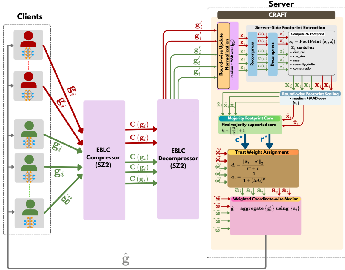
Fig. 1: Overview of CRAFT. The server decompresses client updates, extracts server-side compression footprints, assigns footprint-based trust weights, and aggregates the decompressed updates with a weighted coordinate-wise median.
