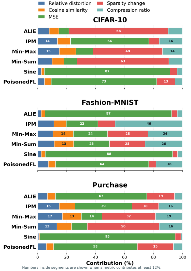
Fig. 6: Contribution of each compression-footprint metric to honest–malicious separation across attacks.
