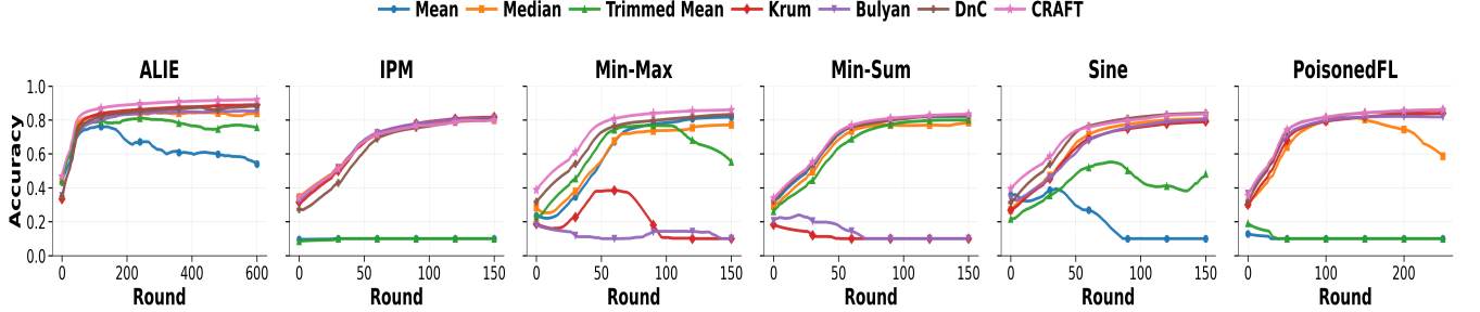
Fig. 8: Fashion-MNIST accuracy under model-poisoning attacks.
