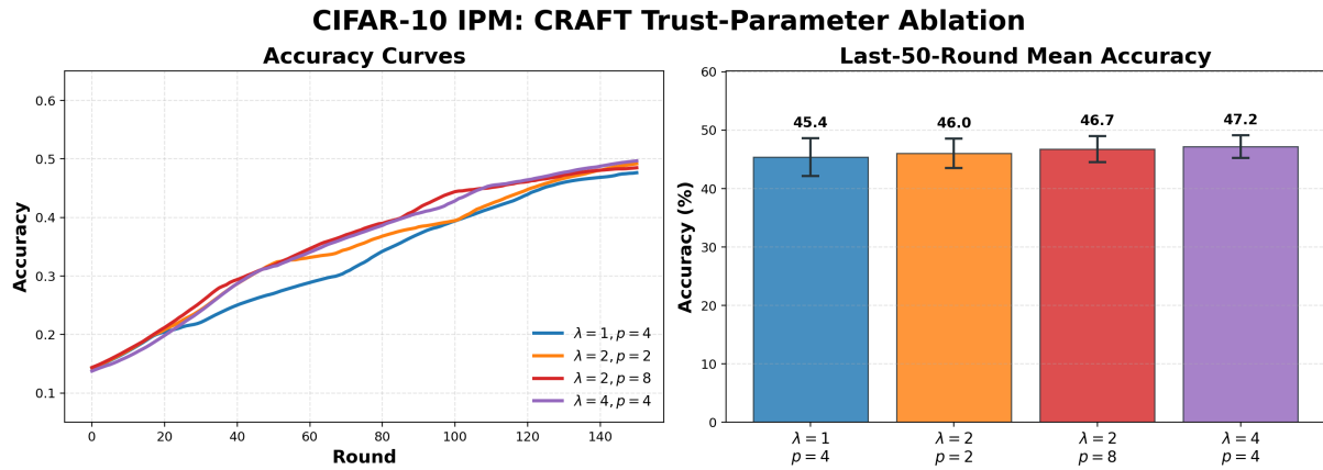
Fig. 16: CRAFT trust-parameter ablation on CIFAR-10 under IPM.
