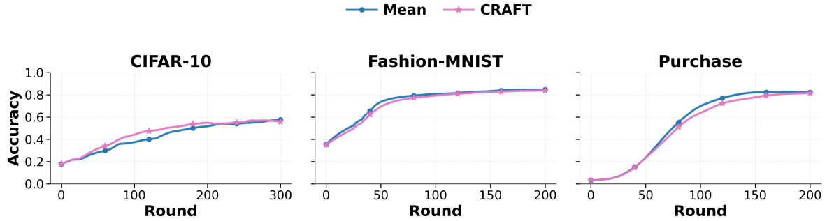
Fig. 15: No-attack baseline accuracy for Mean aggregation and CRAFT on CIFAR-10, Fashion-MNIST, and Purchase. CRAFT closely tracks Mean when all clients are honest.
