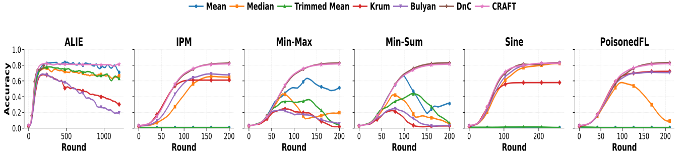
Fig. 9: Purchase accuracy under model-poisoning attacks.
