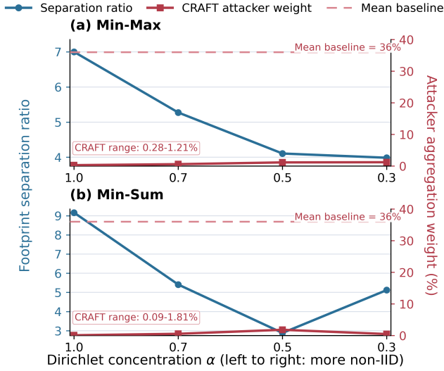
Fig. 10: Effect of Dirichlet label skew on CRAFT for CIFAR-10 under Min-Max and Min-Sum attacks. Lower \alpha indicates stronger non-IIDness. The dashed line shows the 36% attacker weight under mean aggregation.
