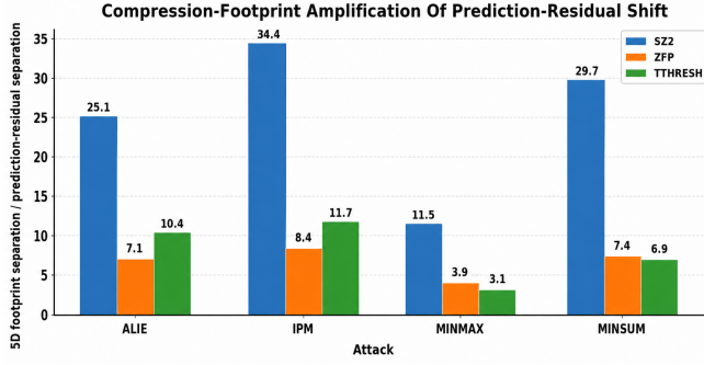
Fig. 4: EBLC-dependent footprint amplification across attacks; SZ2 gives the strongest amplification in this setting.
