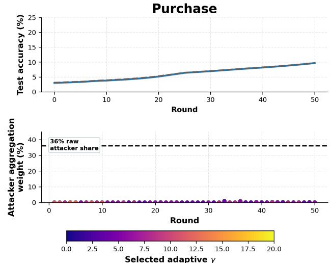
Fig. 14: Purchase under restricted adaptive IPM. CRAFT assigns almost no aggregation weight to attackers.
