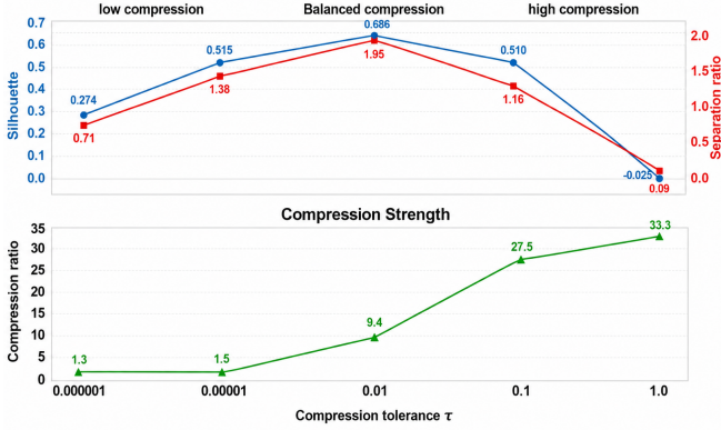
Fig. 5: Effect of SZ2 tolerance on footprint separation and compression strength.
