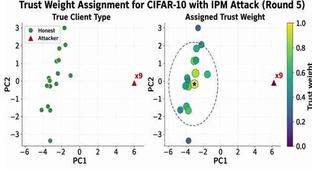
(a) Clear footprint separation.
