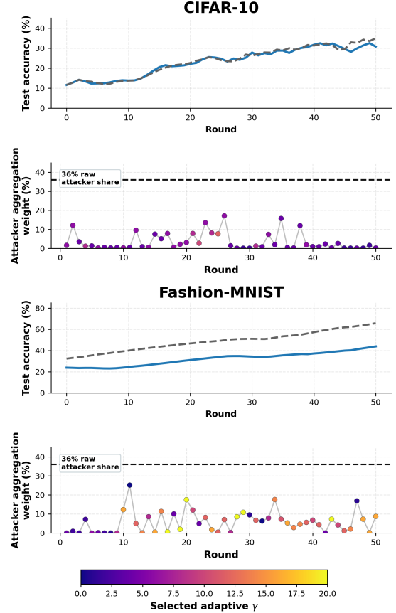
Fig. 11: Restricted adaptive IPM results.
