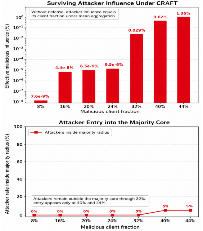
Fig. 12: Effect of malicious client fraction on CRAFT for CIFAR-10 under IPM. Malicious influence remains negligible until attackers begin to enter the majority-supported footprint core.
