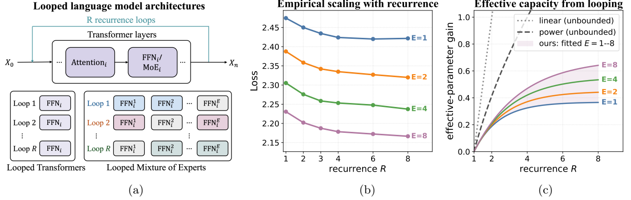
Figure 1 (a) Dense looped transformers reuse the same FFNs, whereas looped MoE models can route tokens to different experts across recurrent passes. (b) At fixed active parameters and training tokens, increasing recurrence yields diminishing returns, with the dense model ( E=1 ) saturating earlier than MoE models ( E>1 ). (c) Our Loop Scaling Laws model a bounded effective-parameter gain conditioned on recurrence R and sparsity (varied by expert count E ), unlike prior linear and power-law mappings that assume unbounded gains.
