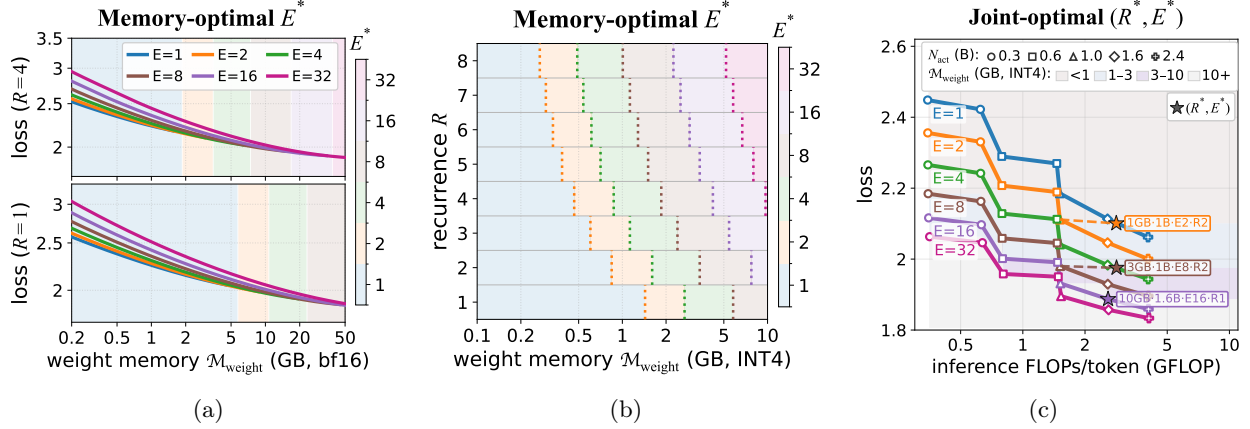
Figure 6 Predicted memory-optimal expert count E^* and joint optimum (N_{\text{act}}^*, E^*, R^*) at \bar{F}_{\text{train}}=5 \times 10^{21} FLOPs. (a) E^* across bf16 weight-memory budgets at R=4 (top) and R=1 (bottom). (b) E^* across INT4 weight memory and recurrence. (c) Predicted joint optimum (N_{\text{act}}^*, E^*, R^*) across INT4 weight memory.
