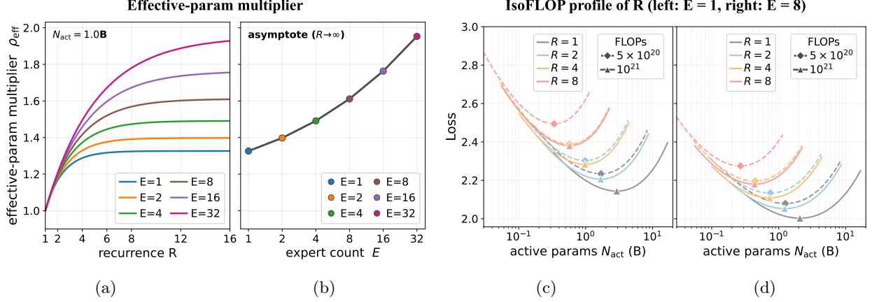
Figure 4 (a,b) Effective-parameter multiplier over recurrence at N_{\text{act}}=1.0\text{B} , and its asymptote over expert count. (c,d) Recurrence IsoFLOP profiles for dense ( E=1 ) and MoE ( E=8 ) models; markers denote minima.
