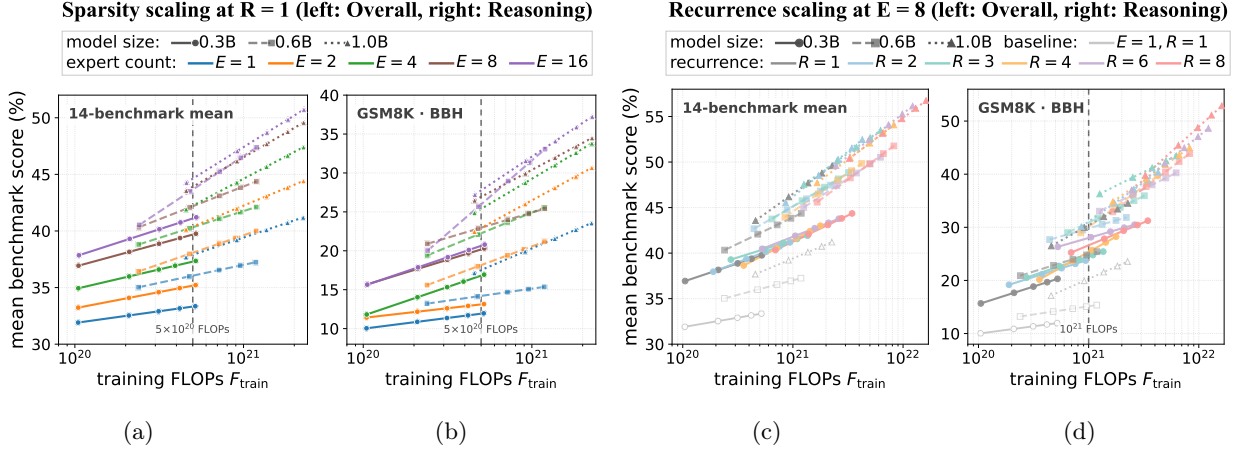
Figure 7 Downstream scaling of sparsity and recurrence. (a,b) Scaling E at R=1 ; (c,d) Scaling R at E=8 , with the dense baseline E=1, R=1 . (a,c) report Overall performance, and (b,d) report Reasoning performance; dashed lines mark compute-matched comparisons.
