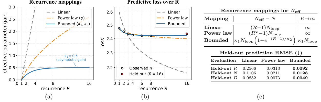
Figure 2 (a) Illustration of effective-parameter gain under linear, power-law, bounded recurrence mappings. (b) Predictive loss by different recurrence mappings: each mapping is fitted on R \leq 8 and applied to predict the held-out- R up to R = 16 . (c) Formula on recurrence mappings and their effective-parameter gains (top) and their evaluation on held-out recurrence R , model N , and data D with RMSE scores (bottom).
