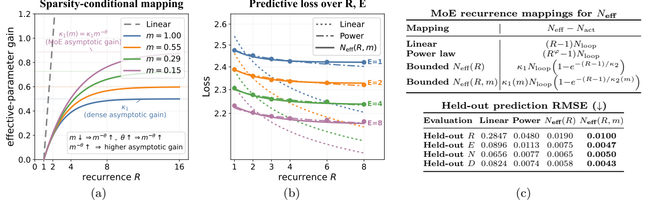
Figure 3 (a) Illustration of effective-parameter gain with sparsity-conditional recurrence mapping. (b) Predictive loss under different MoE recurrence mappings fitted on runs with R \leq 8 ; markers denote observations used for fitting. (c) Formula on MoE recurrence mappings and their effective-parameter gains (top), and their evaluation on held-out recurrence R , expert count E , model size N , and data D with RMSE scores (bottom).
