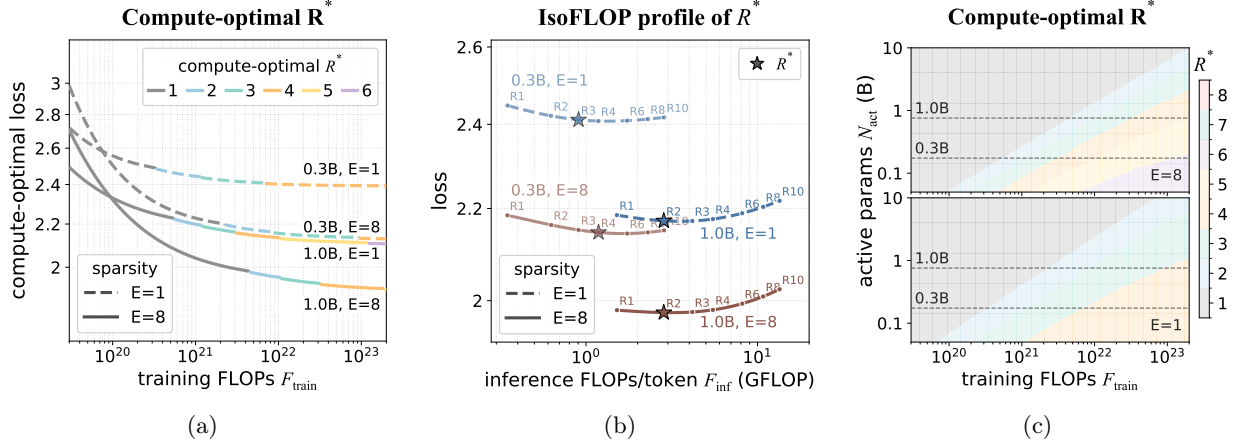
Figure 5 Predicted compute-optimal recurrence R^* of dense ( E=1 ) and MoE ( E=8 ) models. (a) Recurrence with compute-optimal loss across training-compute budgets. (b) IsoFLOP profiles over recurrence at \bar{F}_{\text{train}}=5 \times 10^{21} FLOPs; stars mark R^* . (c) R^* across compute and active model size for E=8 (top) and E=1 (bottom).
