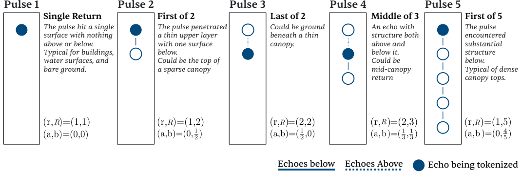
Figure 12: LiDAR return encoding. The pair (a, b) describes the relative position of each observation within its pulse’s return sequence. Normalization by the per-pulse return count R makes the representation independent of the sensor-specific maximum number of returns while preserving the original (r, R) attributes.
