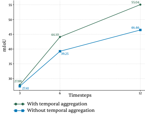
Figure 8: Temporal aggregation ablation on PASTIS as the number of input timesteps increases.
