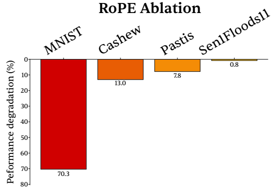
Figure 9: Relative degradation when spatial RoPE is removed, computed as 100(\text{RoPE} - \text{No RoPE})/\text{RoPE} .
