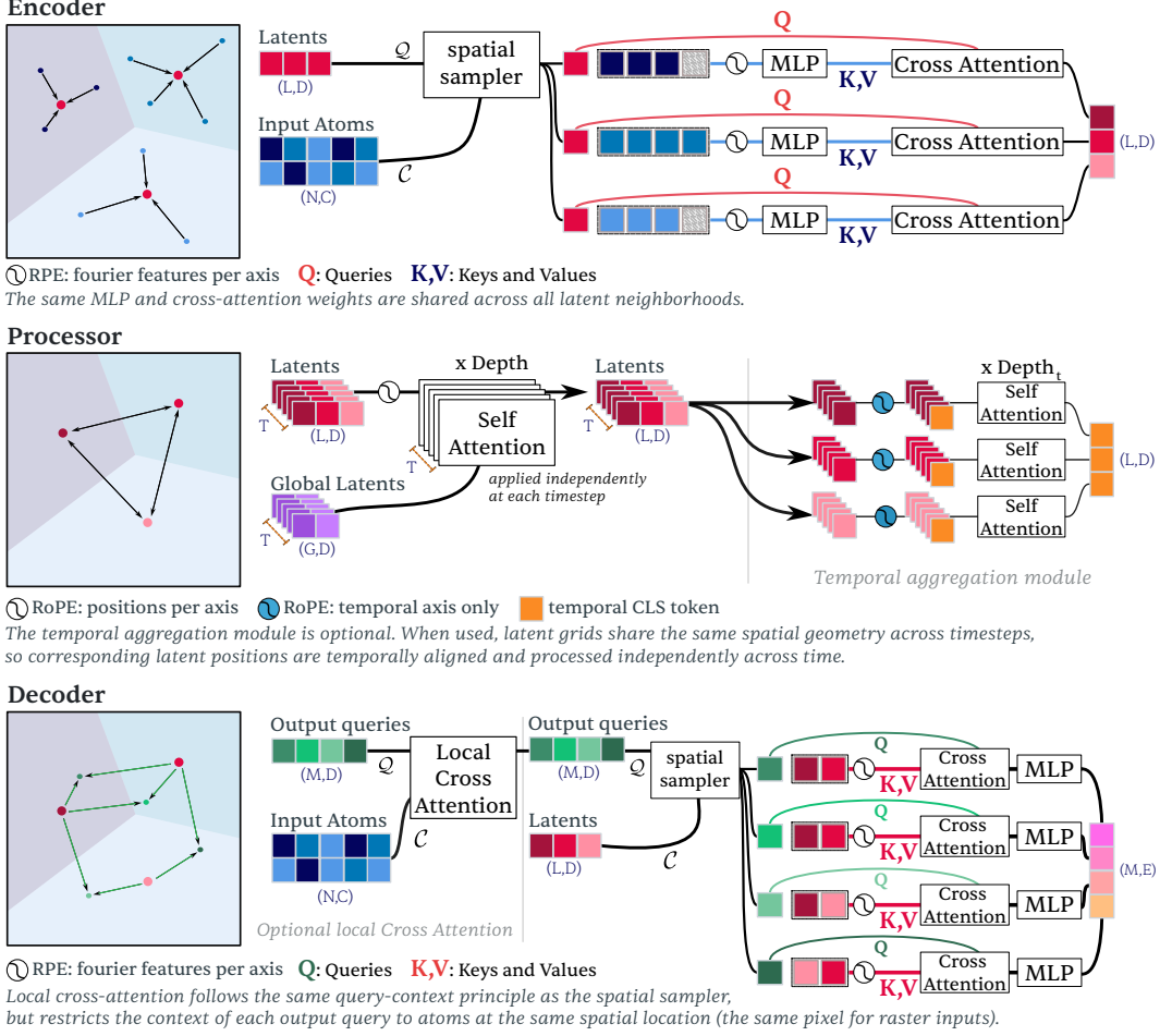
Figure 7: Detailed Atomizer-IO architecture. The encoder aggregates local neighborhoods of input atoms into spatial latents through the spatial sampler; the processor applies latent self-attention with optional temporal aggregation; and the decoder maps local latent neighborhoods to spatial output queries, optionally conditioning first on raw observations at the target location. Relative positional information is introduced locally, and MLP and attention weights are shared across spatial neighborhoods.
