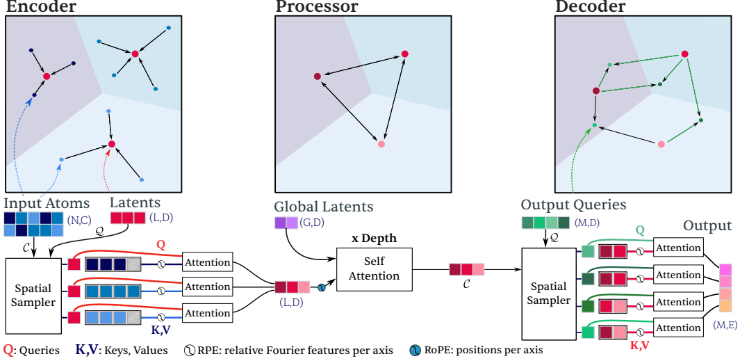
Figure 2: The Atomizer-IO architecture. Atoms are locally aggregated into a compact spatial representation, processed globally in latent space, and decoded through spatial output queries. The same local context-to-query operation is used for encoding and decoding, with spatial relationships defined in physical coordinates rather than by a fixed input grid.
