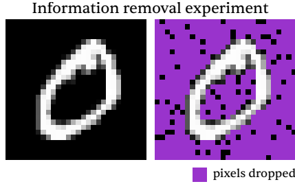
Figure 13: MNIST sparsification protocol. Models are trained on complete images. At evaluation, pixels with value v \leq 0.5 are progressively removed, while pixels with value v > 0.5 are always retained.
