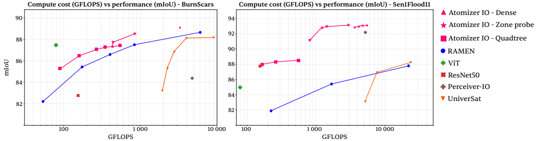
Figure 6: Compute cost (GFLOPS) versus segmentation performance (mIoU). Dense, Zone-probe, and Quadtree decoding vary inference cost through different output query strategies, using the same Atomizer-IO checkpoint without retraining.
