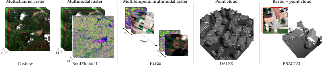
Figure 1: Sensing configurations considered in this work. All are processed through the same atomic interface, without rasterization, resampling, or modality-specific branches.
