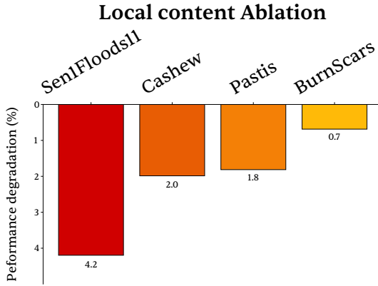
Figure 10: Relative degradation when local observation conditioning is removed, computed as 100(\text{Full} - \text{No Local})/\text{Full} .
