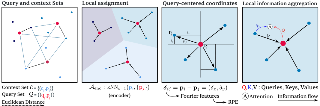
Figure 4: Spatial sampler. From left to right: query and context sets; construction of a local receptive field from spatial proximity, illustrated by the encoder’s nearest-latent assignment and resulting Voronoi partition; query-centered relative coordinates; local cross-attention.
