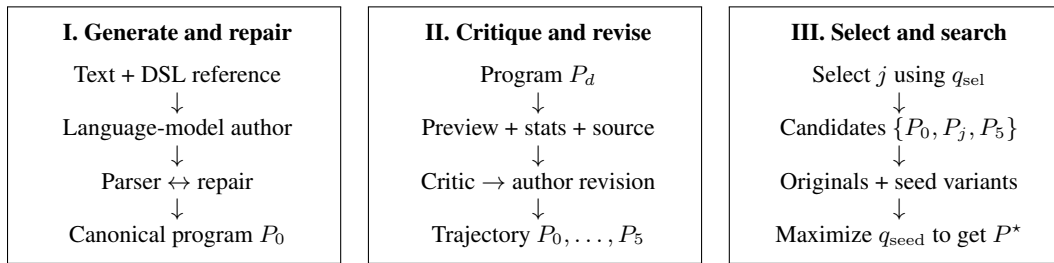
Figure 7: The three-stage pipeline in Figure 3, summarized algorithmically. I. Generation proposes a program and repairs parser errors. II. Critique and refinement revises it using a quick render, material statistics, and source code where configured. III. Selection and seed search scores the trajectory and explores noise realizations of up to three candidate programs while fixing each candidate’s remaining source. The loop uses a lightweight preview renderer and requires no path tracer.
